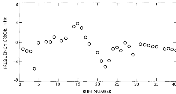
Fig. 11. Tropospheric frequency error for a single raypath
