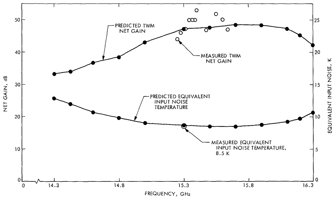
Fig. 5. TWM performance
