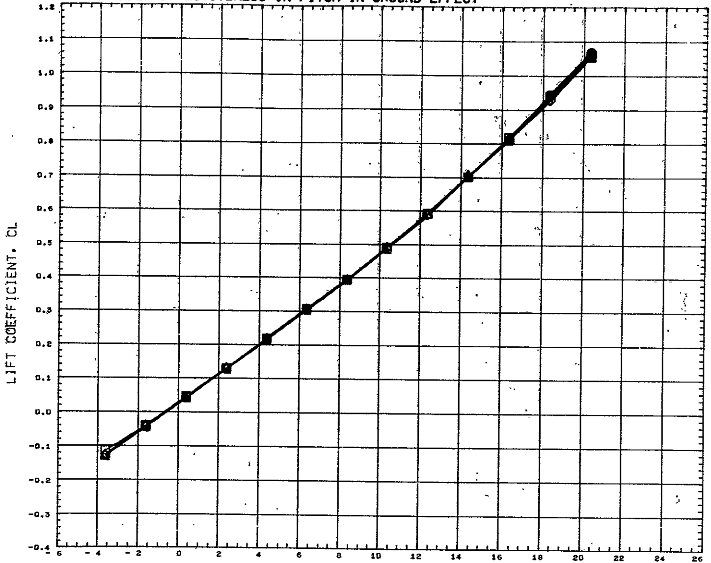
FIG. 6 RUDDER EFFECTIVENESS IN PITCH IN GROUND EFFECT
