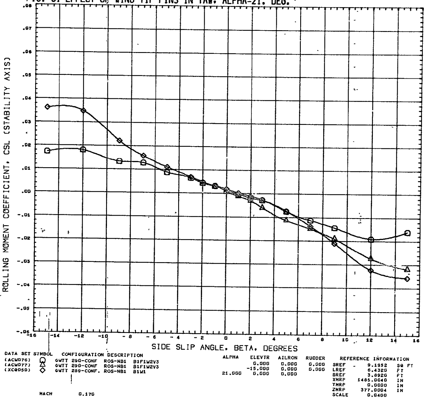
FIG. 31 EFFECT OF WING TIP FINS IN YAW. ALPHA=21. DEG.
