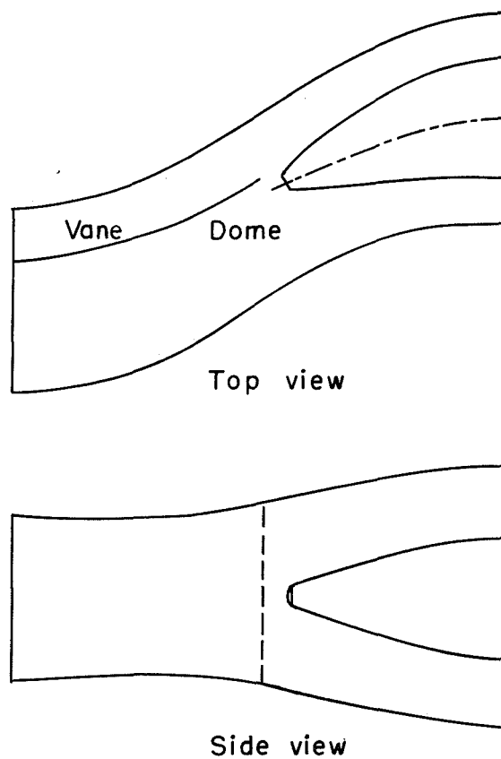
(b) Geometric duct characteristics.
