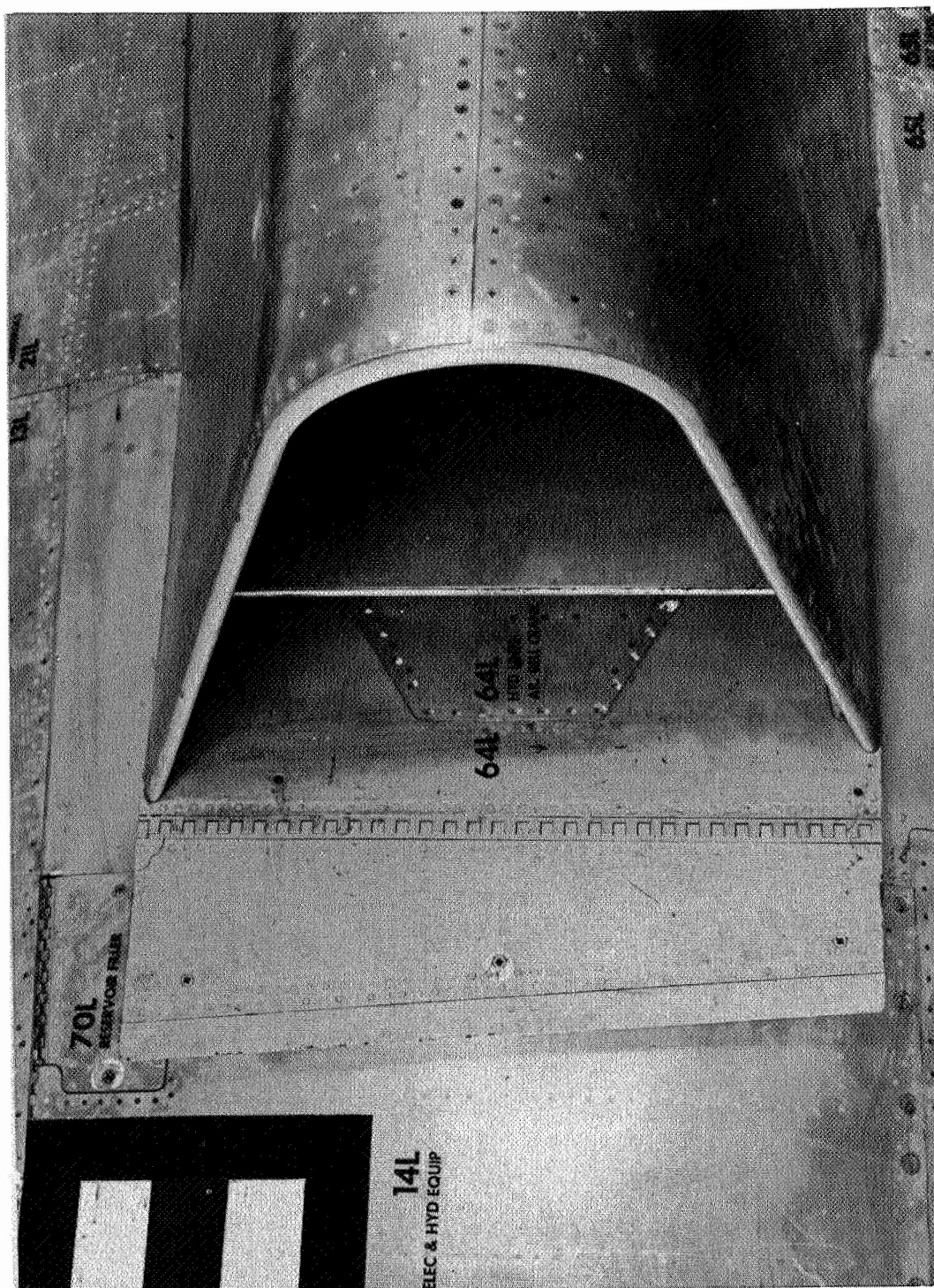
Figure 5.- Photograph showing left inlet of airplane B. E-2459
