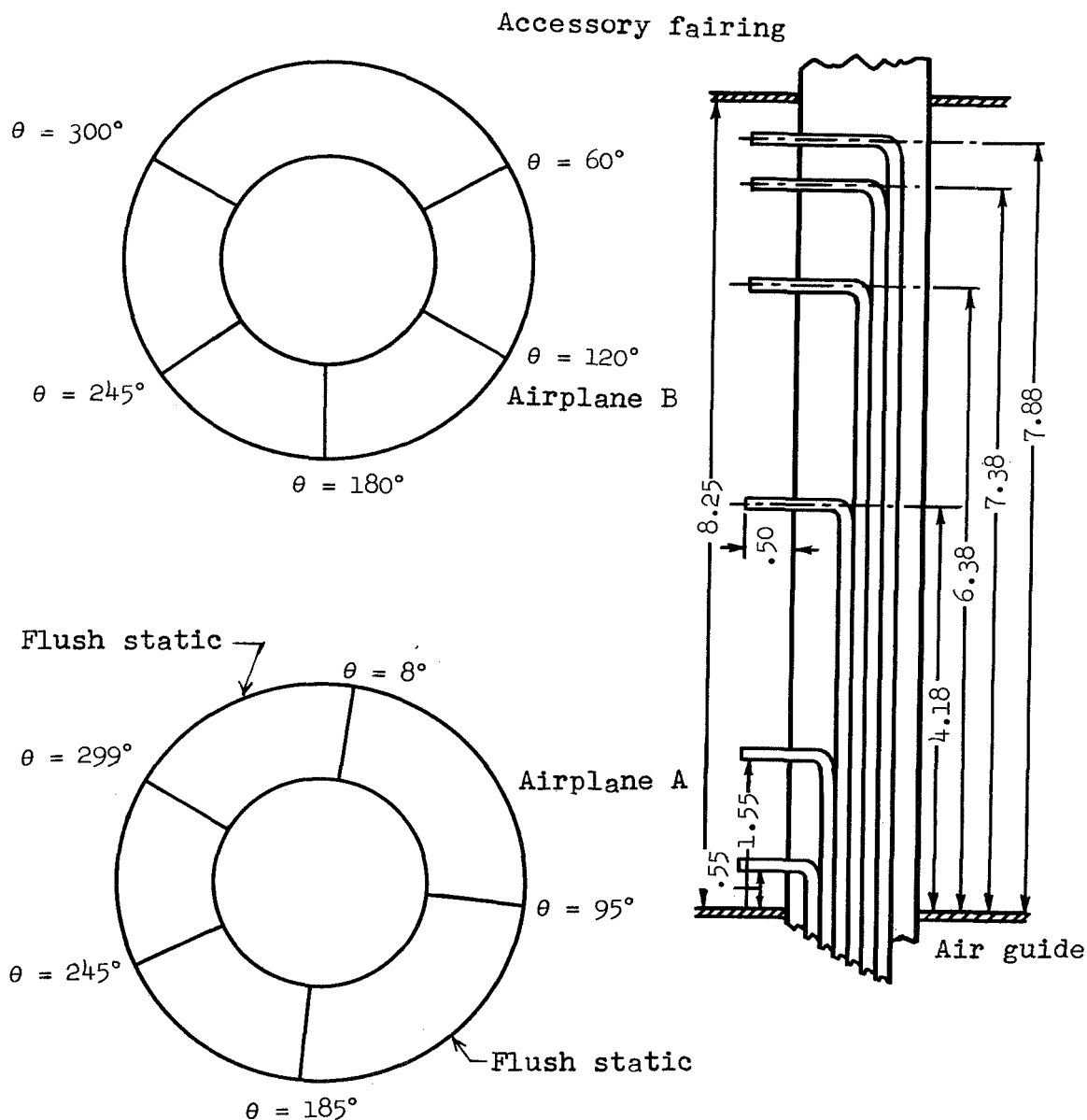
(a) Rake arrangement of compressor face looking aft.
