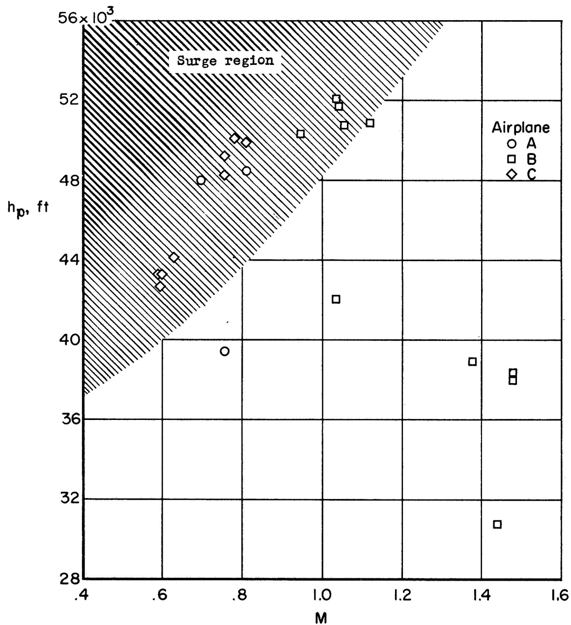
Figure 17.- Pressure altitude and Mach number at incidence of surge for airplanes A, B, and C.
