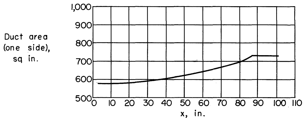
(a) Longitudinal variation of duct cross-sectional area.
