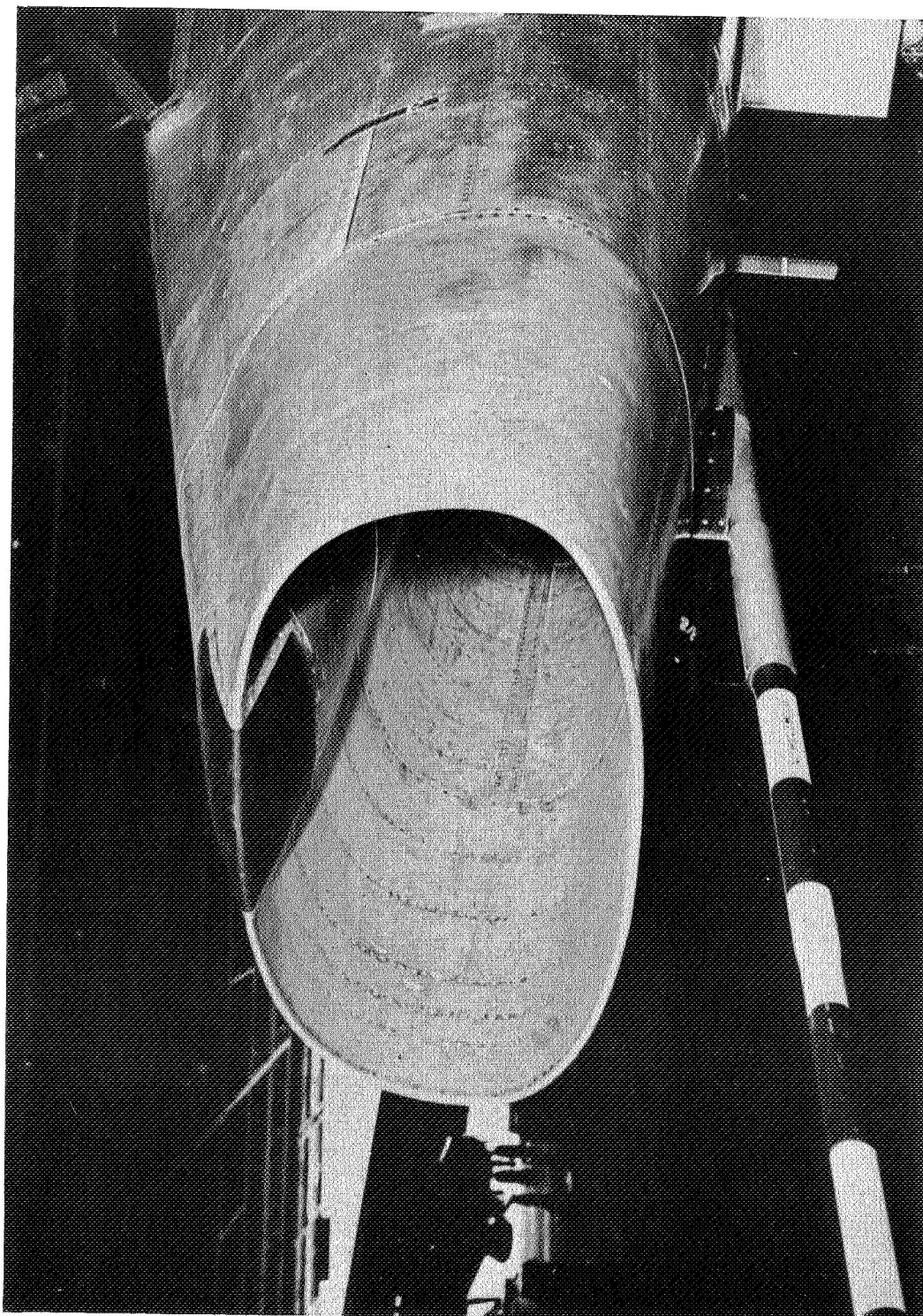
Figure 2.- Photograph showing inlet of airplane A. E-2994
