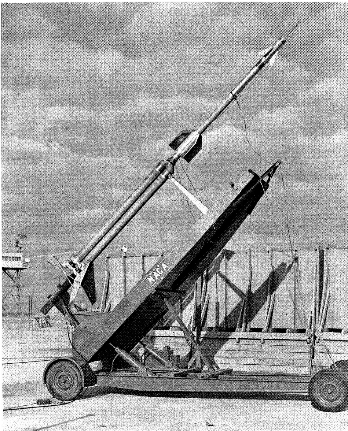
Figure 4.- Photograph of model and booster prior to launching.
