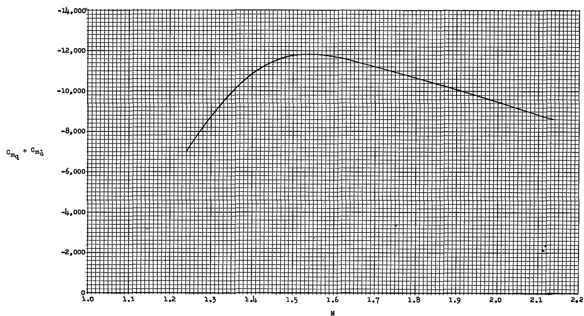
Figure 9.- Variation of the aerodynamic damping-in-pitch derivative C_{mq} + C_{m\delta} with Mach number.
