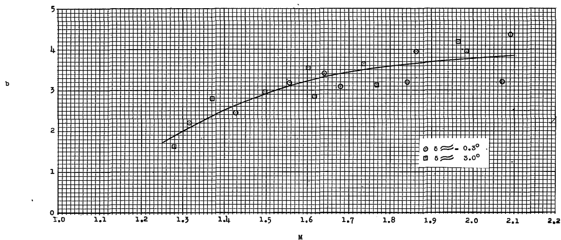
Figure 8.- Variation of the exponential damping constant b with Mach number
