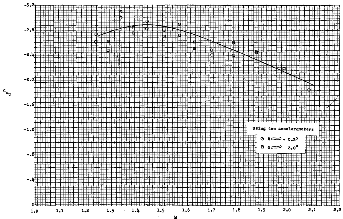
Figure 11.- Variation of the static stability derivative C_{m_\alpha} with Mach number.
