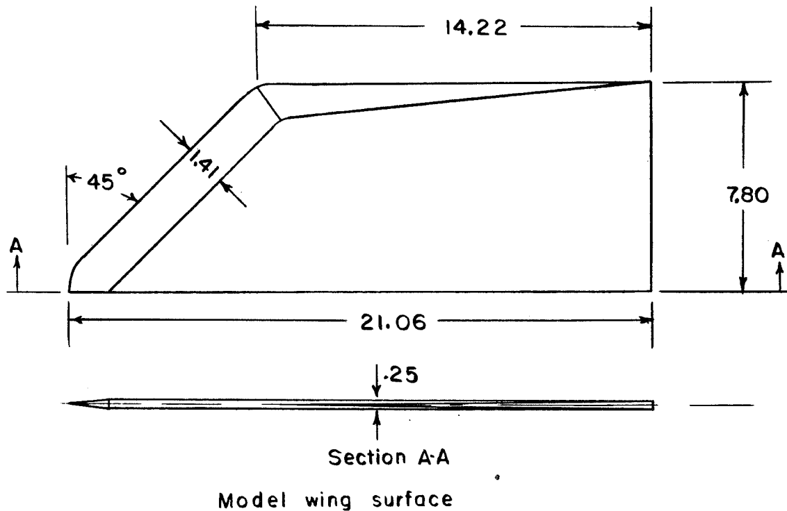
Figure 2.- Sketch of control surface and wing surface for model tested. All dimensions are in inches.
