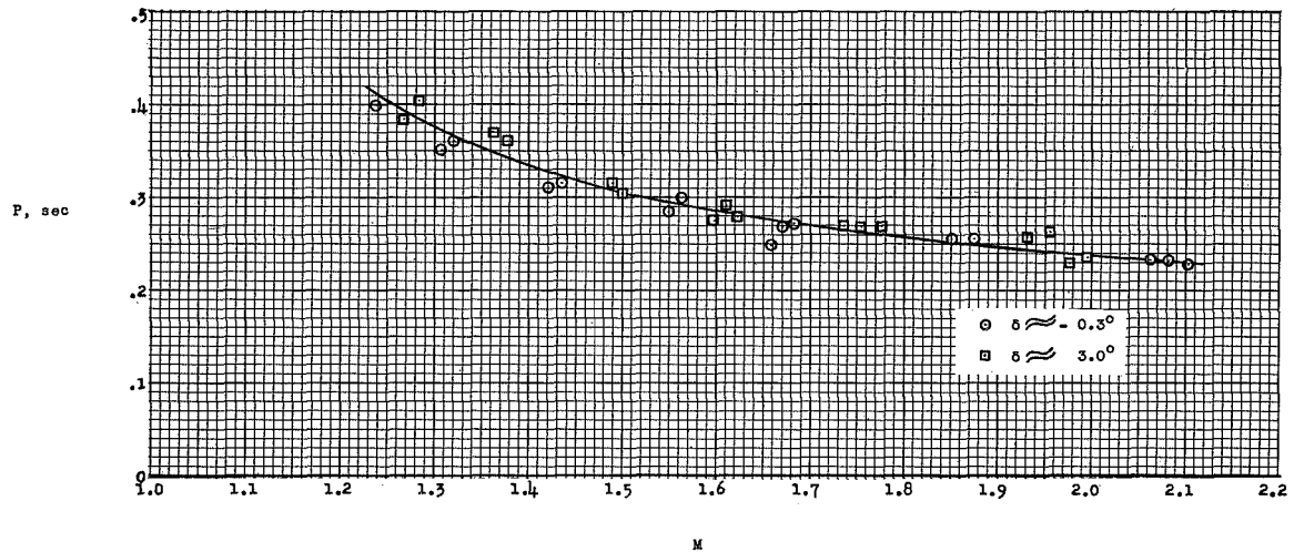
Figure 10.- Variation of period of oscillation with Mach number.
