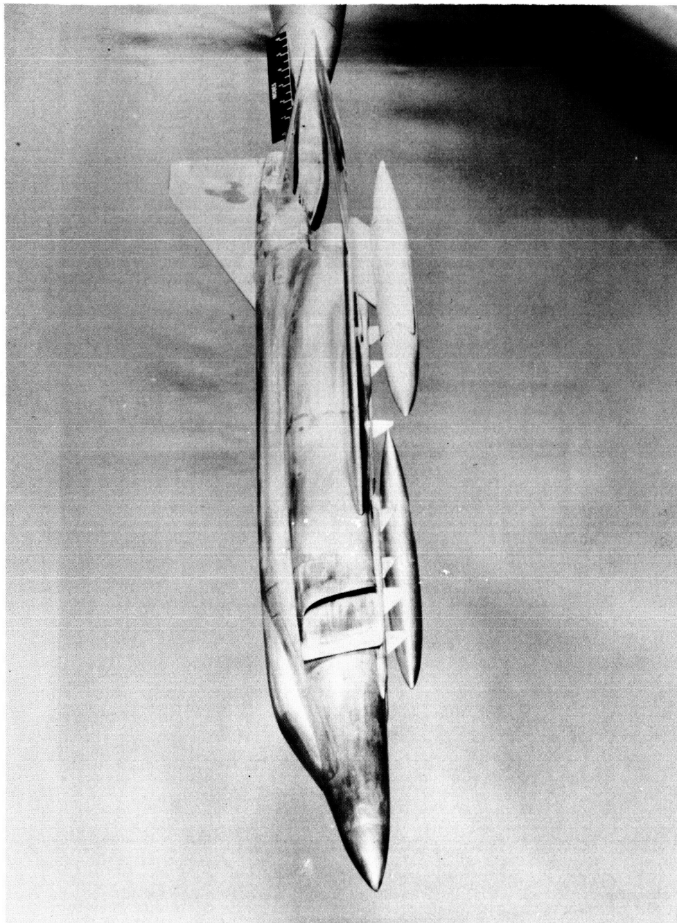
(f) Three-quarter front view with wing tanks. L-57-470
