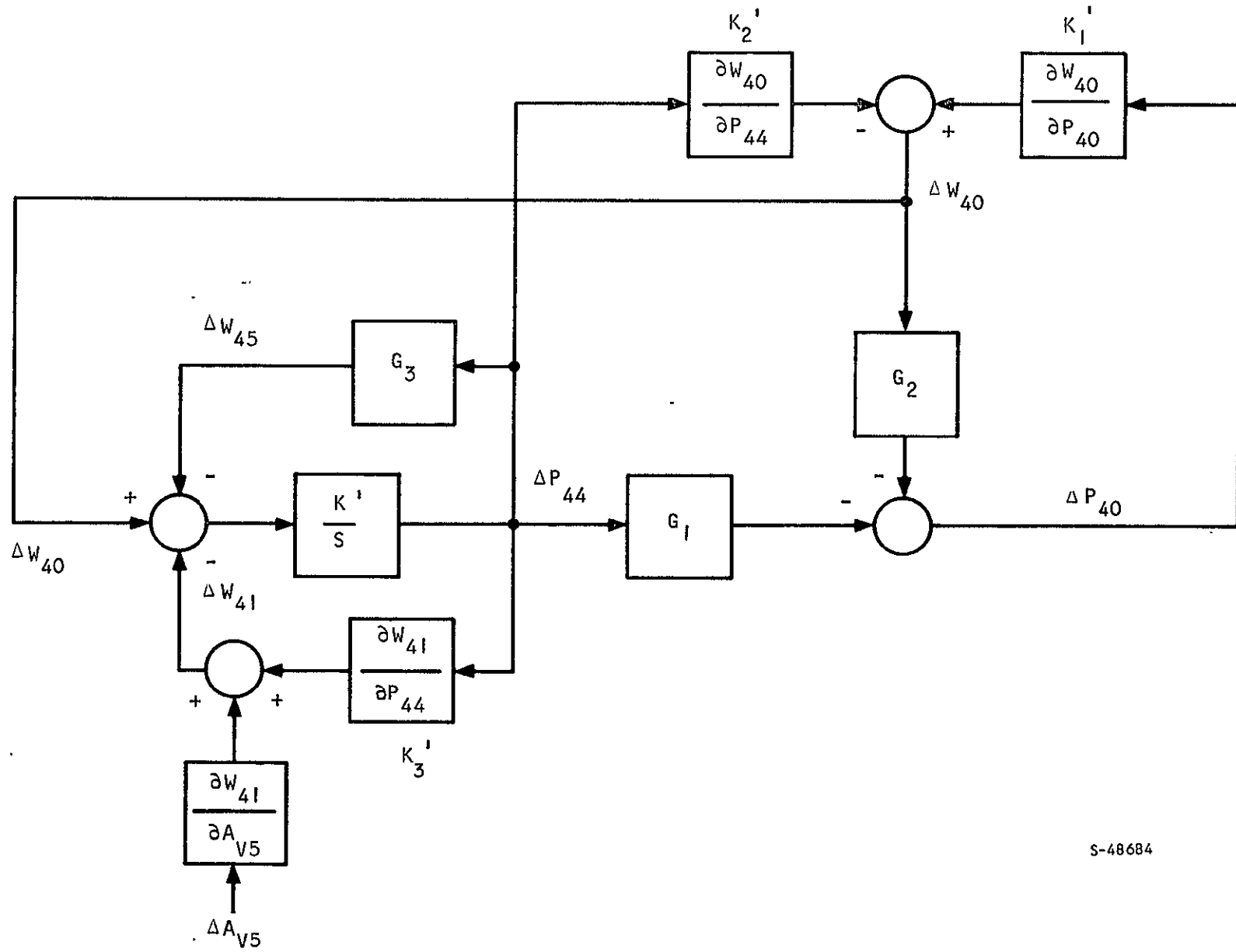
Figure 5.2-8. Turbopump with Simplified System Block Diagram
