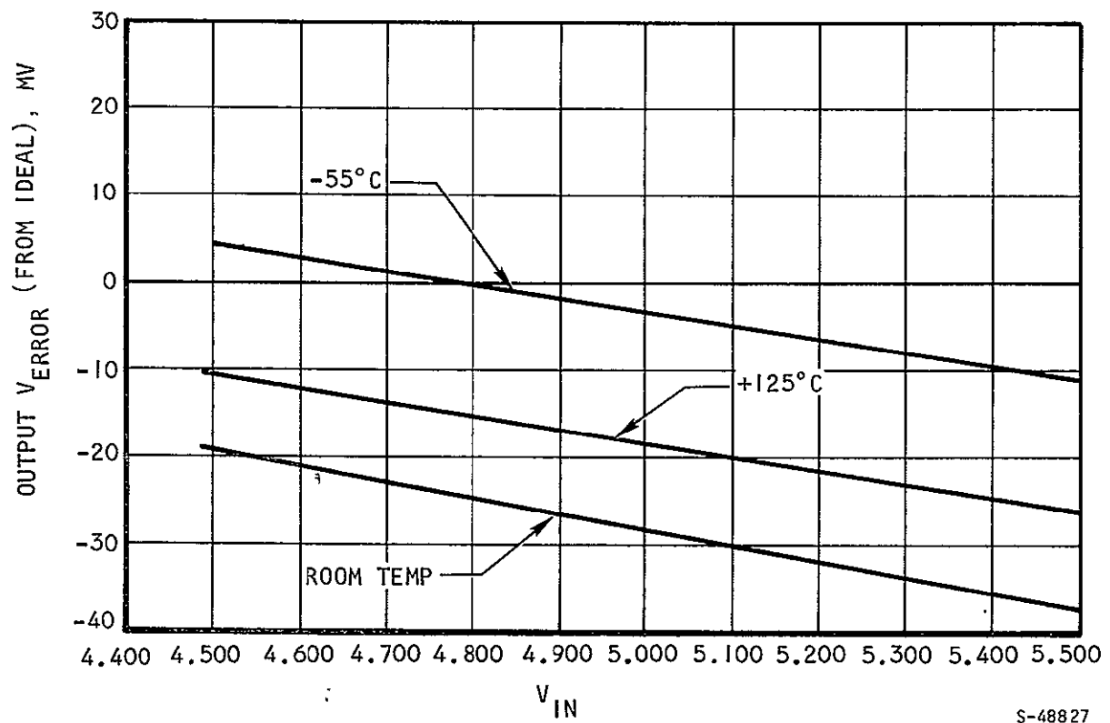
Figure 6.4-11. Dump Valve Driver Temperature Test of Scaling Accuracy
