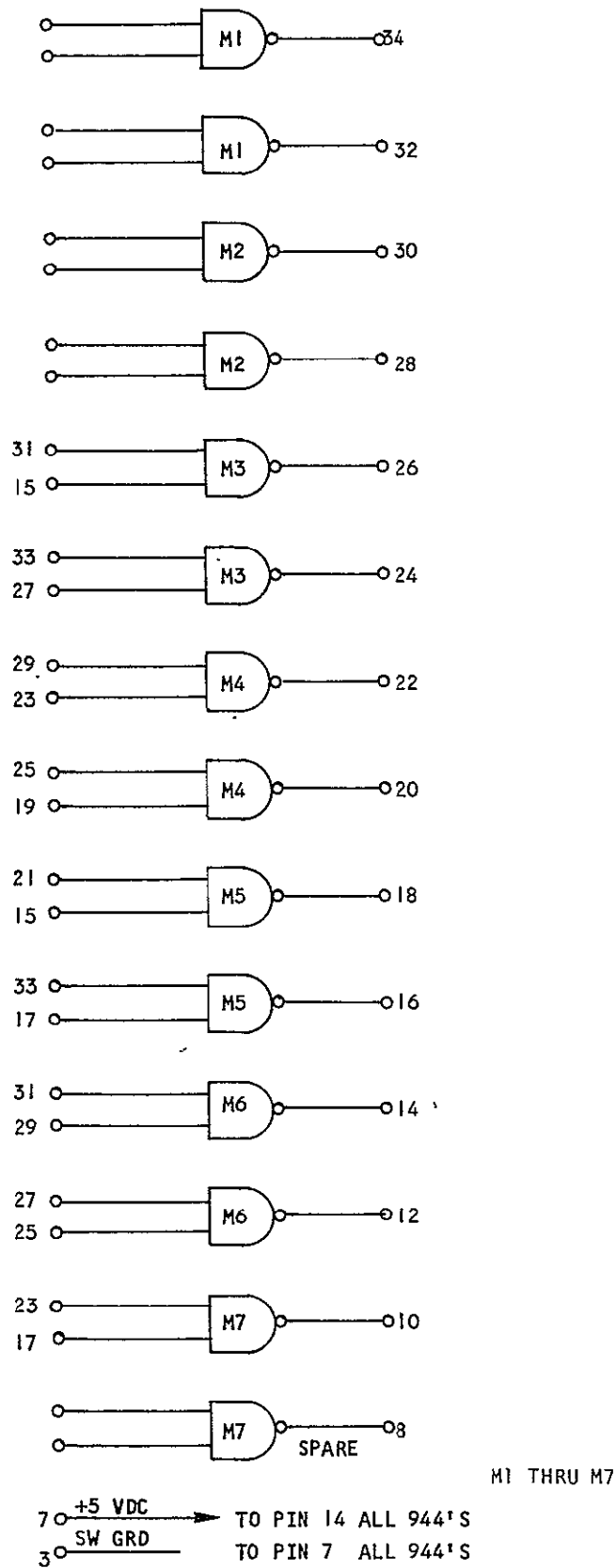
Figure L-14. Decoding Schematic
