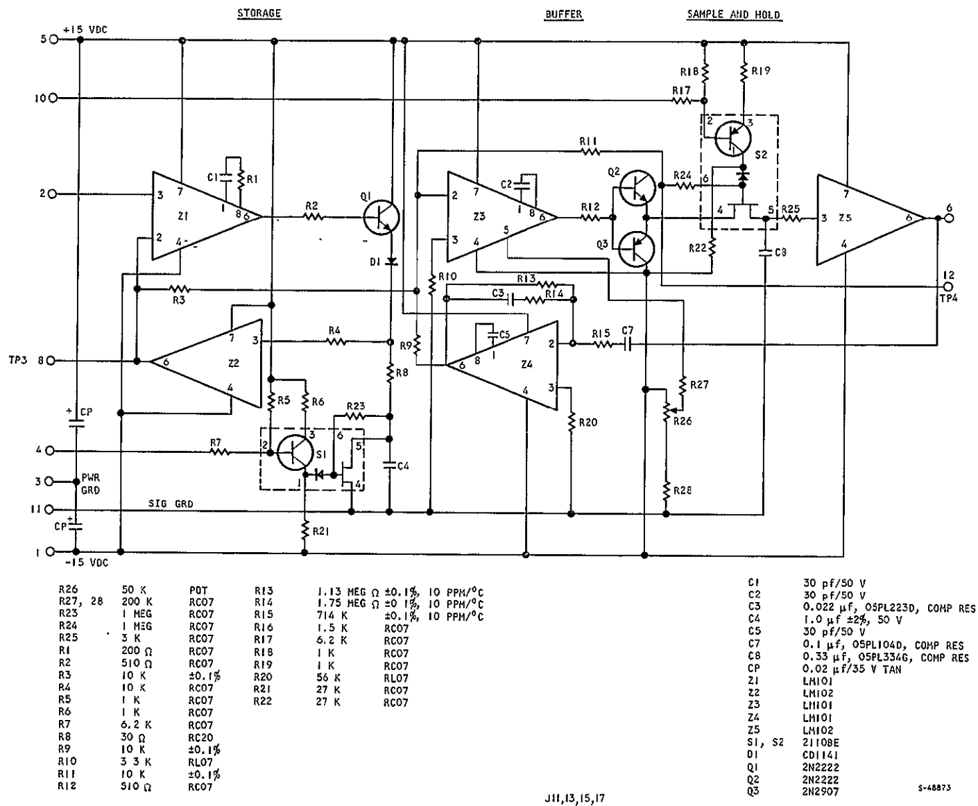
Figure L-9. Storage, Buffer, Sample and Hold Filter Circuits
