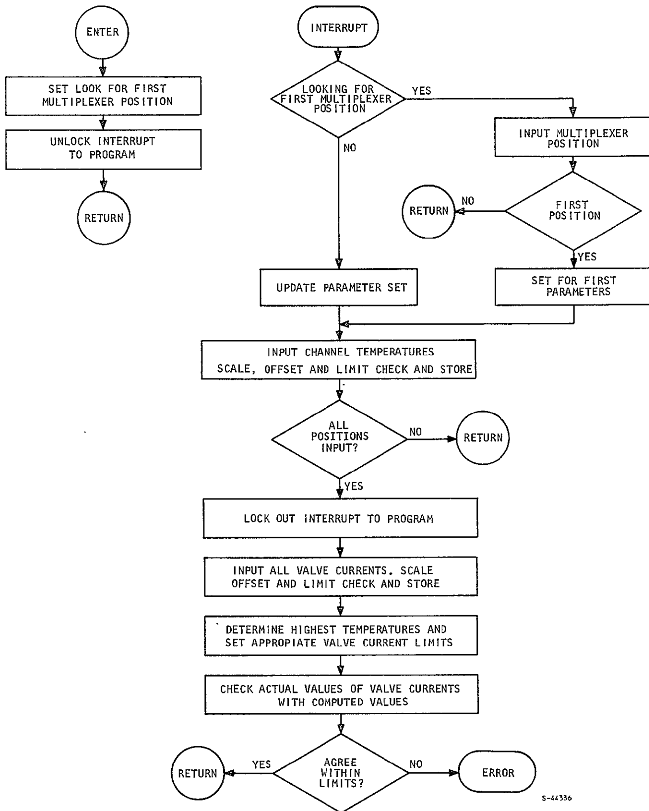
Figure 6.1-9. Temperature Control Monitoring
