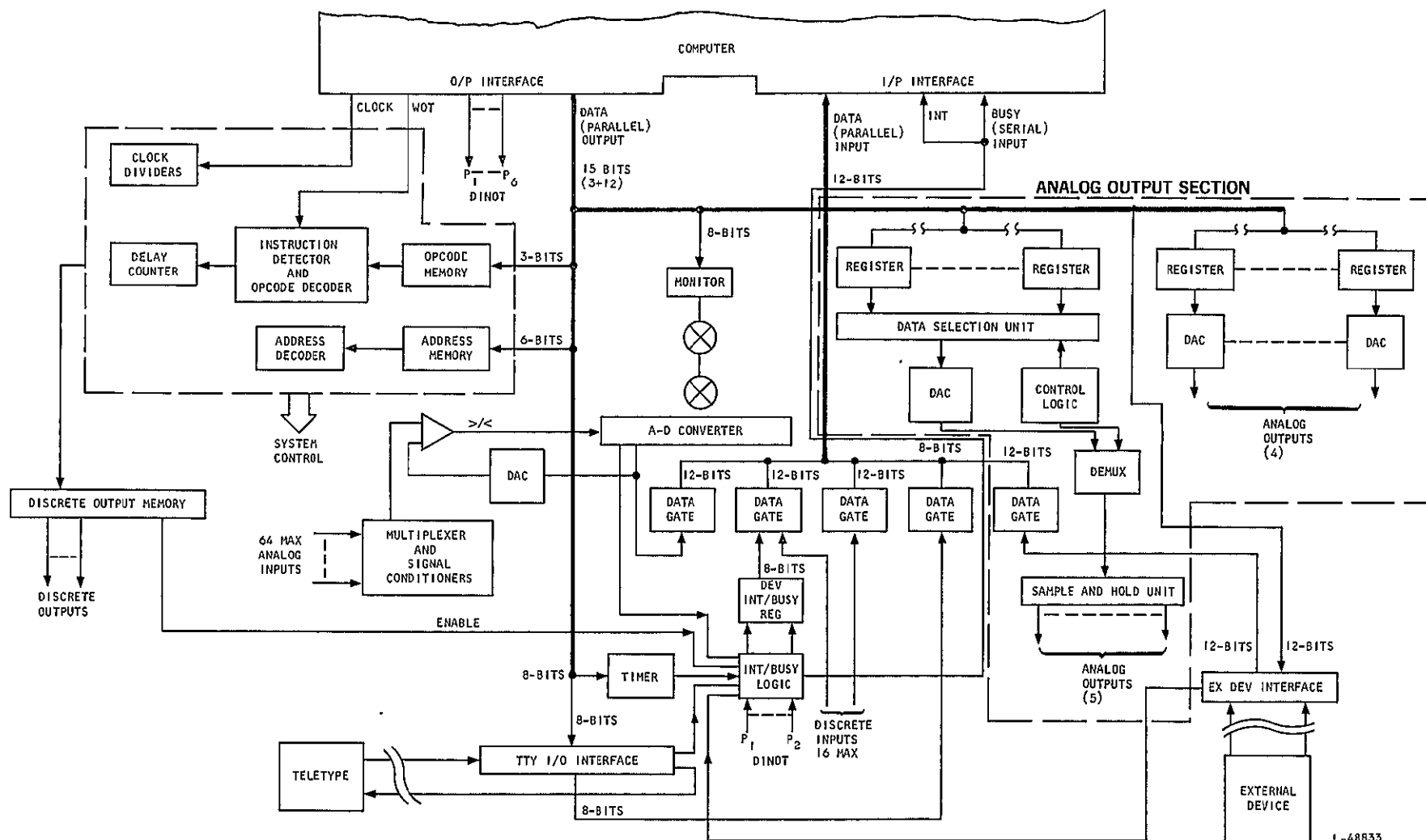
Figure 6.3-2. Present Design CIU-Data Flow Diagram
