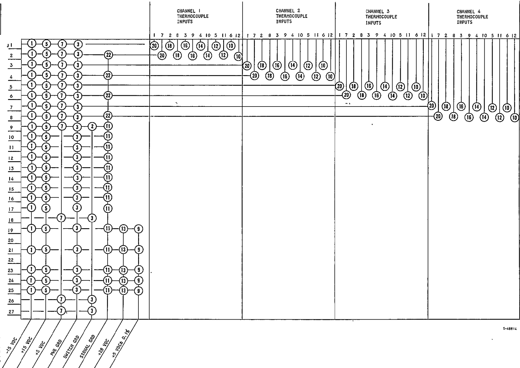
Figure L-3. Breadboard Interconnections
