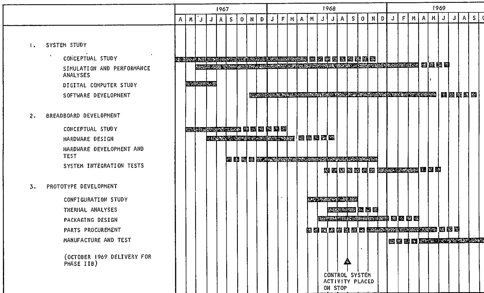
Figure 3.4-1. Control System Development Plan
