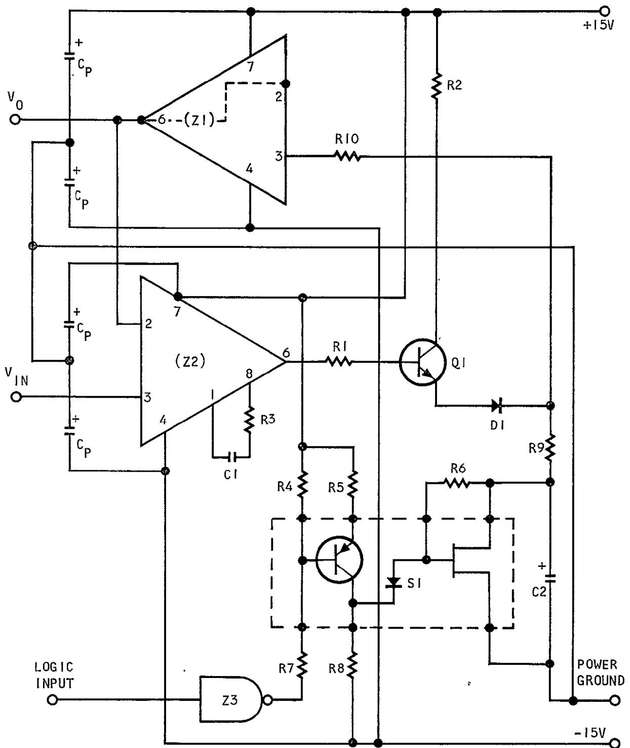
Figure 6.4-2. Storage Circuit
