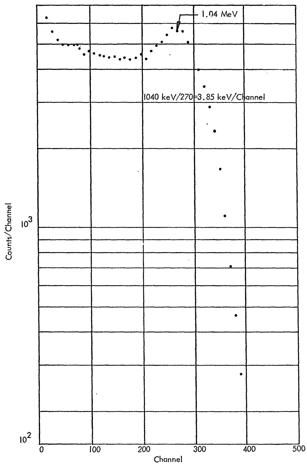
Figure 5 - COMPTON SPECTRUM OF ^{60}\text{Co}
