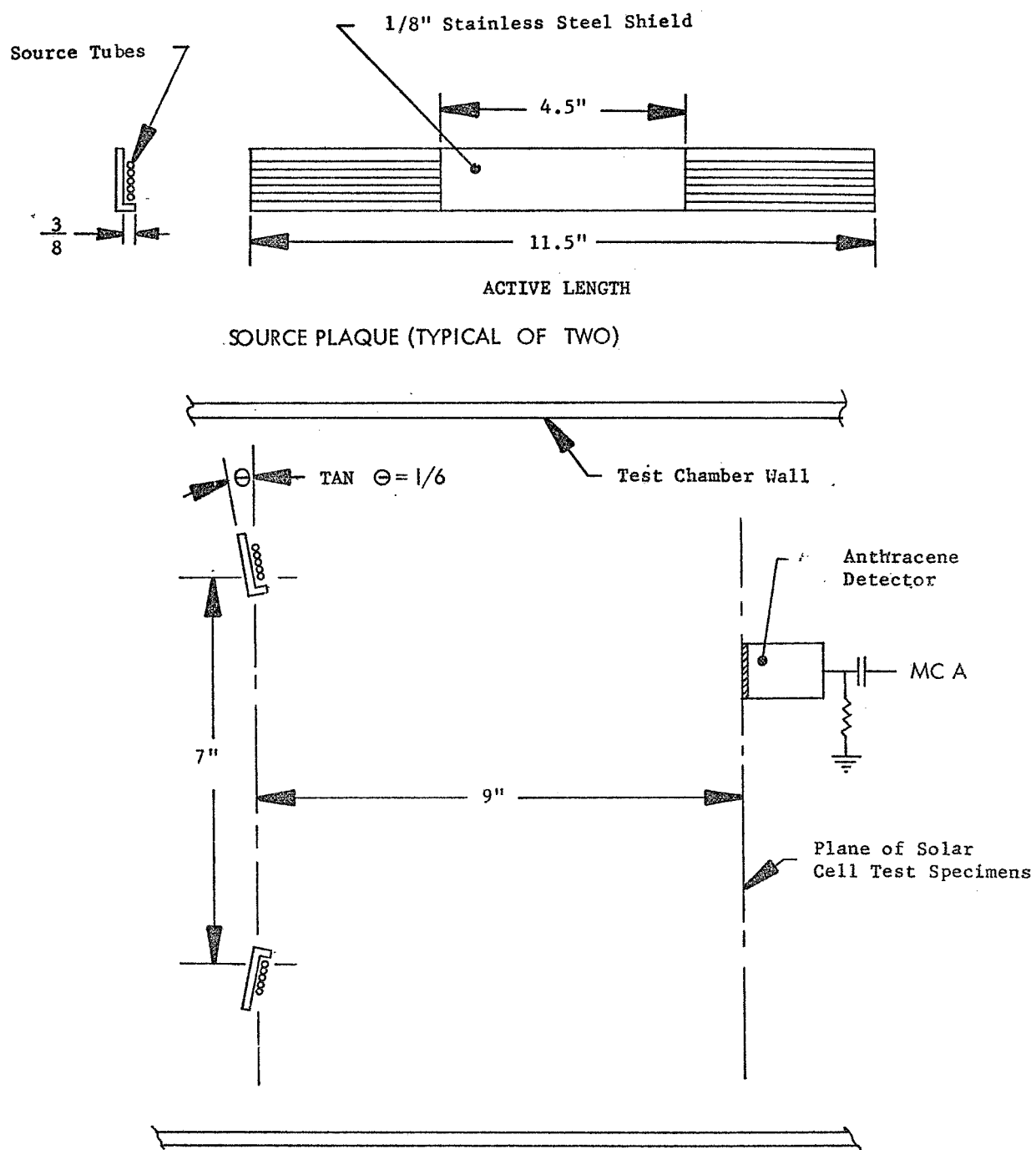
FIGURE 6 - SOURCE TEST AND MAPPING CONFIGURATION
