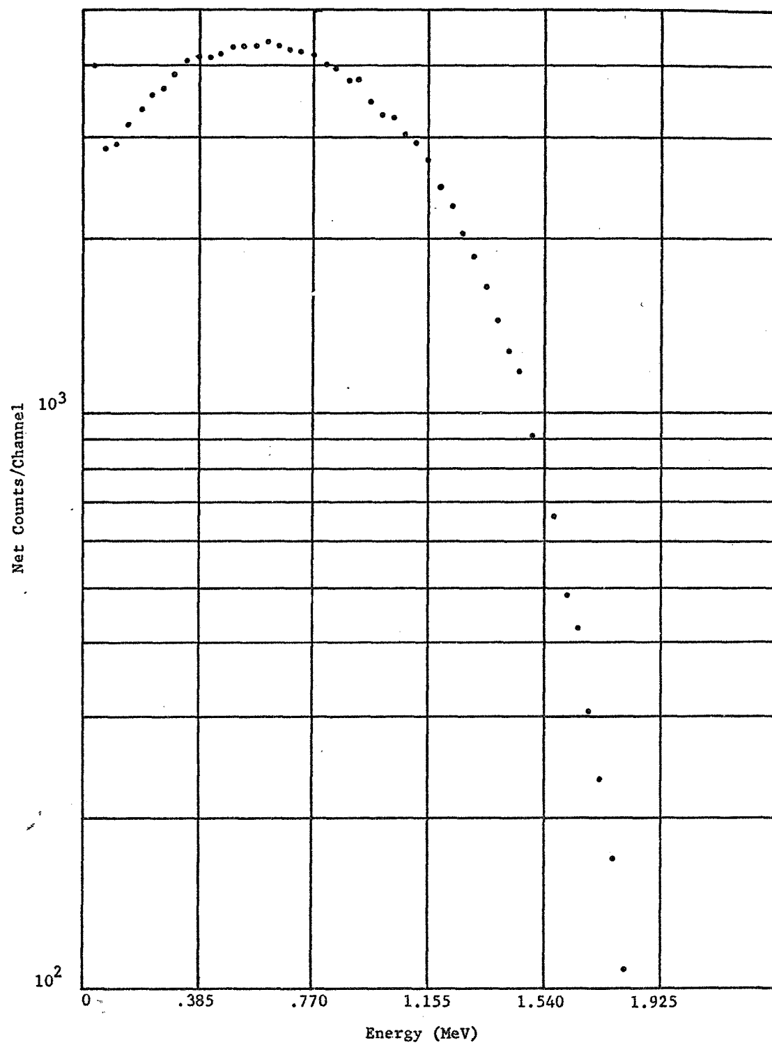
FIGURE 7 - ^{90}\text{Sr} - ^{90}\text{Y} SPECTRUM
