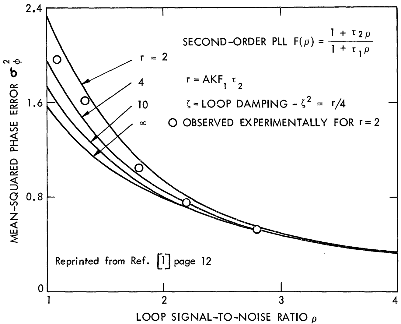
Fig. 7. Variance of the phase error vs loop signal-to-noise ratio for various values of r , for \rho > 3 db, \alpha \approx \rho .
