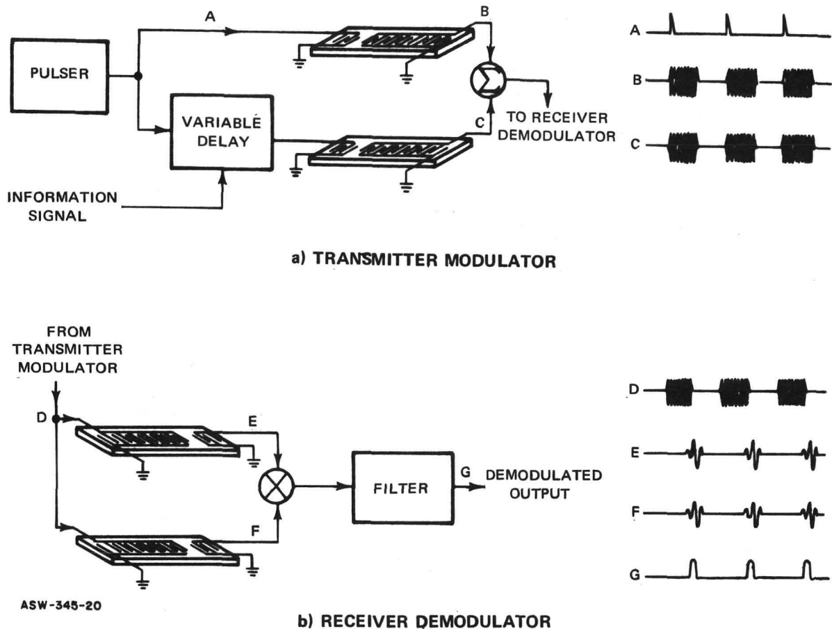
Figure 3-11. Basic Concept of a Code Multiplex Transceiver
