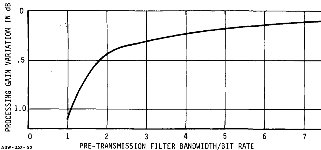
Figure 2-5. Processing Gain Loss Due to Pre-Transmission Filter
