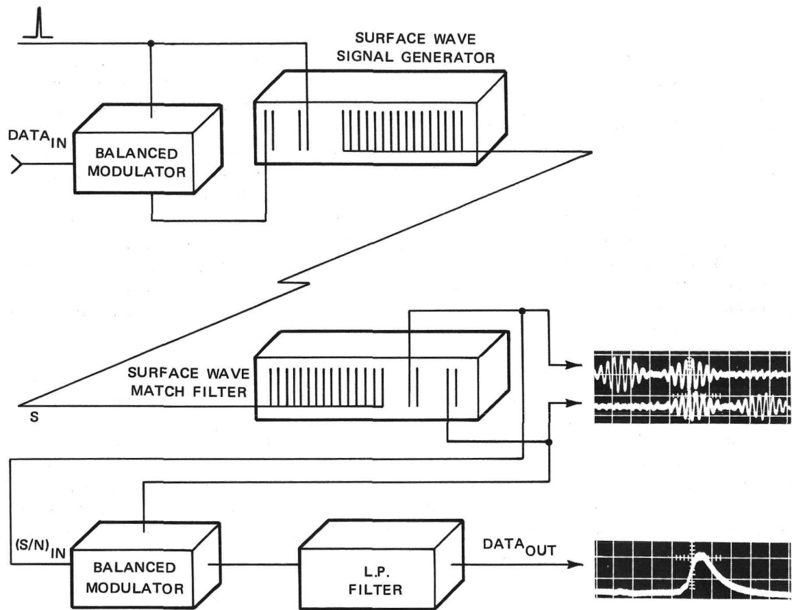
Figure 4-11. Double Pulse Mode PSK Technique
