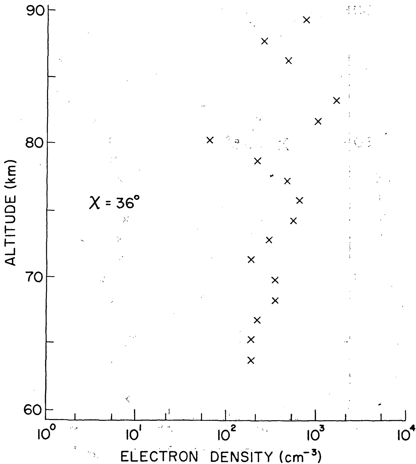
Figure 5.11 Electron-density profile. Date: May 7, 1971, Time: 9:27-9:52 CST.
