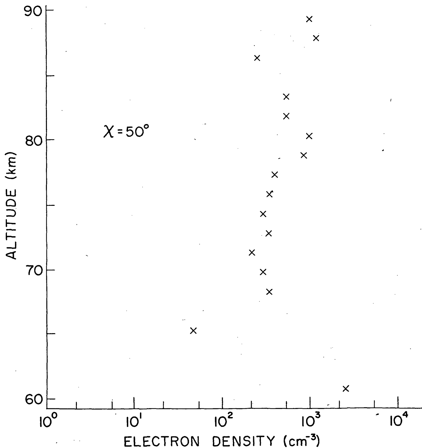
Figure 5.14 Electron-density profile. Date: May 7, 1971, Time: 15:00-15:25 CST.
