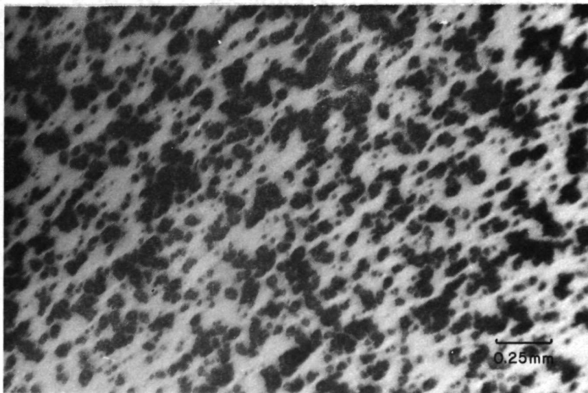
Figure 4-6. Fused \text{SiO}_2 cover glass after dust blasting 72 hours, 100 km/hr., diurnal temperature range. Approximately 40% of the surface is pitted
