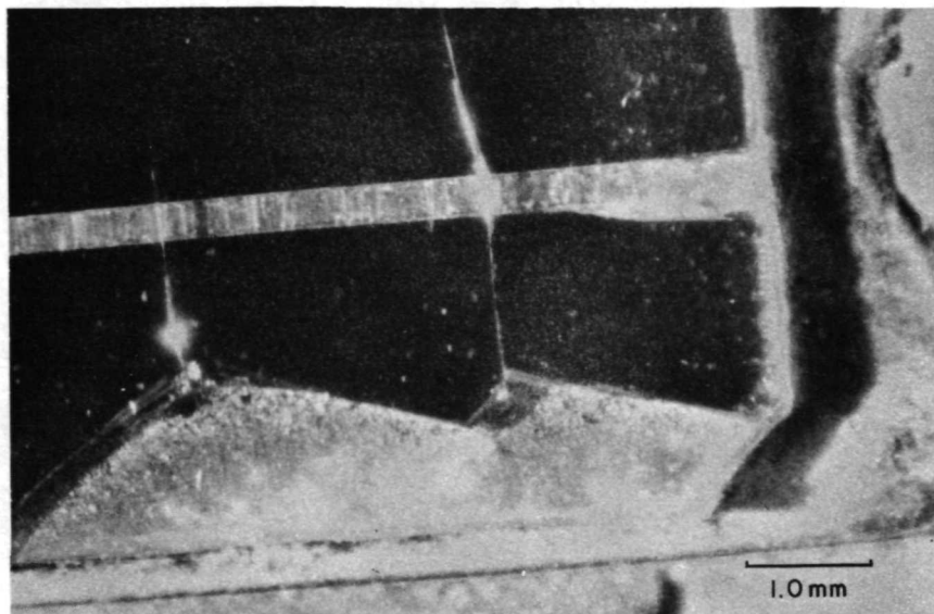
Figure 4-15. Chipped edge of microsheet cover glass after dust balsting 72 hours, 100 km/hr., diurnal temperature range. Oblique illumination
