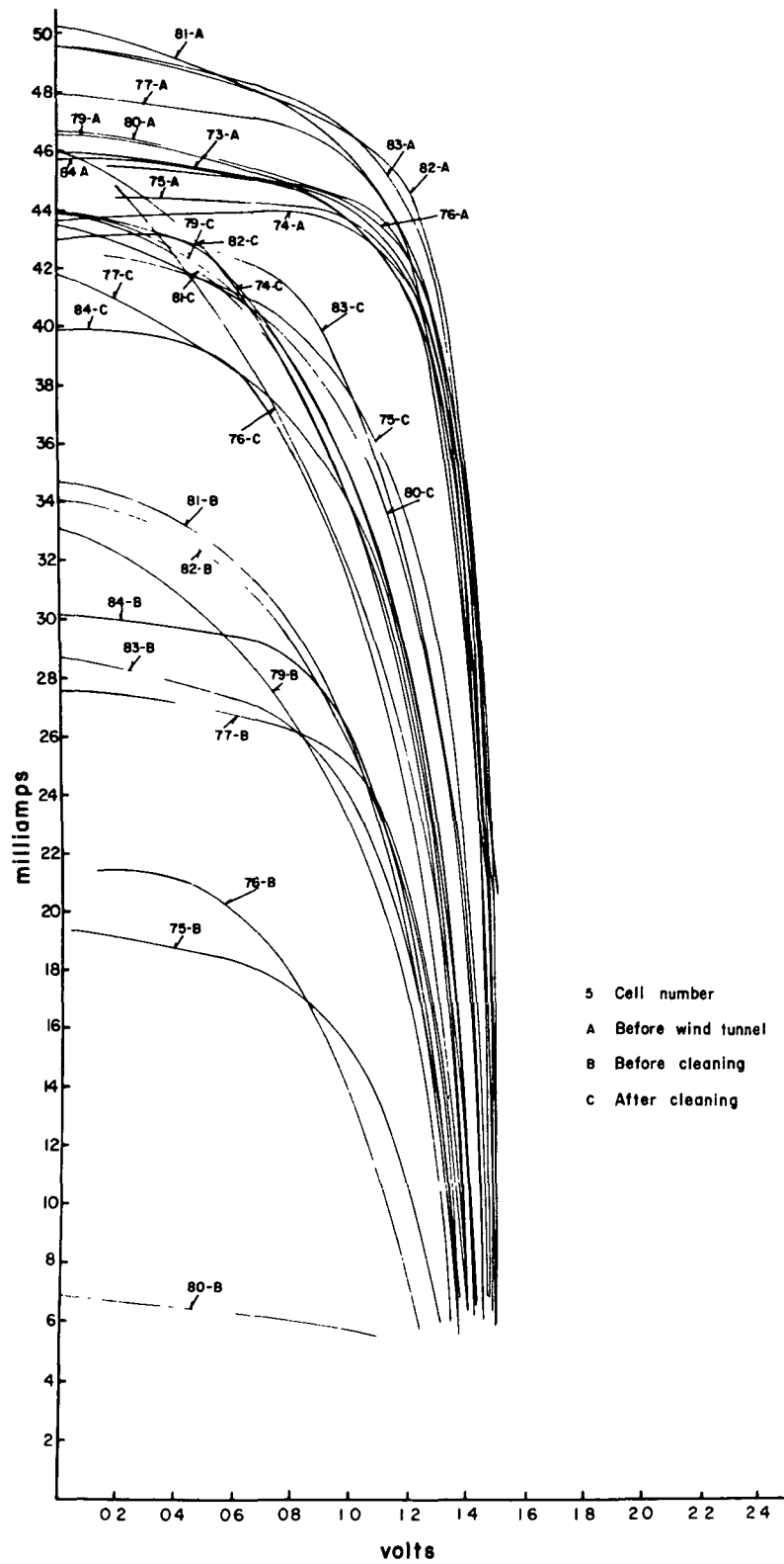
Figure 5-6. I-V Curves. Sapphire. JPL Bus Bar Connectors. Refer to Table 5-3 for cell number identification.
