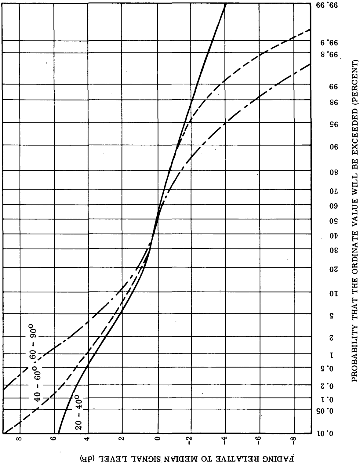
Figure 3-4. Probability Distribution of Signal Fading.
