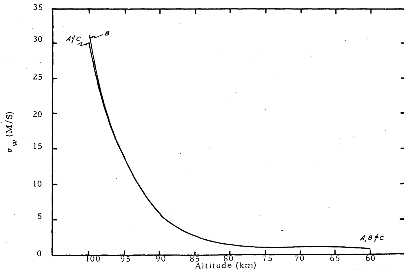
Figure 23 Noise Error in North Wind for Various Launch Directions (Slant Range Radar)
