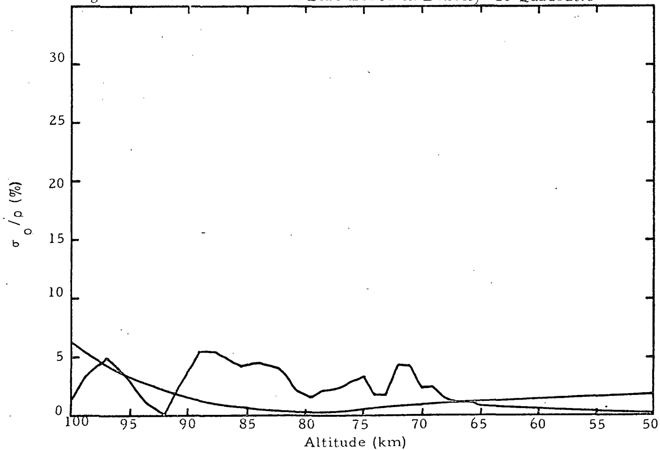
Figure 13i Noise Error and Bias Error in Density 41-11 Cubic-Linear
