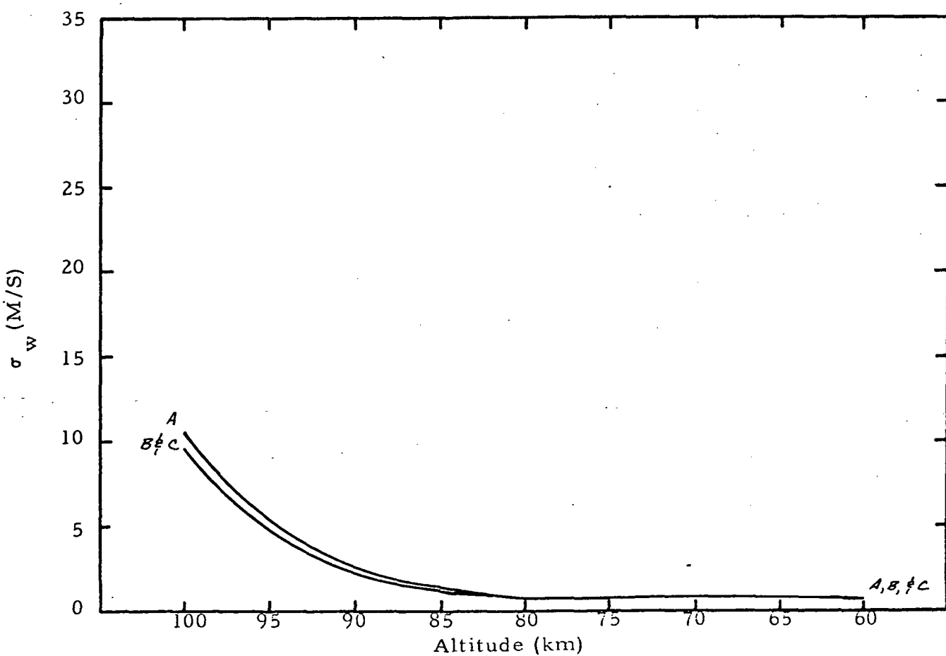
Figure 27 Noise Error in East Wind for Various Launch Directions (Range-Rate Radar)
