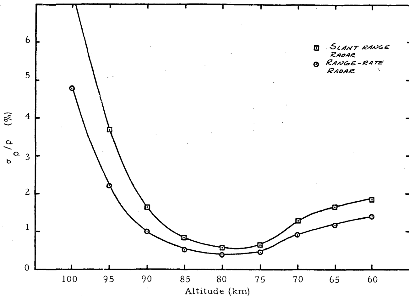
Figure 11 Noise Error in Density for Slant Range and Range-Rate Radar Tracking.
