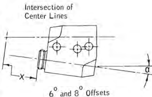
FIGURE 15. SCHEDULE OF STINGS FOR THE 6° AND 8° OFFSETS
