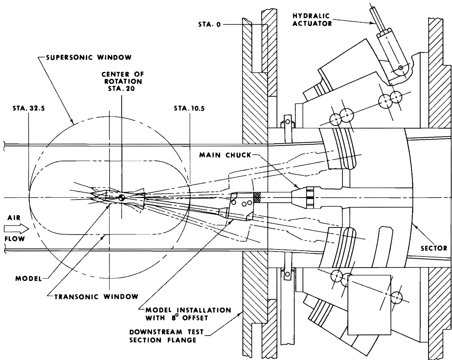
FIGURE 16. MODEL SUPPORT SYSTEM GEOMETRY
