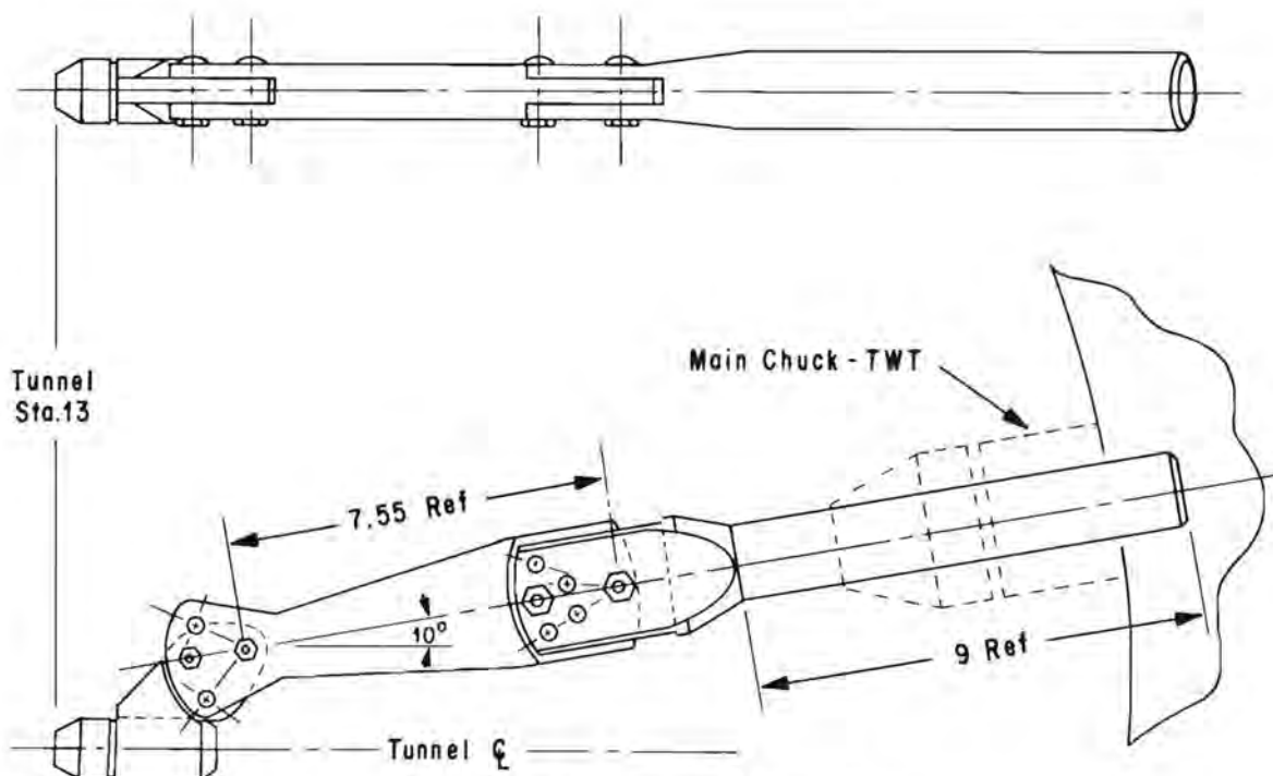
FIGURE 11. KNUCKLE STING
