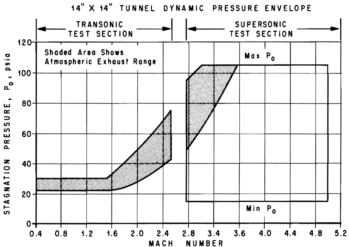
FIGURE 7. STAGNATION AND DYNAMIC PRESSURES
