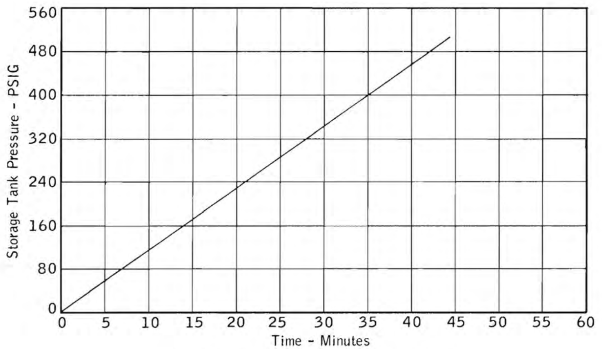
FIG. 5b. COMPRESSOR PUMPING SCHEDULE
