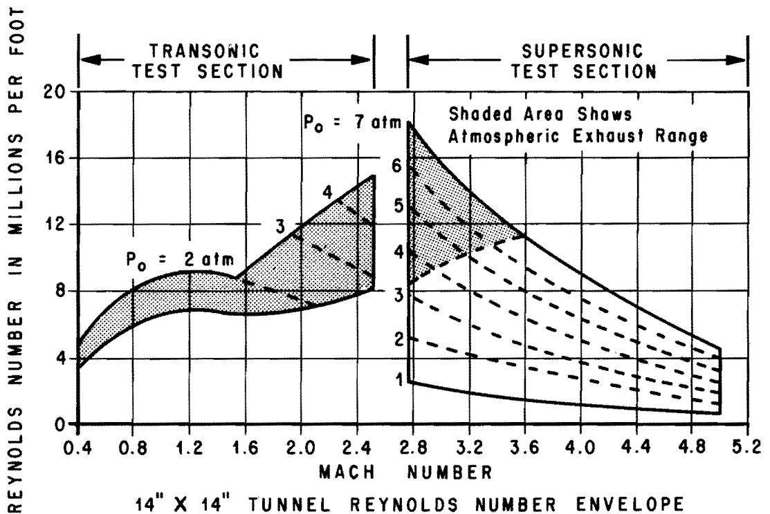
FIGURE 8. REYNOLDS NUMBER AND MASS FLOW VERSUS MACH NUMBER
