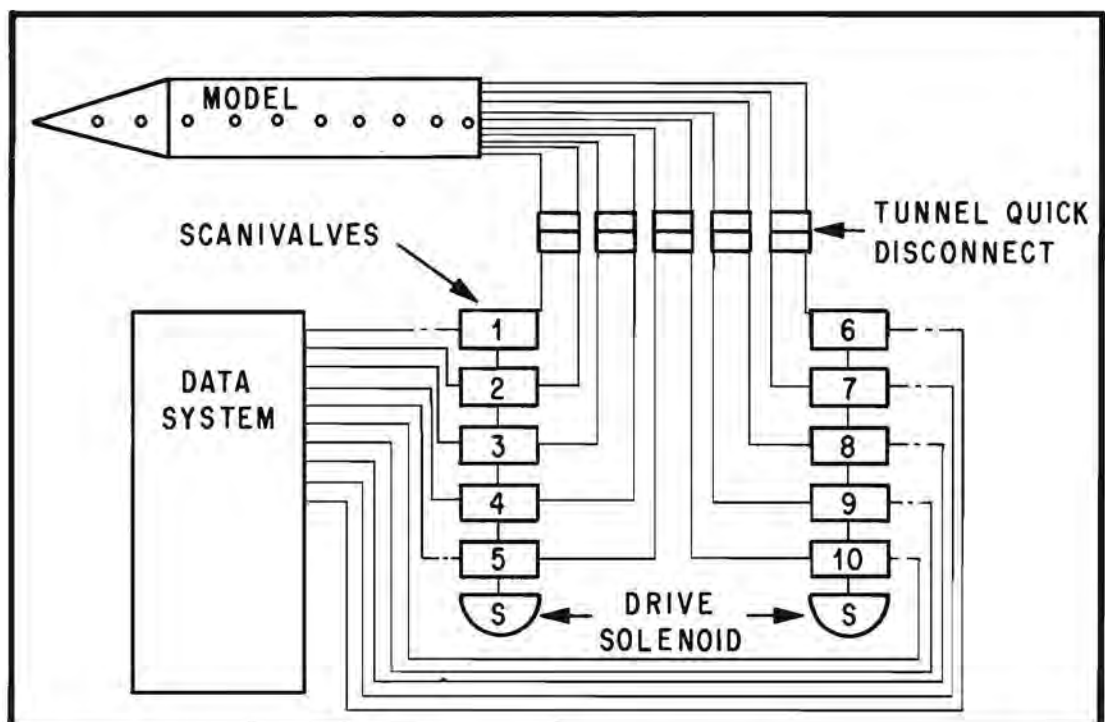
FIGURE 20. SCANIVALVE MODULE
