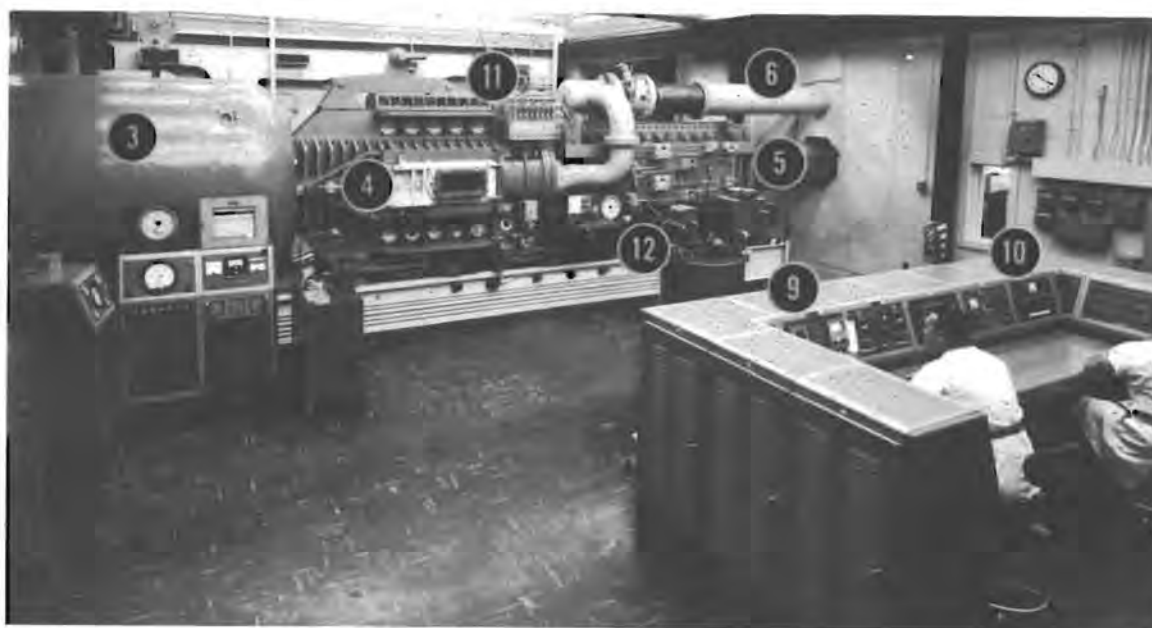
FIGURE 3. 14 x 14-INCH TUNNEL AND CONTROL AREA
