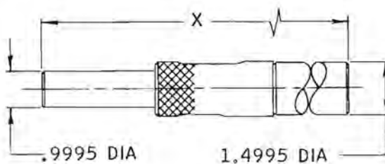
Sting Extension
