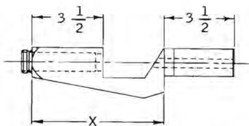
FIGURE 13. PRESSURE STING EXTENSION
