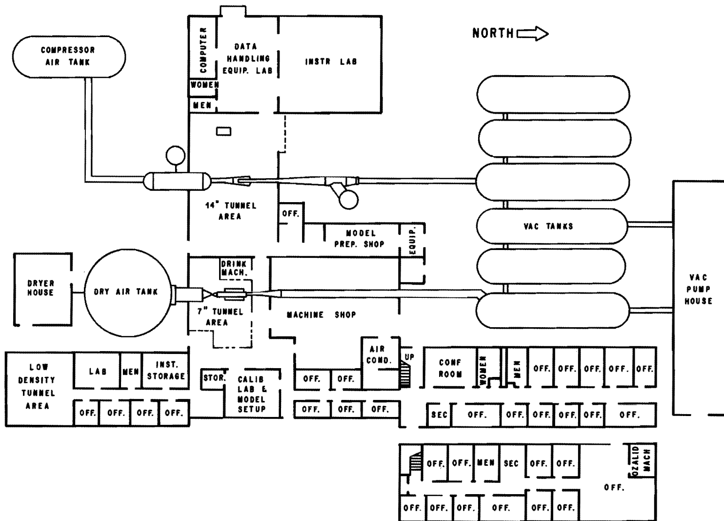
FIGURE 2. LAYOUT OF WIND TUNNEL BUILDING
