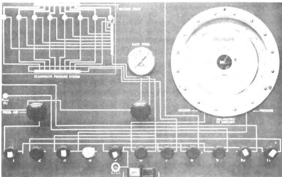
FIGURE 24. PRESSURE CALIBRATION PANEL
