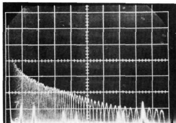
b) Rear Cavity Scribed Plexiglass Disk No Amplifier 1.4 MHz/Div. 10 dB/Div.
