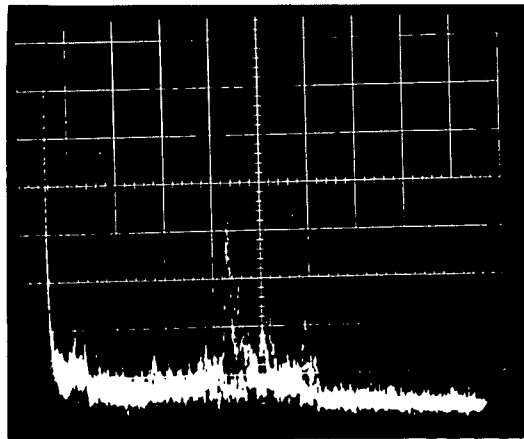
Figure 2-5. Ground Wind Returns, Ft. Collins, Colorado, 31 March 1971 0.5 MHz per Division 5 MHz Full Scale 60 Miles per hour Full Scale
