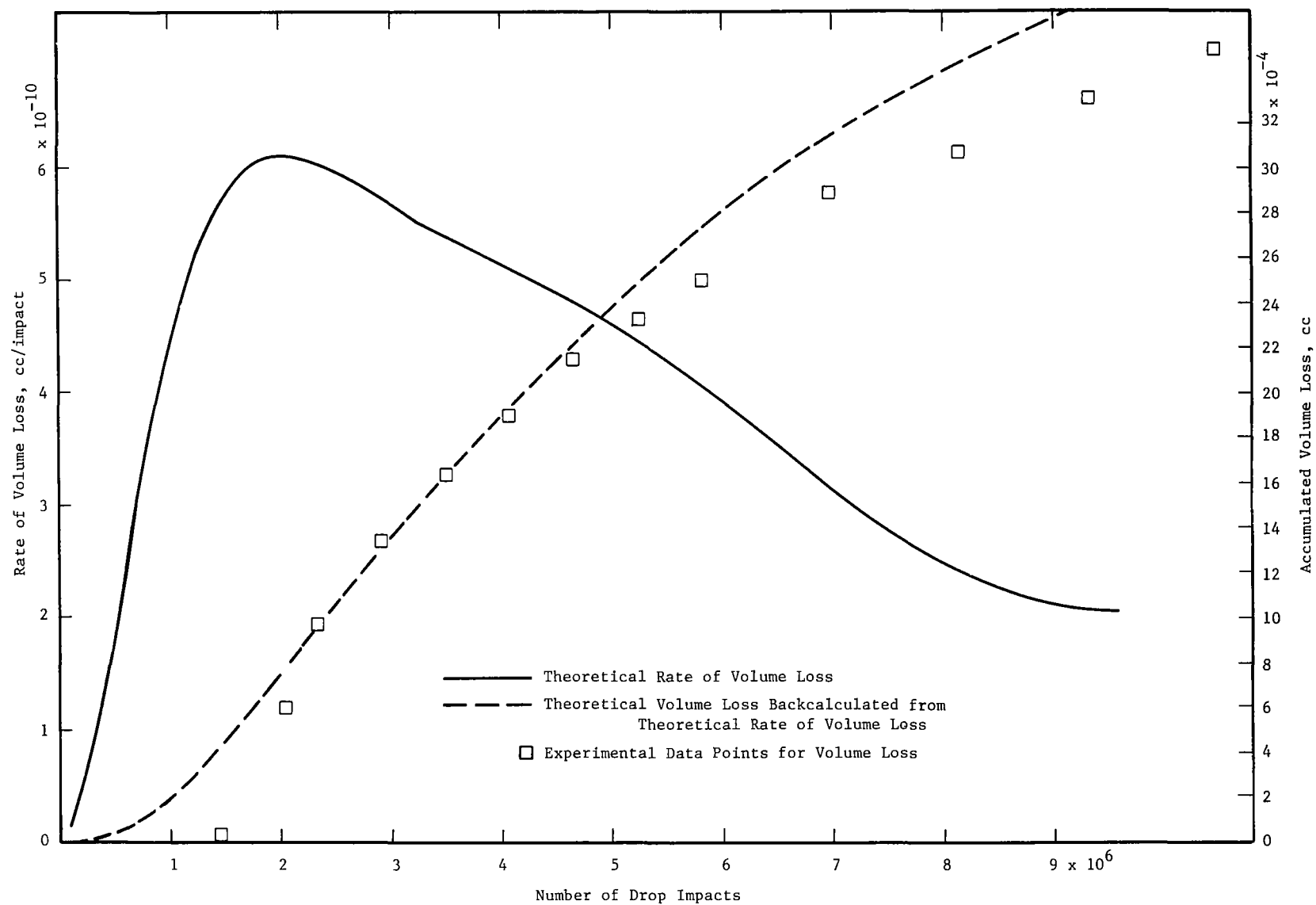
Figure 16. Theoretical Rate-of-Volume-Loss and Accumulated-Volume-Loss Curves for Aged Udimet 700 Calculated with Fragments of Equal Volume.
