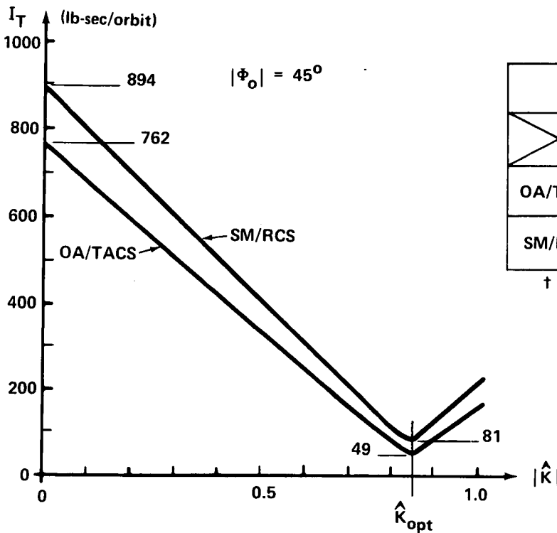
FIGURE 9 - THEORETICAL IMPULSE REQUIREMENT IN THE QI MODE vs \hat{K}
