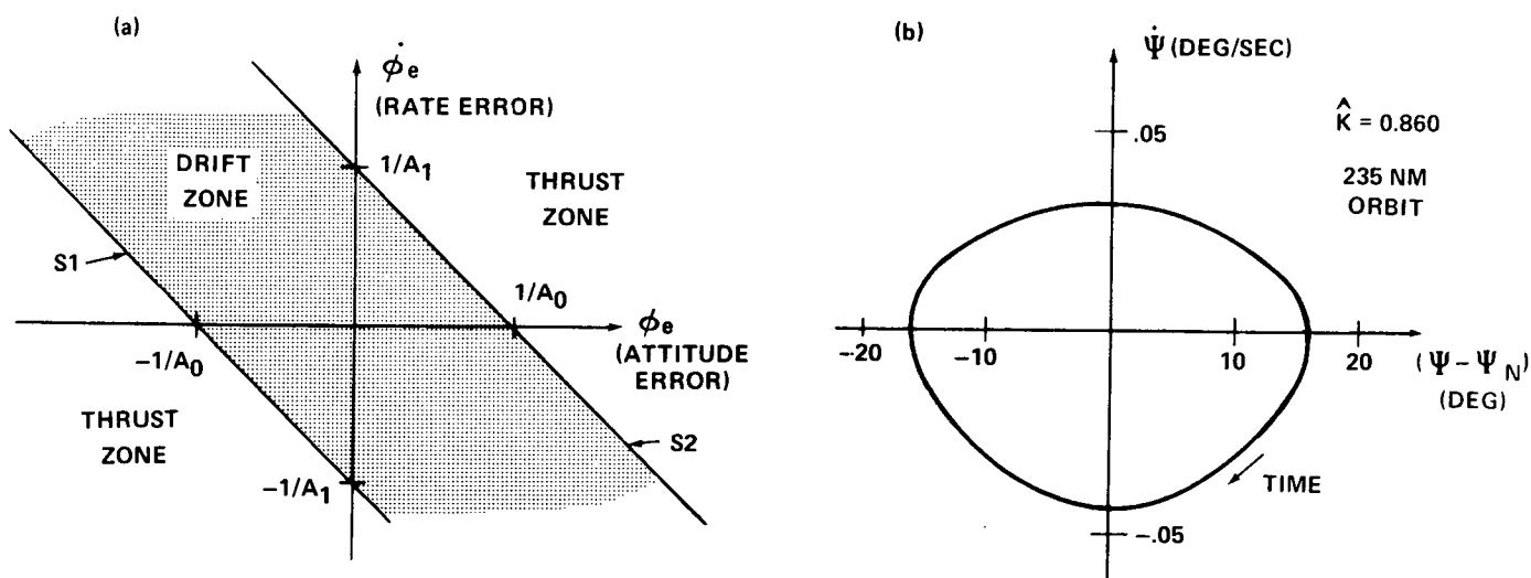
FIGURE 4 - CONTROLLER PHASE PLANE DIAGRAM AND QI MODE PHASE TRAJECTORY
