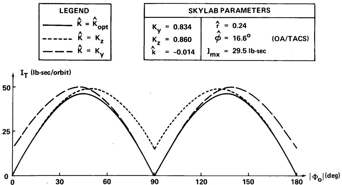
FIGURE 10 - THEORETICAL IMPULSE REQUIREMENT FOR THE QI MODE vs \phi_0 (WITH OA/TACS CONTROL)
