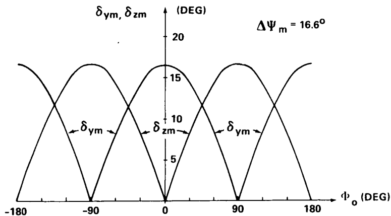
FIGURE A-3 - MAXIMUM INERTIAL POINTING DEVIATION vs \Phi_0
