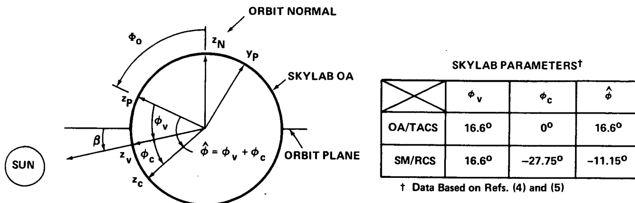
FIGURE 8 - RELATIVE ORIENTATION OF PRINCIPAL, GEOMETRIC AND THRUSTER CONTROL AXES
