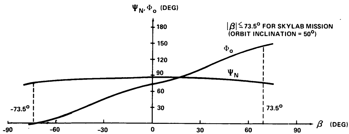
FIGURE A-5 - \Phi_0 AND \Psi_N vs \beta FOR NOMINAL SOLAR ORIENTATION
