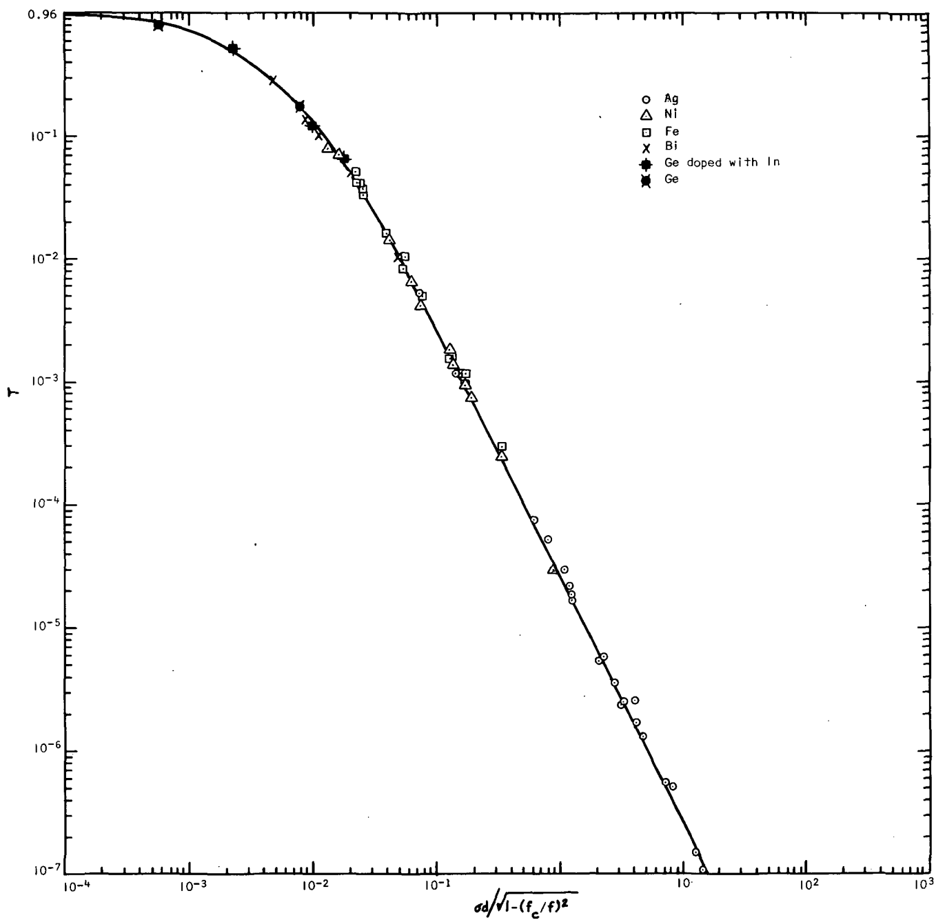
FIGURE 2. THE POWER TRANSMISSION OF THIN FILM WINDOWS IN WAVEGUIDE AS A FUNCTION OF \sigma d .
