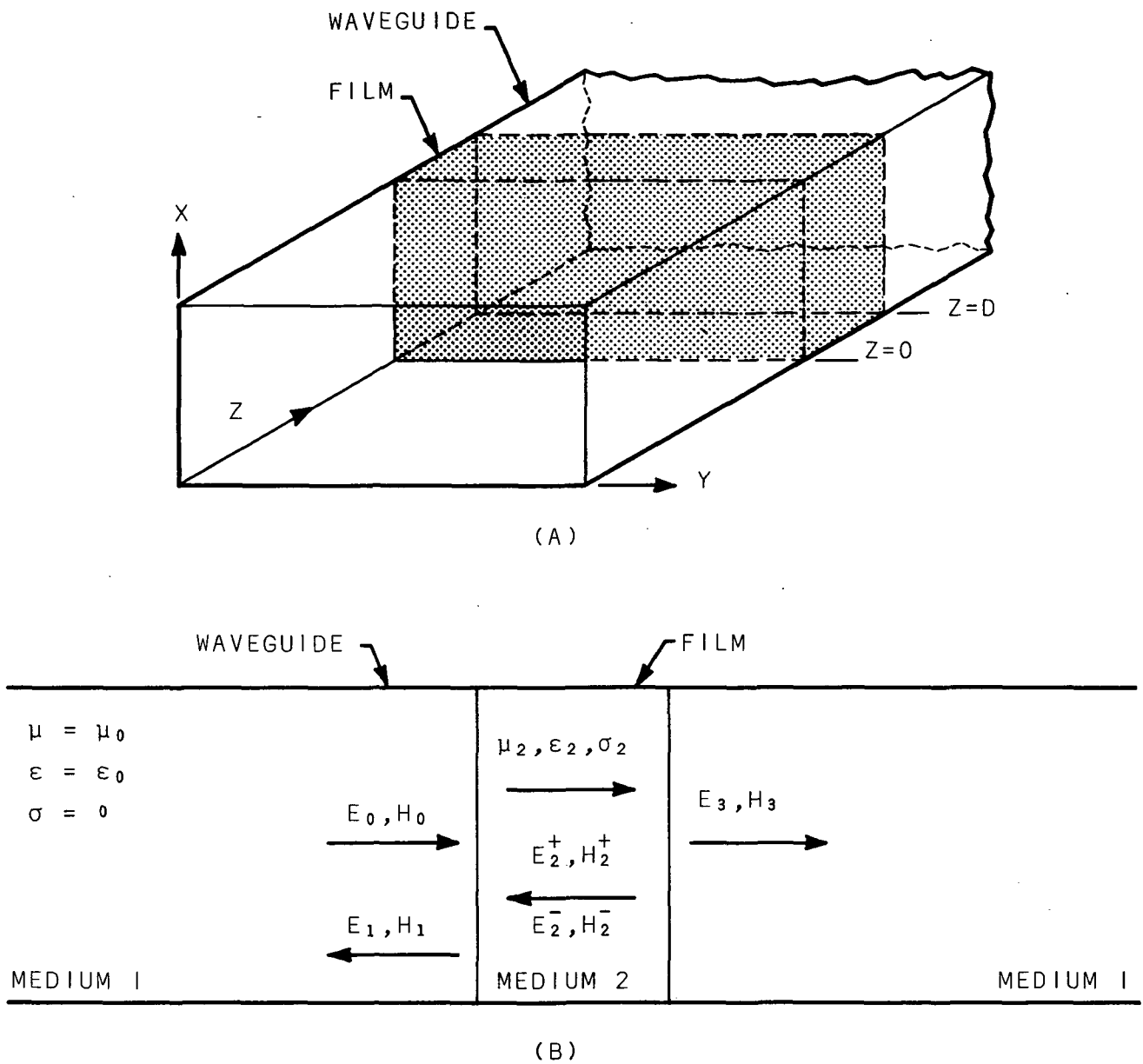
FIGURE 1. (A) FILM AND WAVEGUIDE ORIENTATION FOR BOUNDARY VALUE. (B) IDENTIFICATION OF FIELD COMPONENTS AND MEDIA PARAMETERS.
