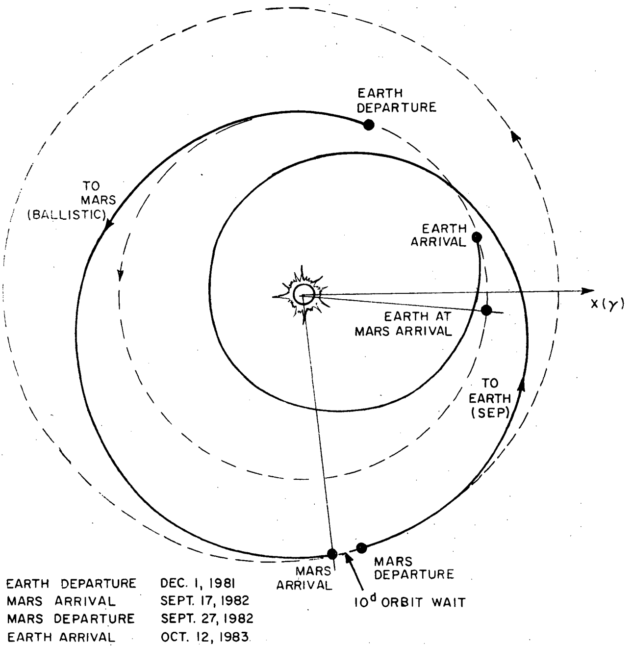
FIGURE 21. TRAJECTORY PROFILE FOR 680 d MSR MISSION
