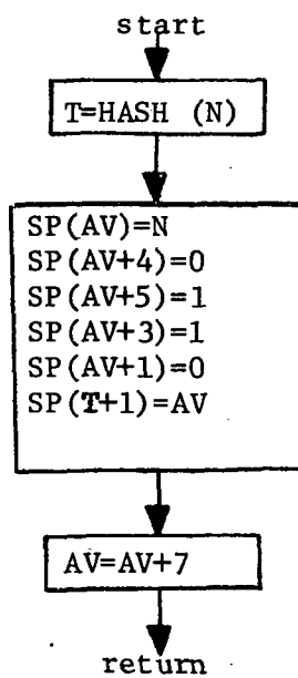
(b) table routine EXEC5
