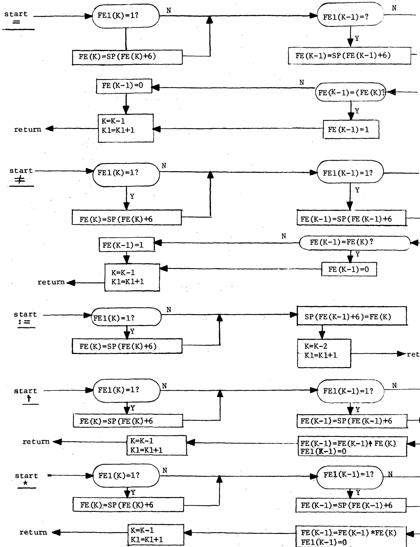
Fig. 16 Flowcharts of = , \neq , := , \dagger , and * routine
