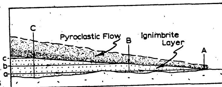
Fig. 8. Diagrammatic illustration of a moving pyroclastic flow and its gradually thickening ignimbrite deposit. Particles along line "a" were deposited from the portion of the flow that has reached station A. Particles along line "b" were deposited from the portion of the flow that has reached station B and so on through innumerable theoretical lines parallel to the base of the deposit deposited by innumerable theoretical turbulent "fronts" that follow the leading edge of the pyroclastic flow.
