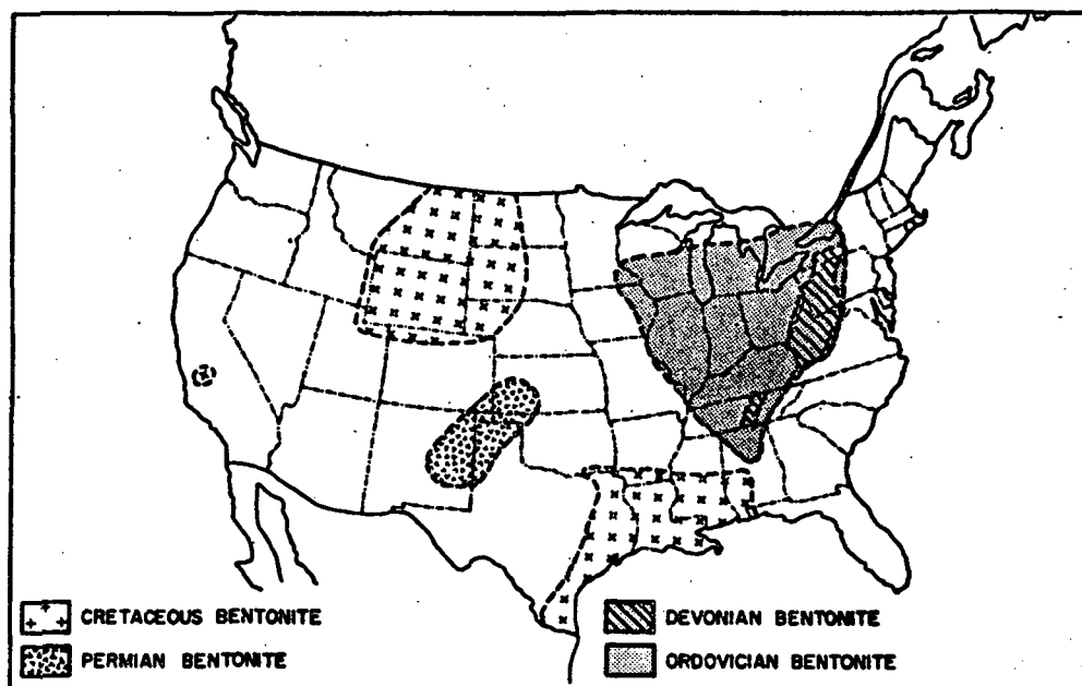
FIG. 11.—Geographic distribution of pre-Tertiary volcanic ash and bentonite in the continental United States. The areas outlined could serve as starting points for studies of high-altitude winds in the geologic past (data from Hass, 1948; Flowers, 1952; Ross, 1955; Marsh, 1960; and Reeside and Cobban, 1960). From Eaton (1963).
