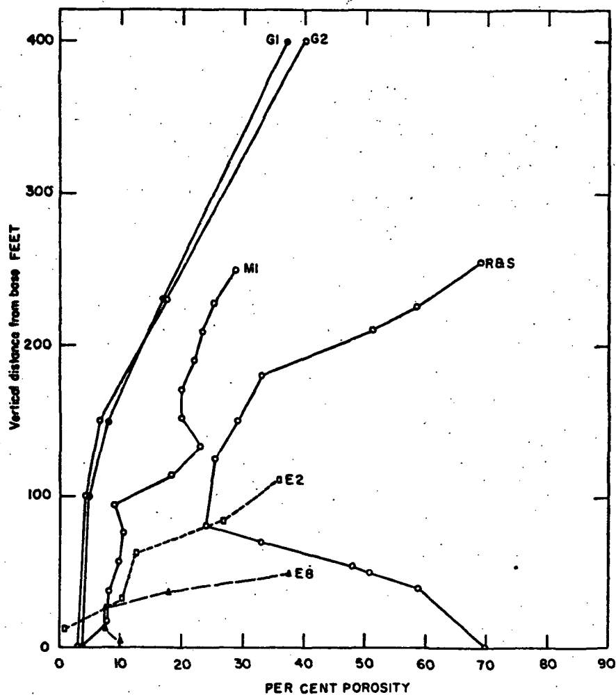
FIGURE 14.—POROSITY CURVES FOR WELDED-TUFF SHEETS
