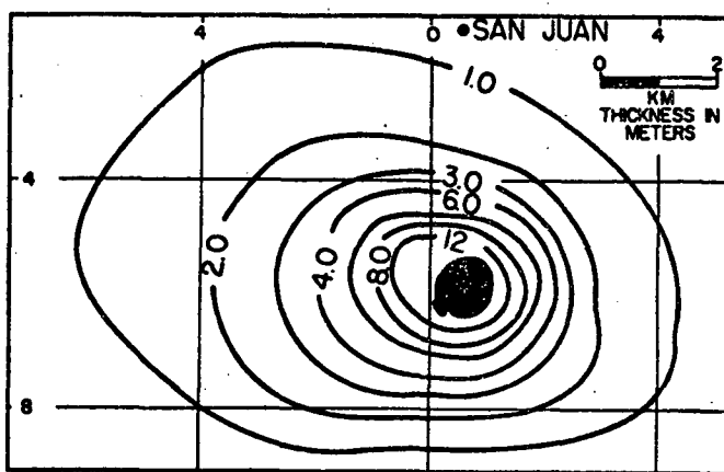
PARICUTIN, MEXICO
