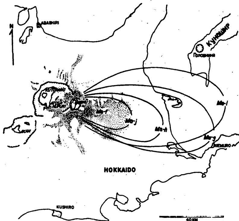
Fig. 9. Map showing the distribution of the Mashu pyroclastic deposits erupted during the culminating phase.
