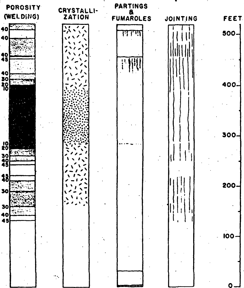
FIG. 16 - A sample stratigraphic section of the upper member of the Bandelier Tuff, showing recorded changes in degree of welding (percent porosity, shaded), crystallization, (vapor phase, dashed; devitrification, dotted) position of partings and fumaroles, and spacing of joints.
