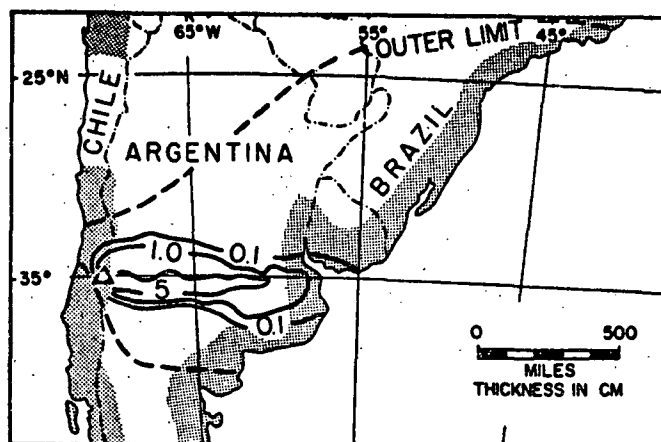
QUIZAPU, CHILE
