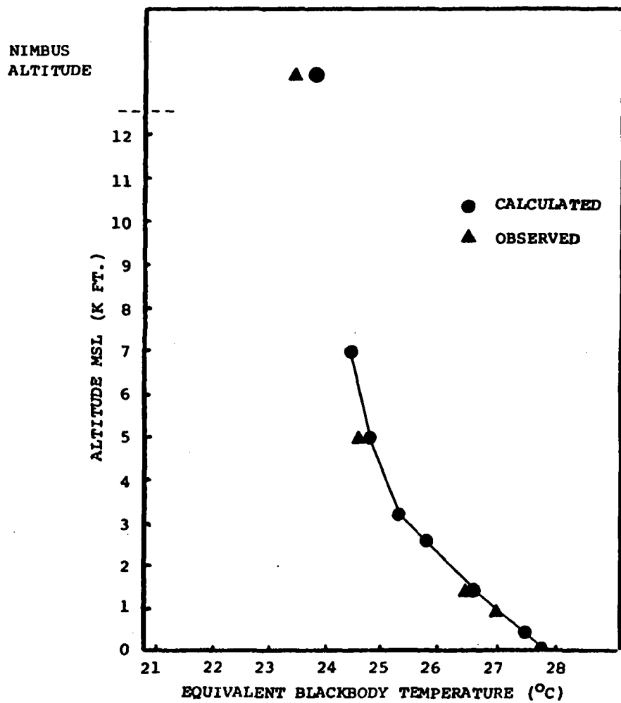
FIGURE 4. COMPARISON OF OBSERVED AND CALCULATED SEA SURFACE TEMPERATURES FOR JULY 13, 1969.
