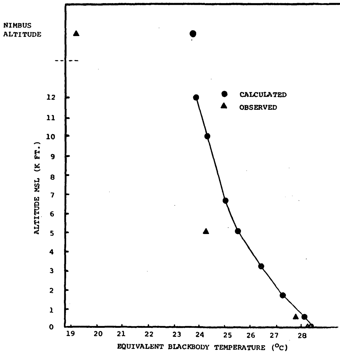
FIGURE 6. COMPARISON OF OBSERVED AND CALCULATED SEA SURFACE TEMPERATURES FOR JULY 18, 1969.
