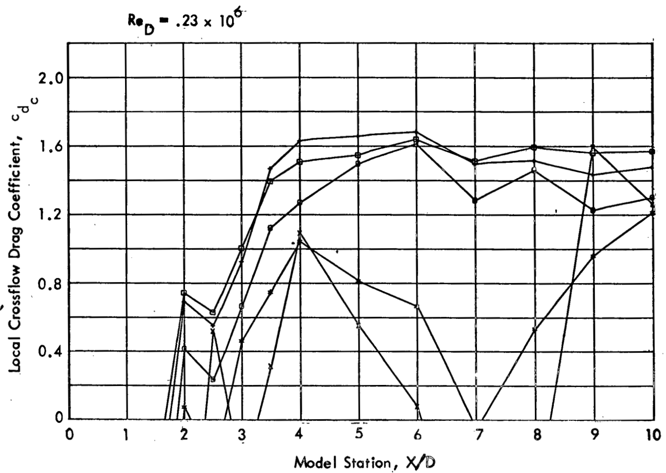
Figure 18. Local Crossflow Drag Coefficient vs. Model Station, Ogive-Cylinder Configuration (concluded)
