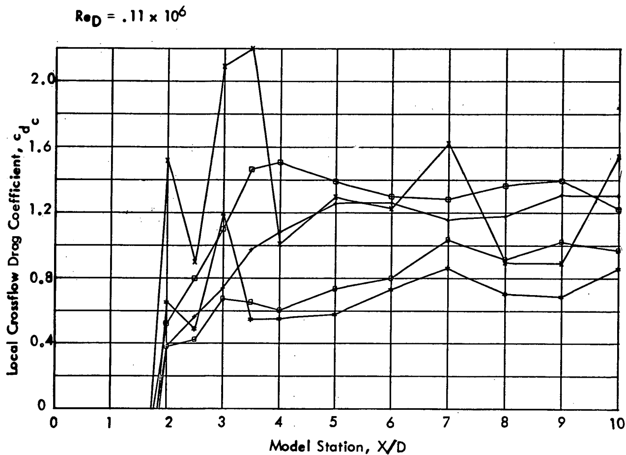
Figure 18. Local Crossflow Drag Coefficient vs. Model Station, Ogive-Cylinder Configuration
