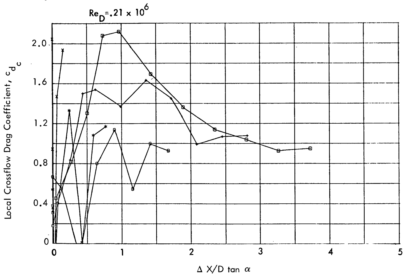
Figure 21. Local Crossflow Drag Coefficient vs \Delta X/D \tan \alpha , Ogive-Cylinder Configuration (continued)
