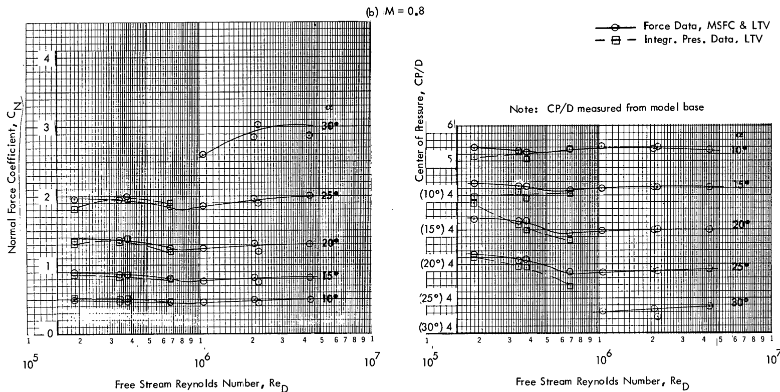
Figure 5. Ogive-Cylinder - Frustum-Cylinder Normal Force and Center of Pressure (continued)
