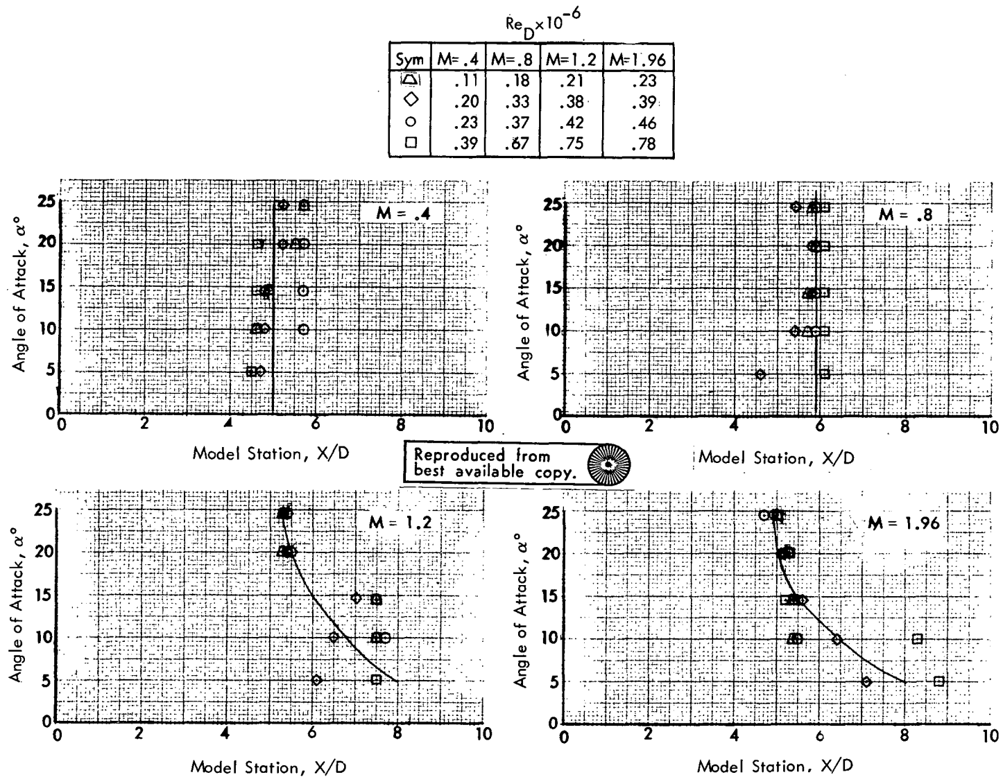
Figure 24. Axial Location of Initial Crossflow Separation, O/C/F/C Aft Cylinder
