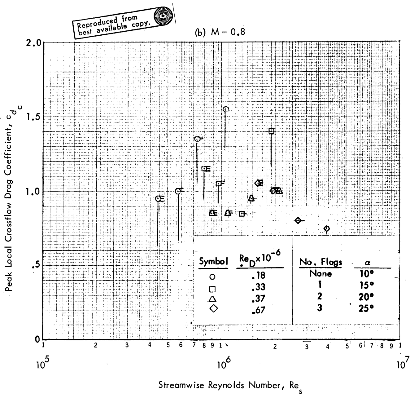
Figure 23. Correlation of Peak Local Crossflow Drag Coefficient, O/C/F/C Aft Cylinder (concluded)
