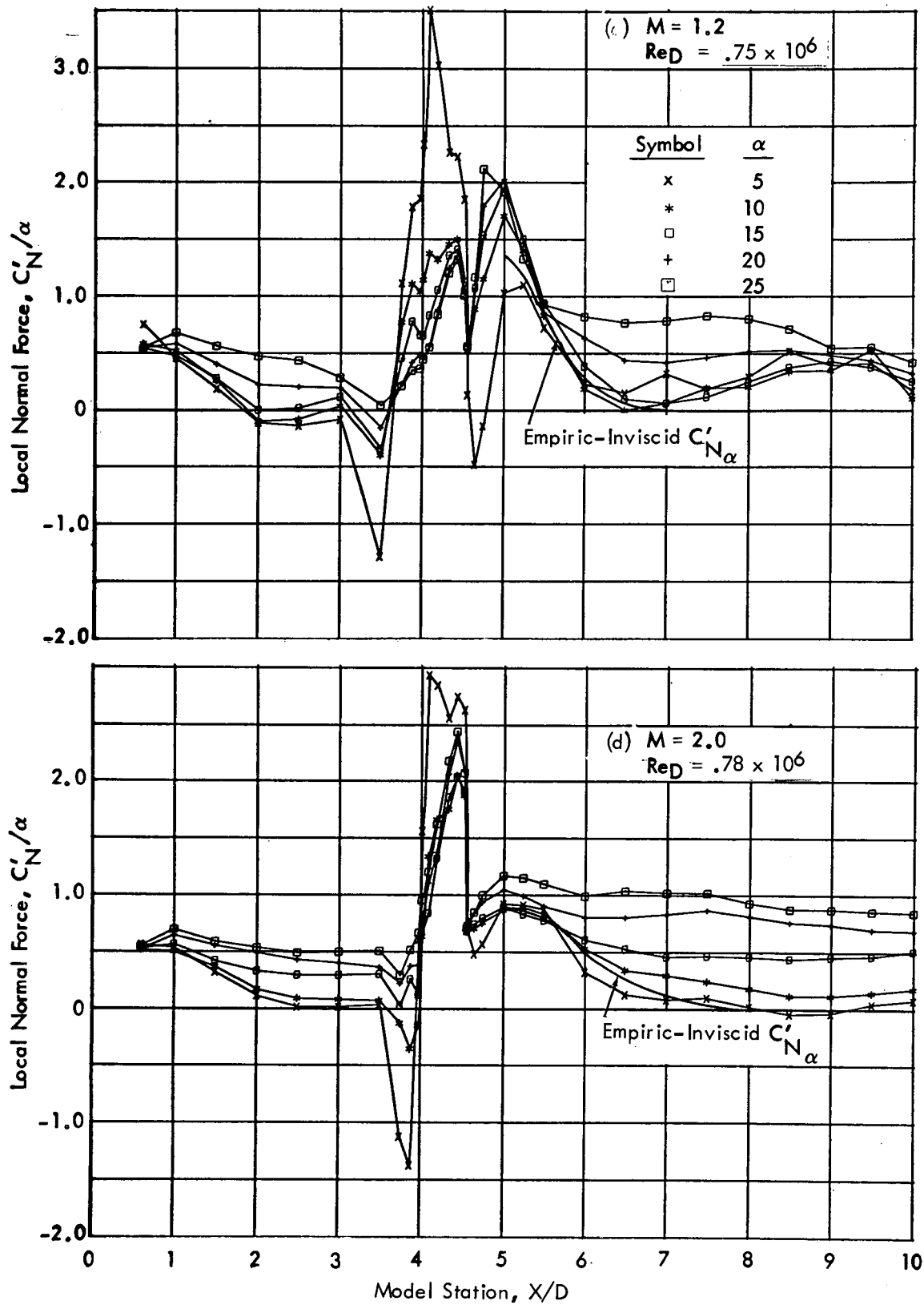
Figure 16. Local Normal Force Distributions, Ogive-Cylinder-Frustum-Cylinder (concluded)
