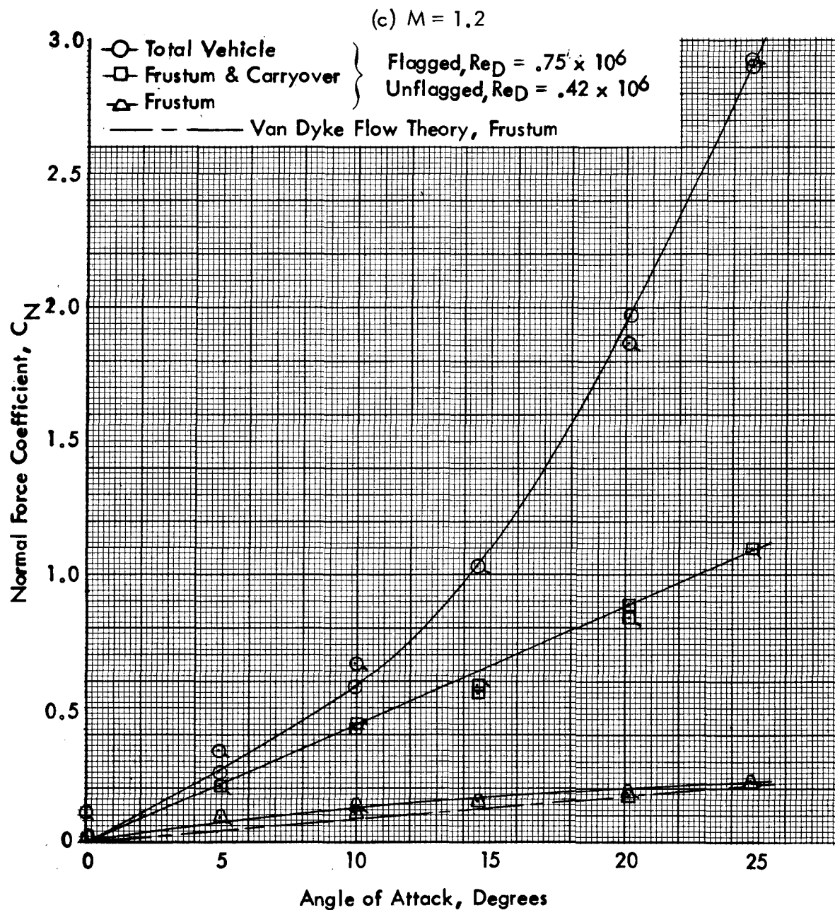
Figure 17. Component Normal Force Coefficients, O/C/F/C (continued)
