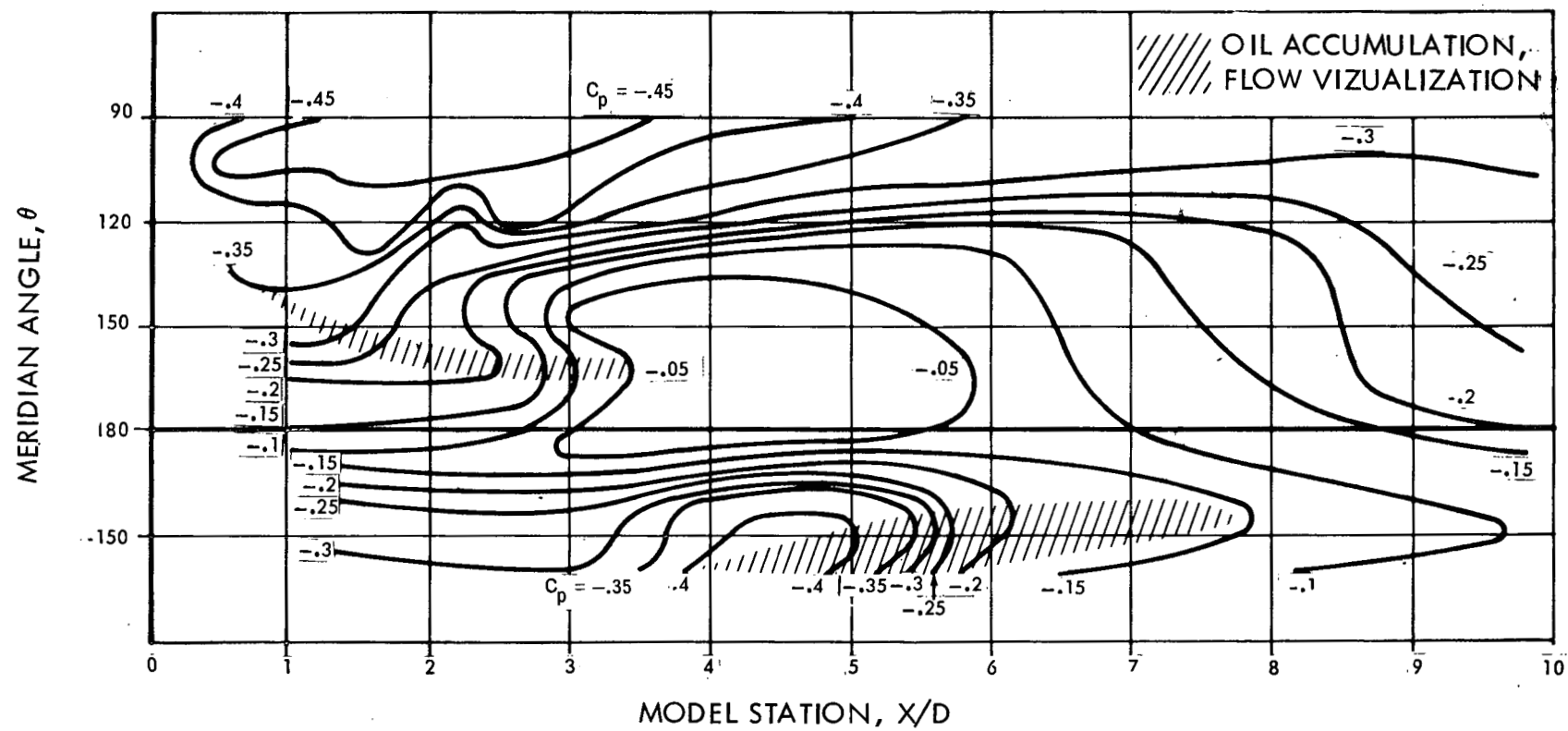
Figure 11. Surface Pressures on Lee Side of Ogive-Cylinder
