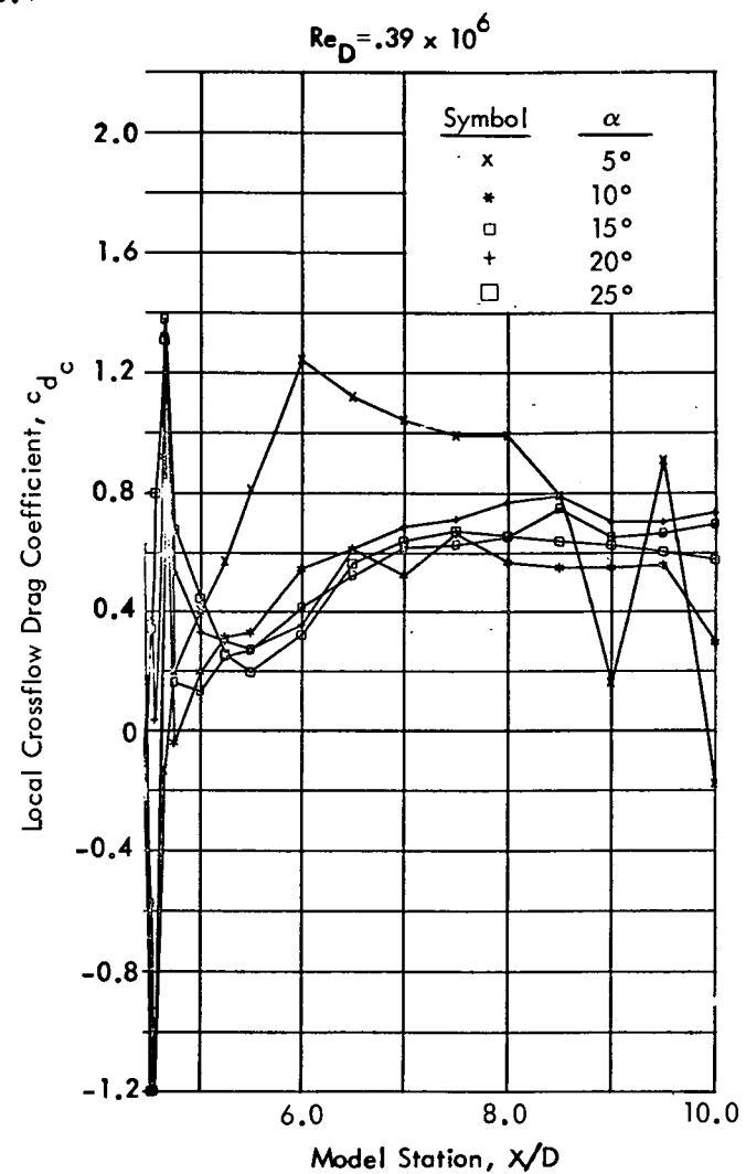
Figure 22. Local Crossflow Drag Coefficient vs Model Station, Aft Cylinder of O/C/F/C Configuration (Shee
