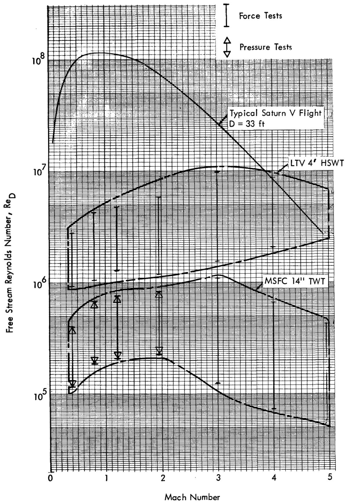
Figure 3. Mach/Reynolds No. Test Conditions - MSFC "Non-Linear-Lift" Research Program
