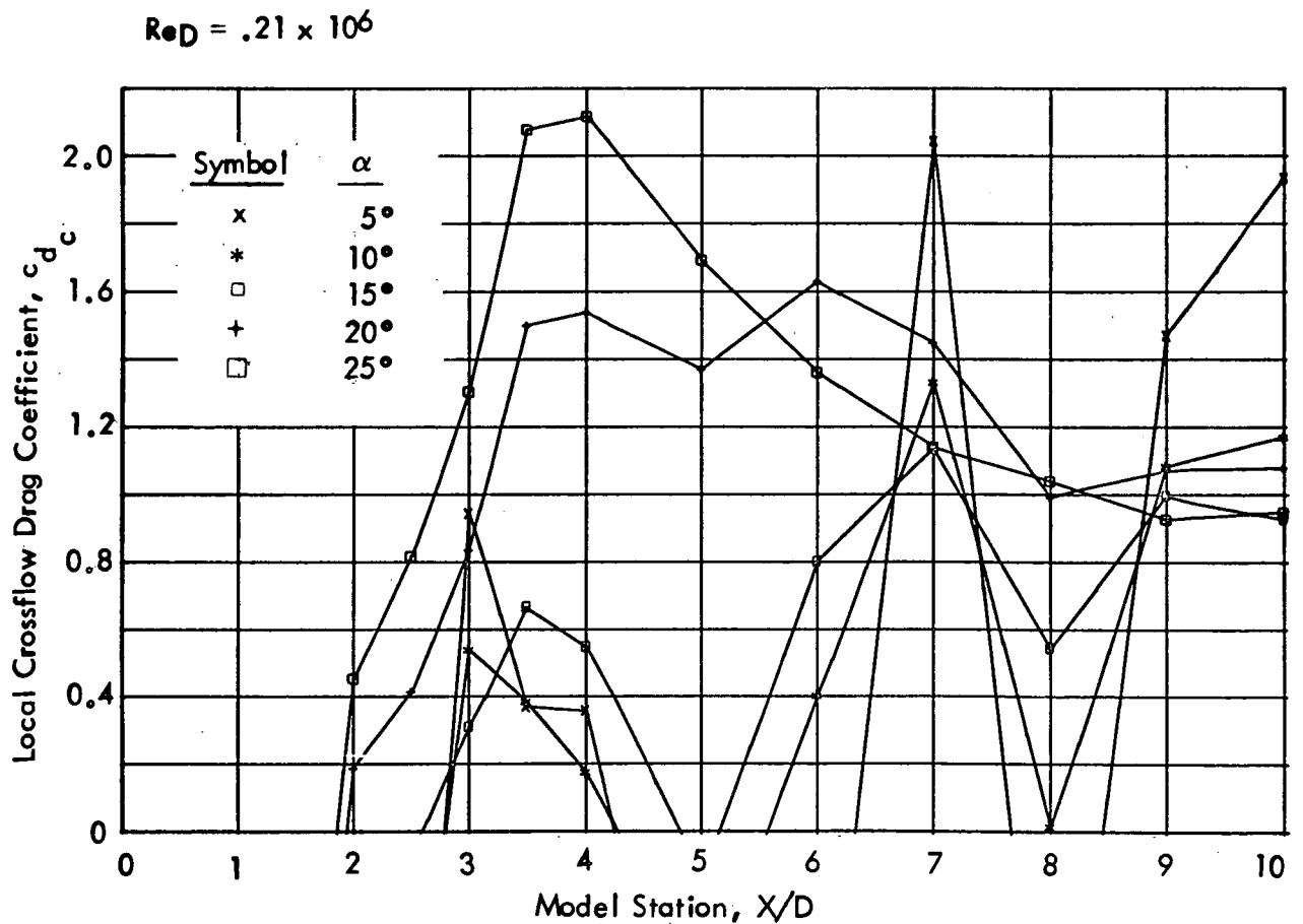
Figure 18. Local Crossflow Drag Coefficient vs. Model Station, Ogive-Cylinder Configuration (continued)
