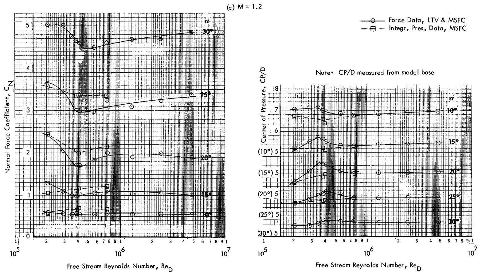
Figure 4. Ogive-Cylinder Normal Force and Center of Pressure (continued)
