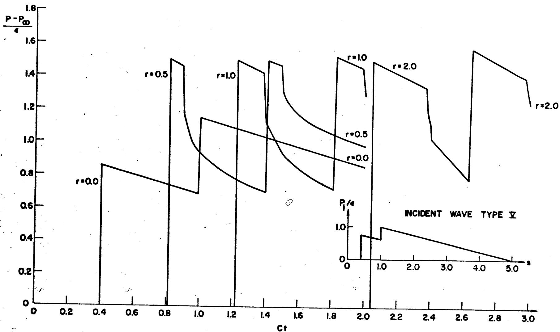
Fig. 10 Pressure signature received at points along line \theta = \pi/2 , \phi = \pi for plane wave incident at equal angles with the edges and with wave form at type V
