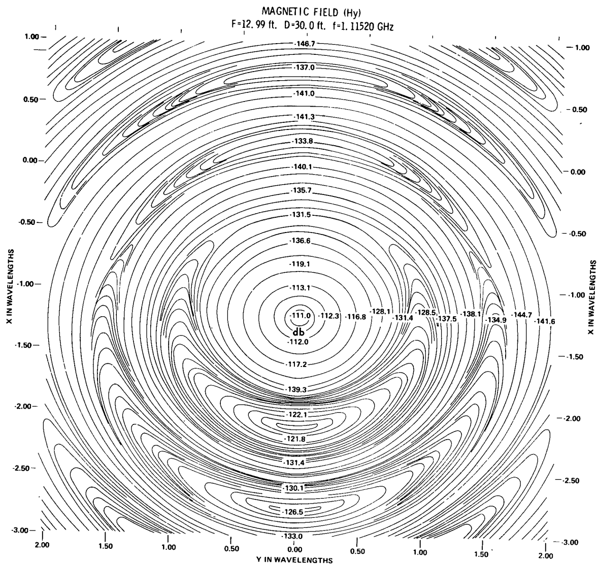
Figure 11. Airy disc and rings (paraxial reception)
