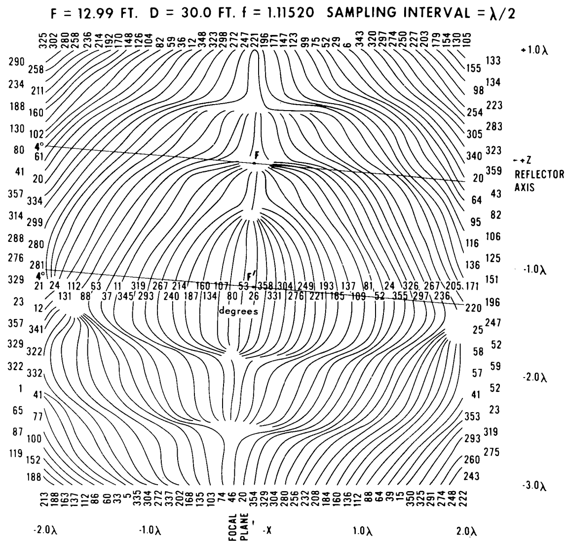
Figure 12. Phase of magnetic field near focal plane (paraxial reception)
