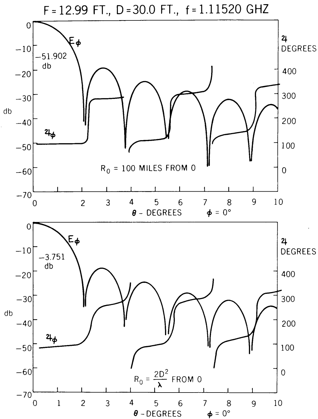
Figure 2. Electric Field vs. Angle \theta
