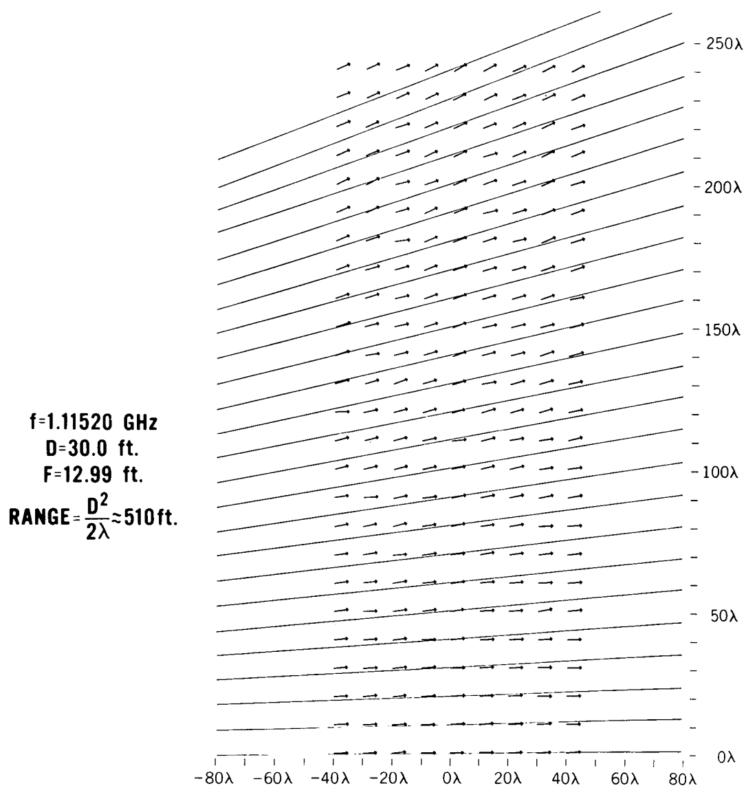
Figure 4. Direction of the time-average Pointing vector
