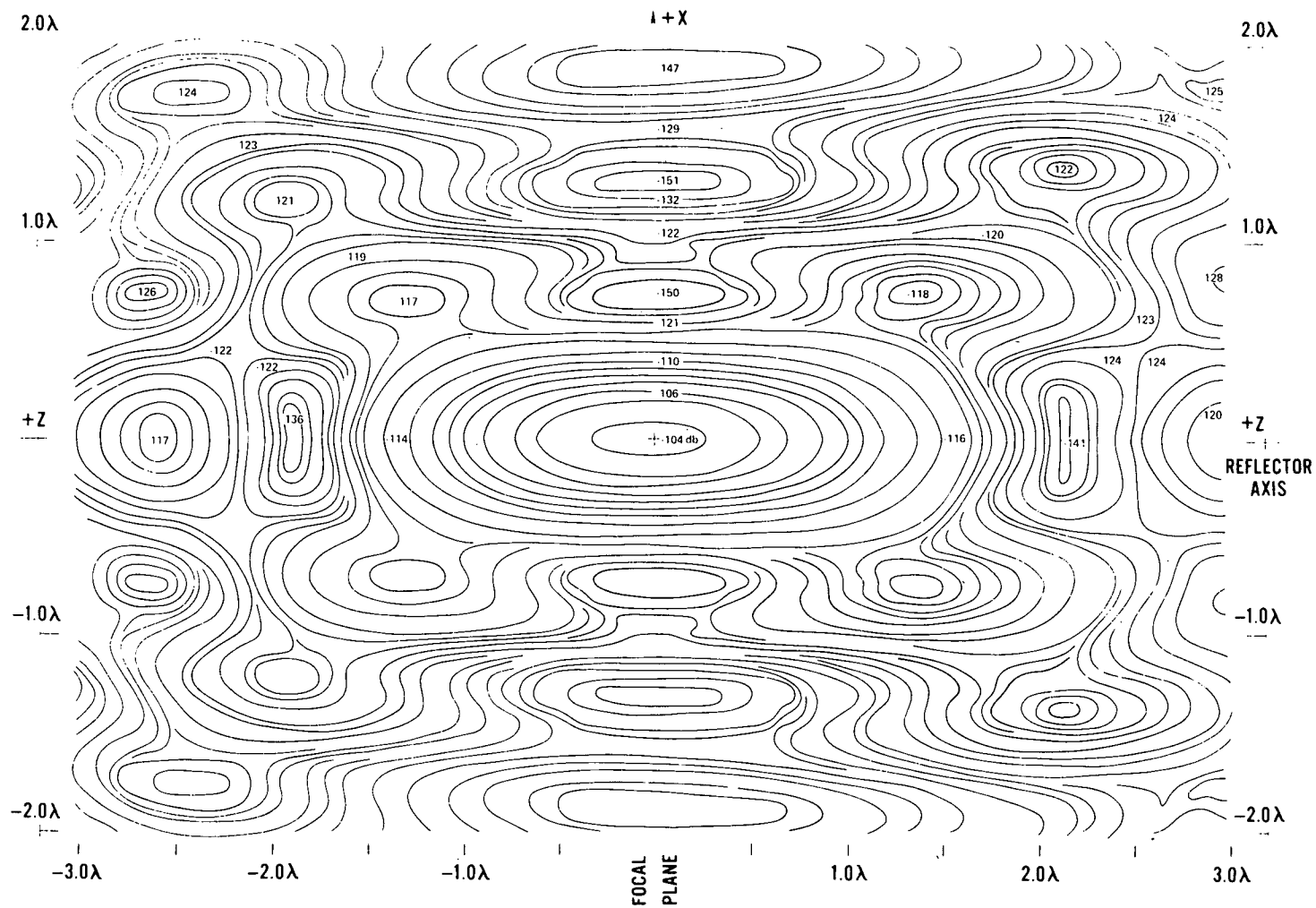
Figure 5. Amplitude of magnetic field near focal-plane (axial reception)
