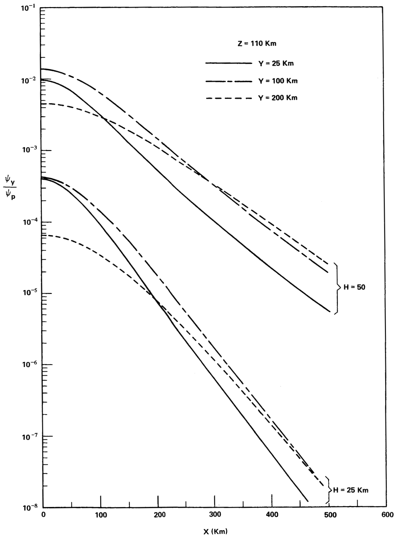
FIGURE 3 - Y-FLUX VARIATIONS VS X AT Z = 110 Km IN THE CASE OF A POINT SOURCE
