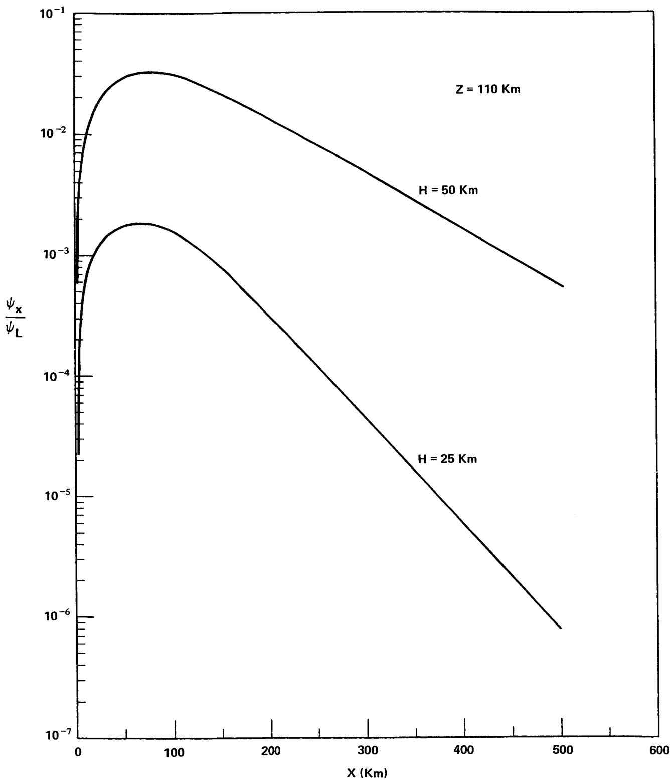
FIGURE 5 - X-FLUX VARIATIONS VS X AT Z = 110 Km IN THE CASE OF A LINE SOURCE
