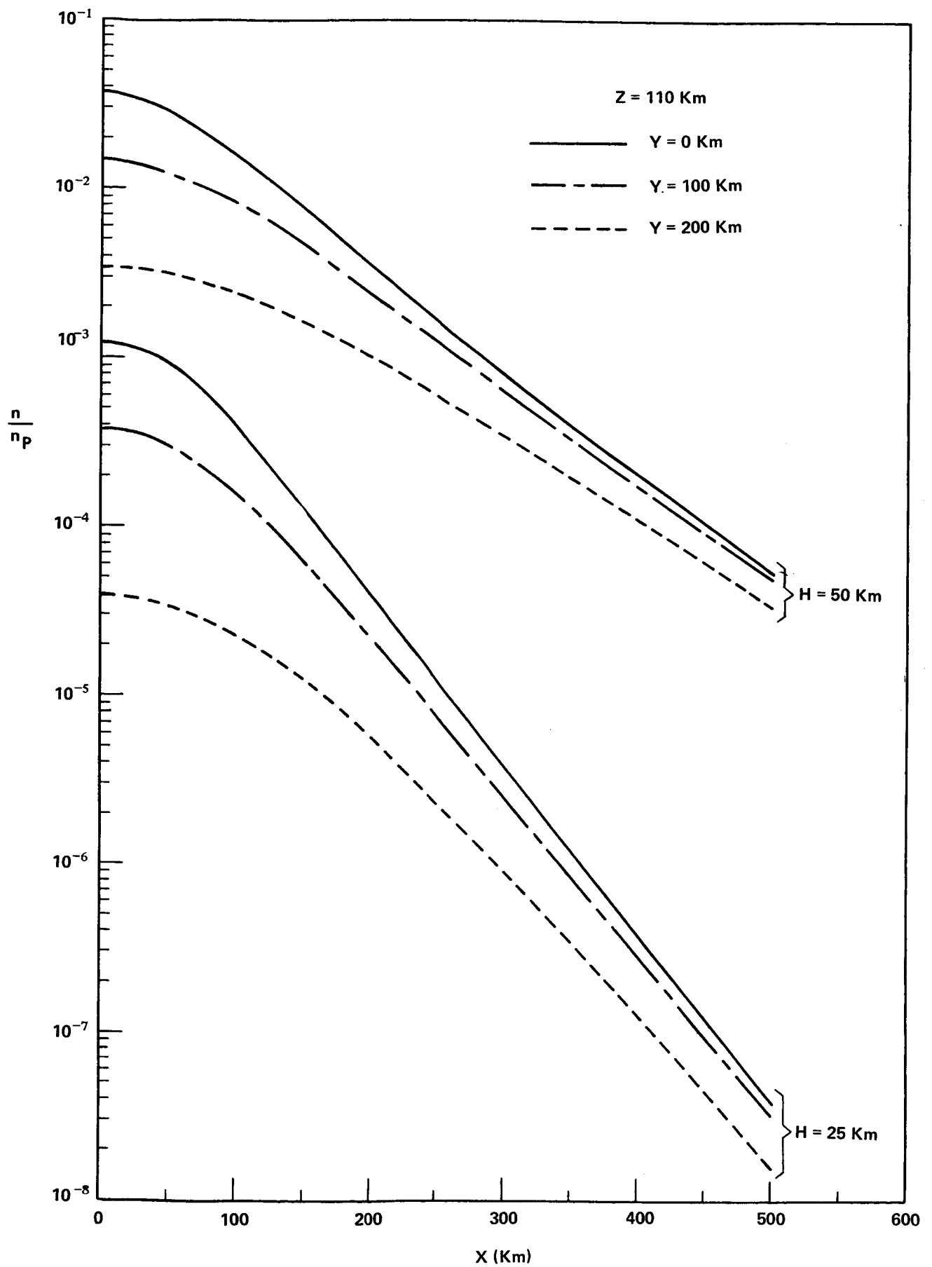
FIGURE 1 - DENSITY VARIATION VS X AT Z = 110 \text{ Km} IN THE CASE OF A POINT SOURCE
