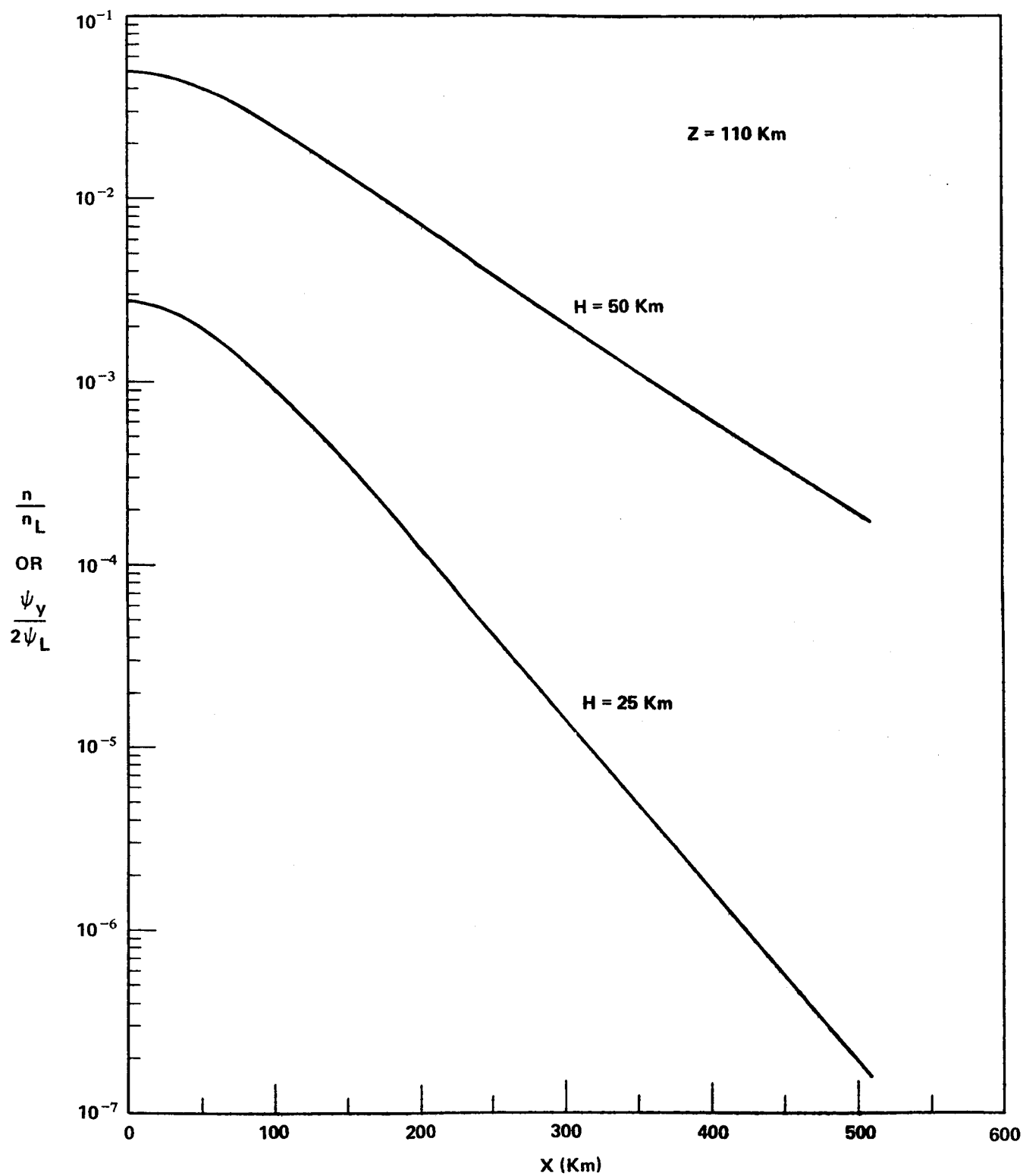
FIGURE 4 - DENSITY AND Y-FLUX VARIATIONS VS X AT Z = 110 Km IN THE CASE OF A LINE SOURCE
