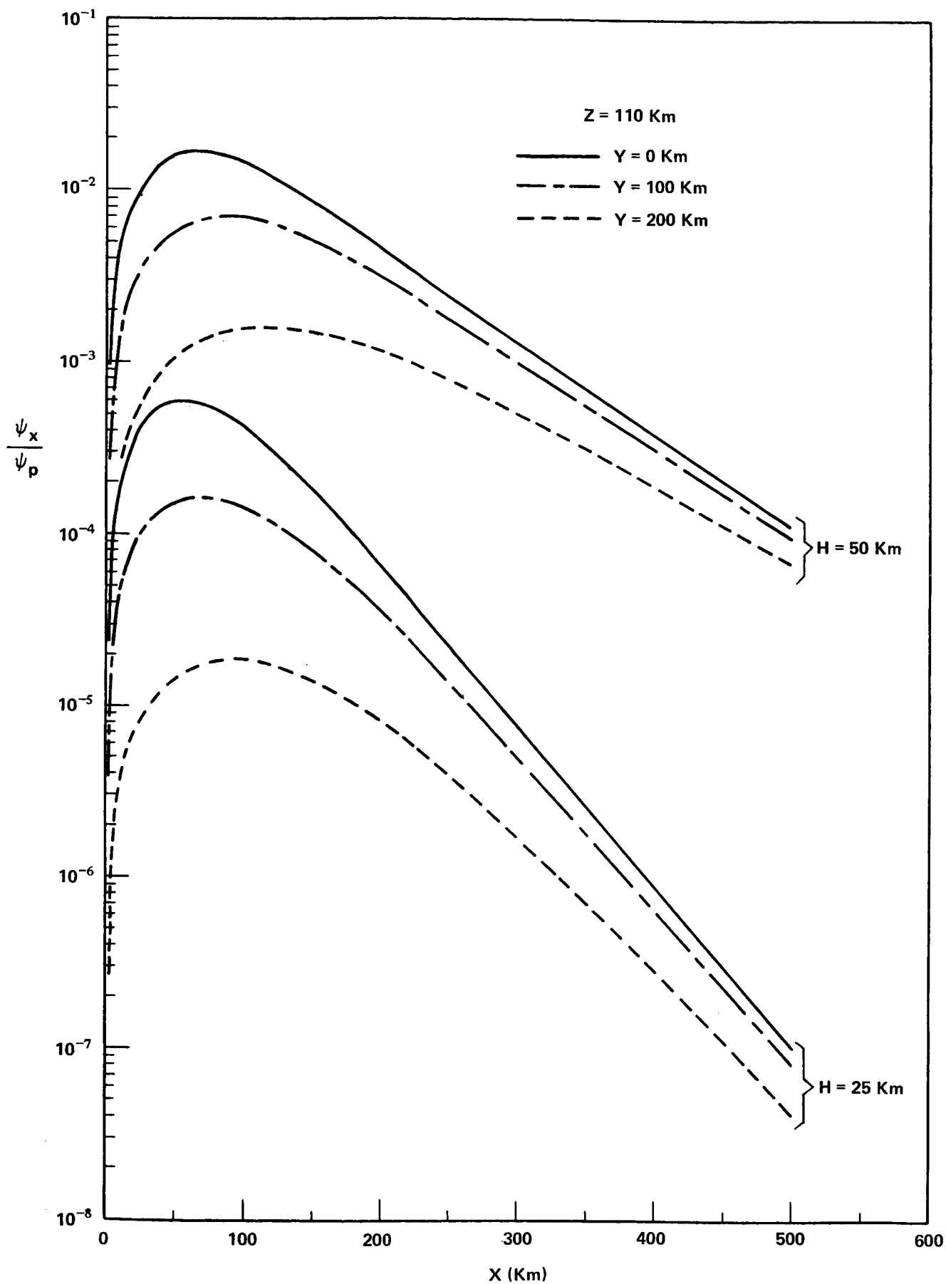
FIGURE 2 - X-FLUX VARIATIONS VS X AT Z = 110 Km IN THE CASE OF A POINT SOURCE
