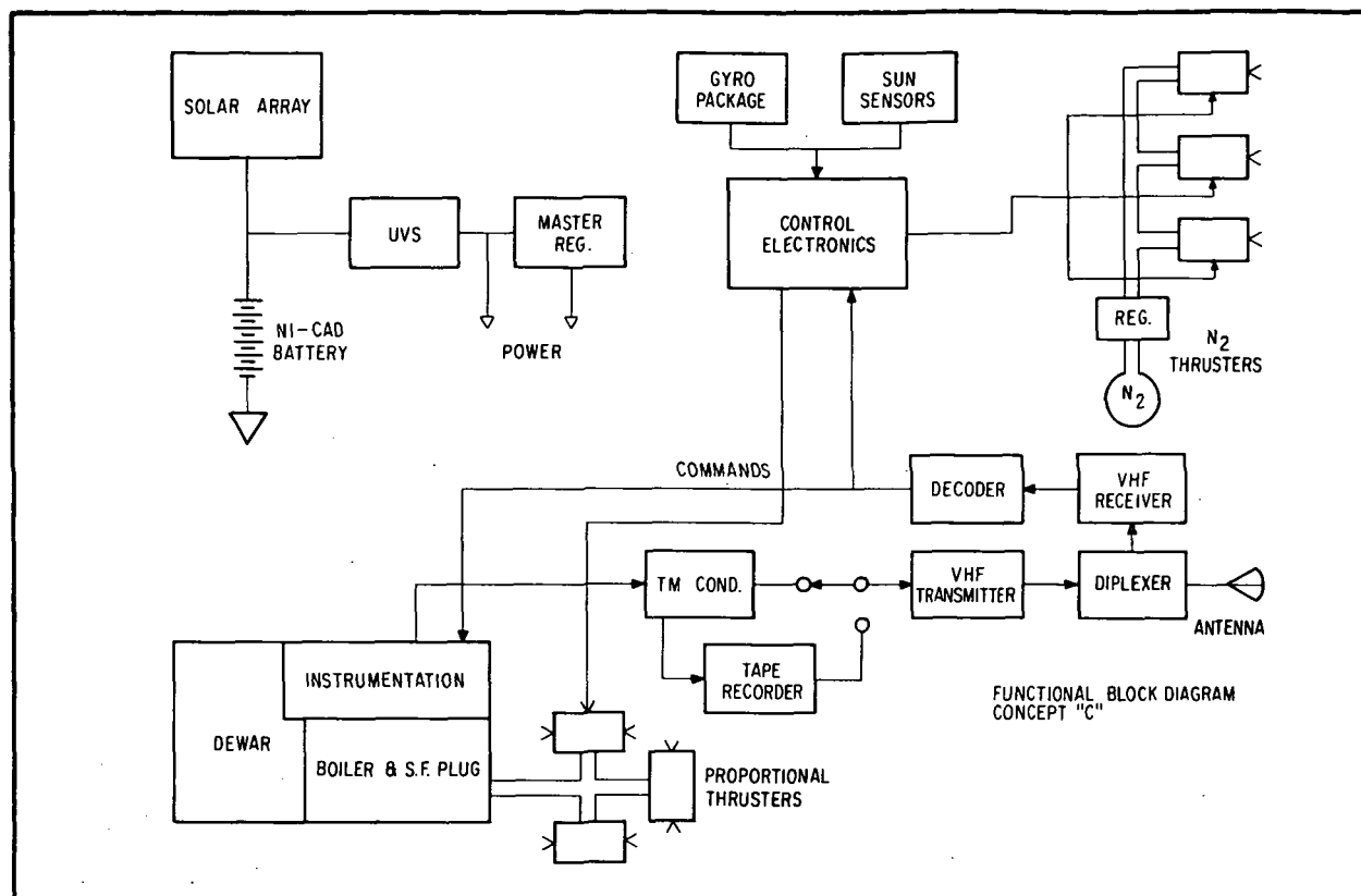
Fig. 4-5 Concept C: Functional Block Diagram
