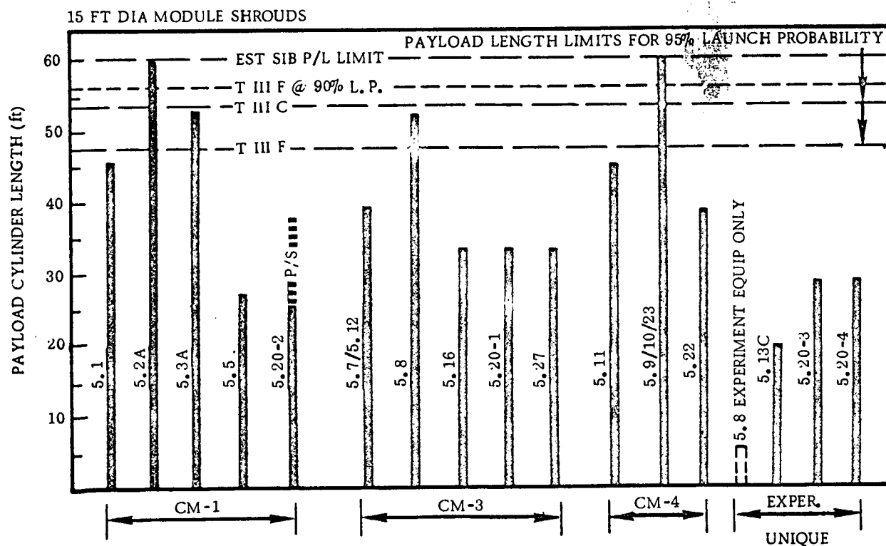
Figure 3-6. Expendable L/V Payload Sensitivity
