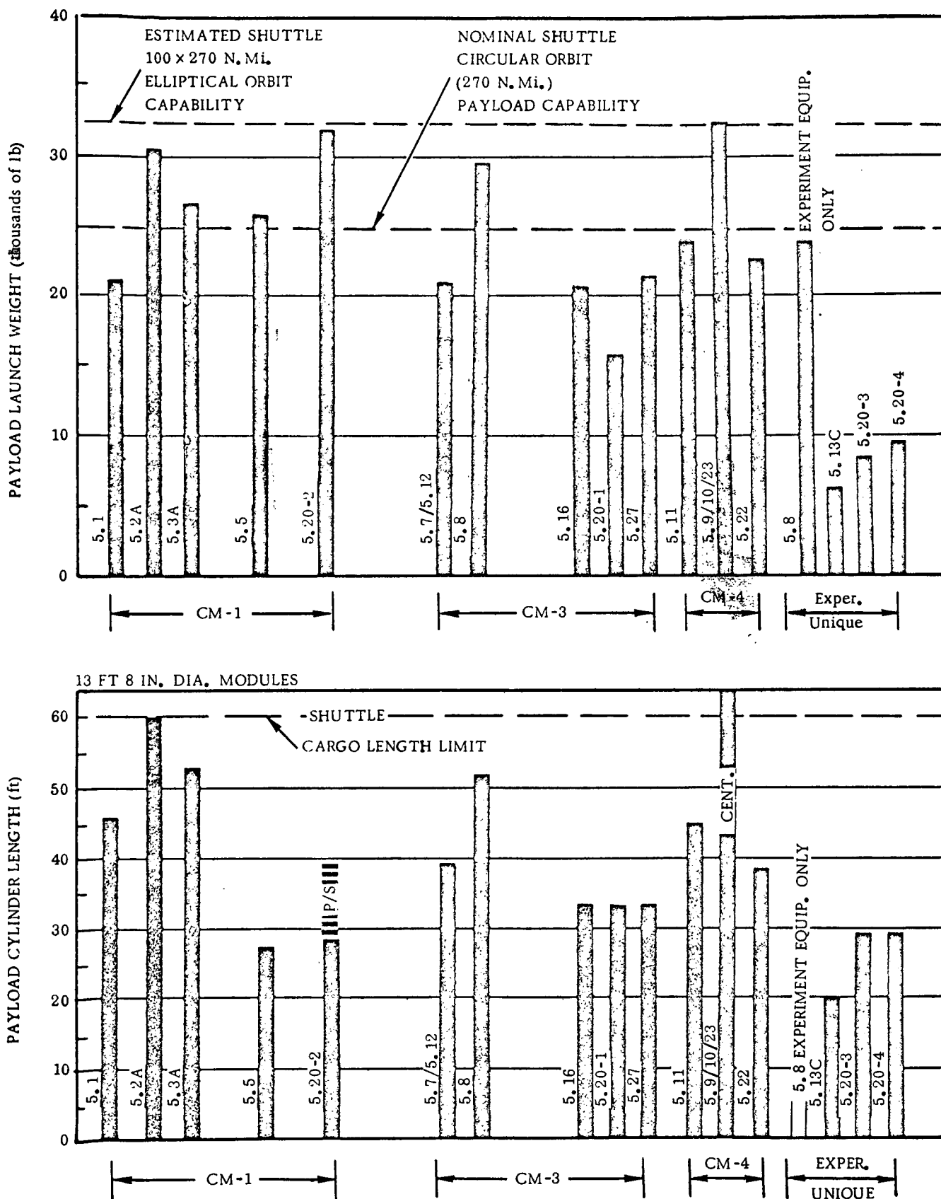
Figure 3-5. Shuttle Payload Sensitivity
