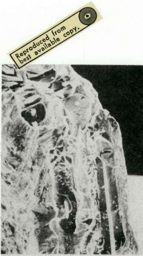
Figure 23. - Details of axial fracture surface containing split filament, 3.9 mils filament diameter.
