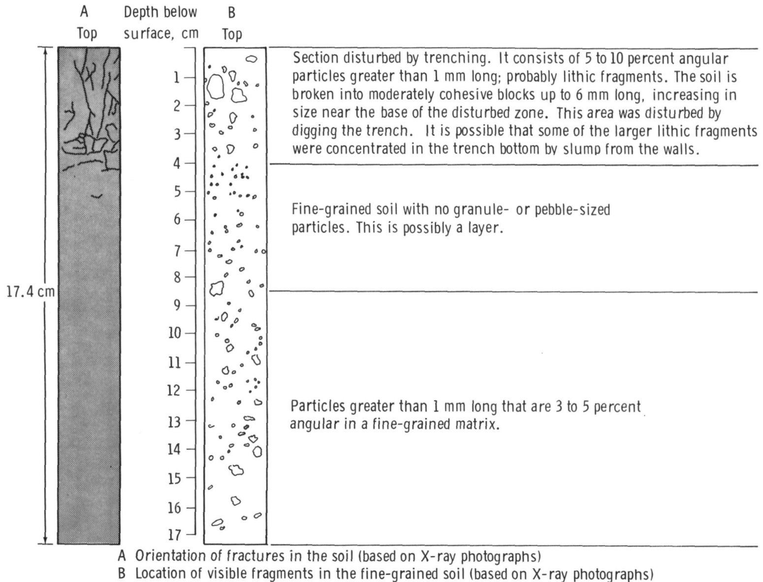
Figure 4. - Core sample 12027, showing the location and orientation of all soil particles larger than 1 millimeter. Diagram is based on X-ray photograph of unopened core.
