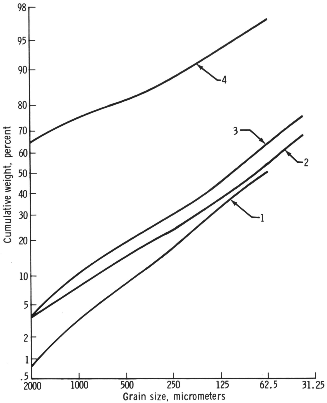
Figure 3.- Grain-size distribution of soil samples from (1) top, (2) middle, and (3) bottom of core sample 12026 and (4) from the coarse layer of the double-drive tube (core sample 12028, daughter sample 16).
