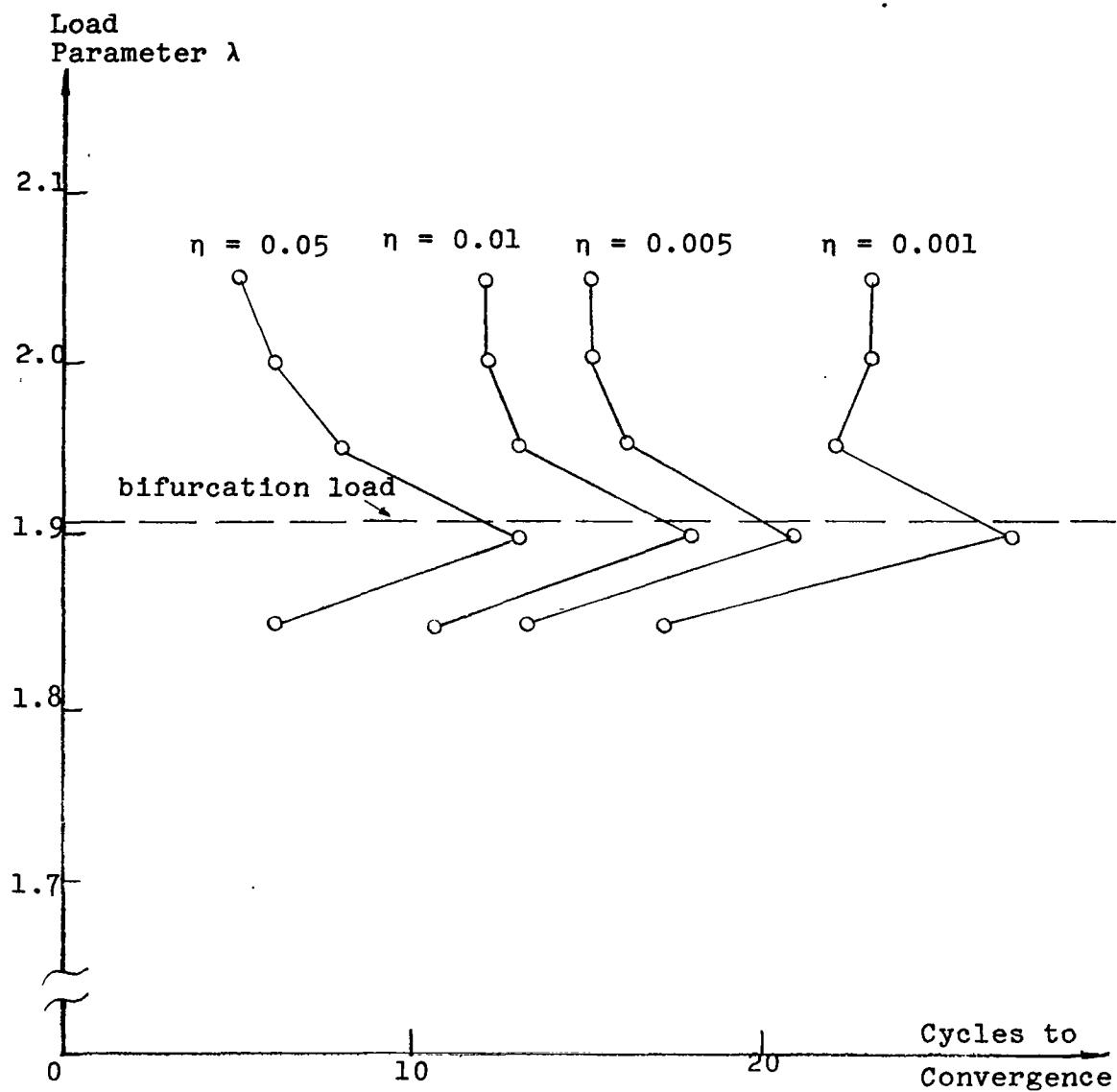
FIGURE A-2. NUMBER OF ITERATIONS FOR CONVERGENCE VS. LOAD LEVEL FOR VARIOUS CONVERGENCE CRITERIA ( \eta )
