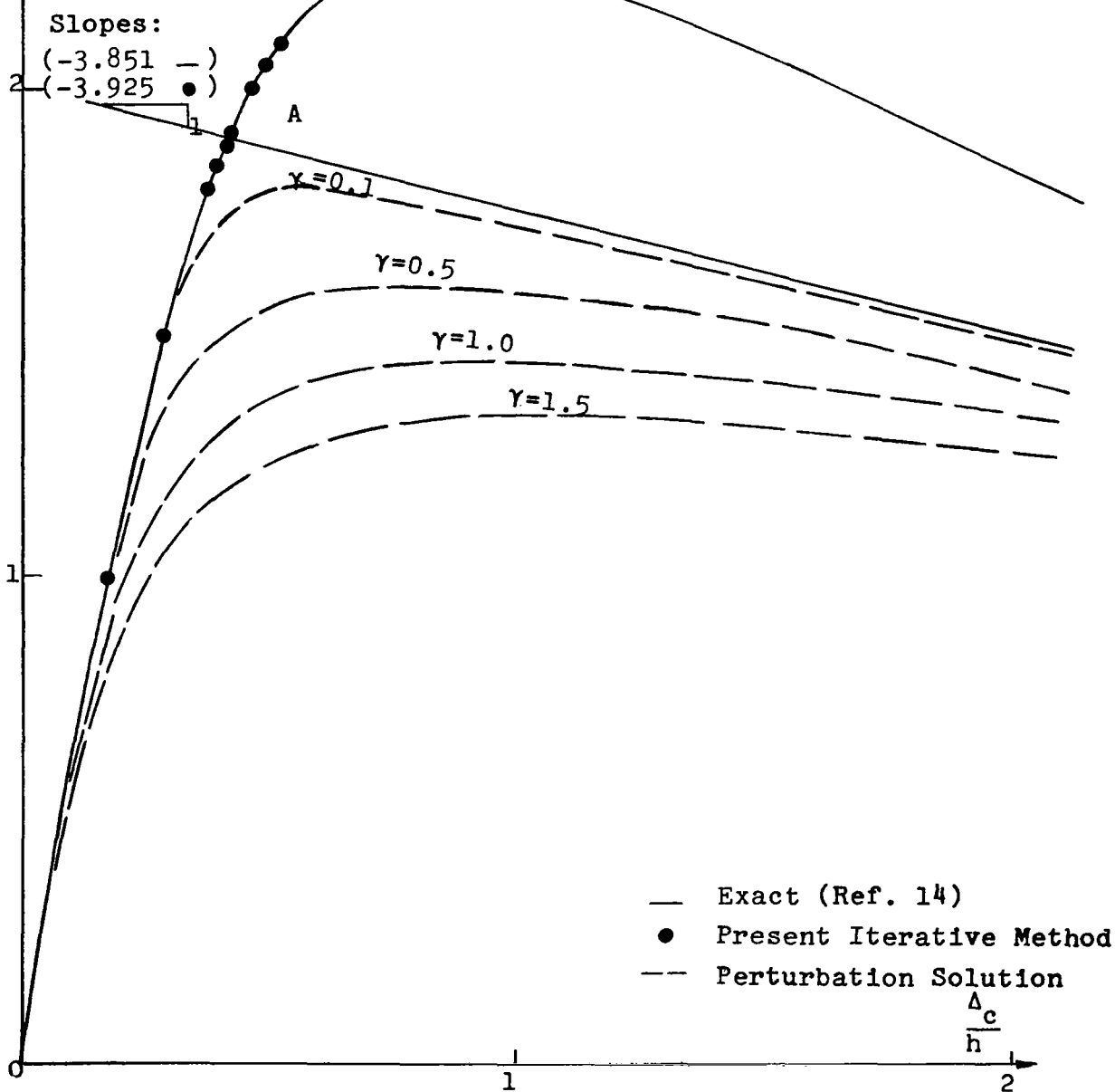
FIGURE 5. LOAD VS. CENTRAL DEFLECTION FOR PRE-BUCKLING, POST-BUCKLING AND IMPERFECT BEHAVIORS
