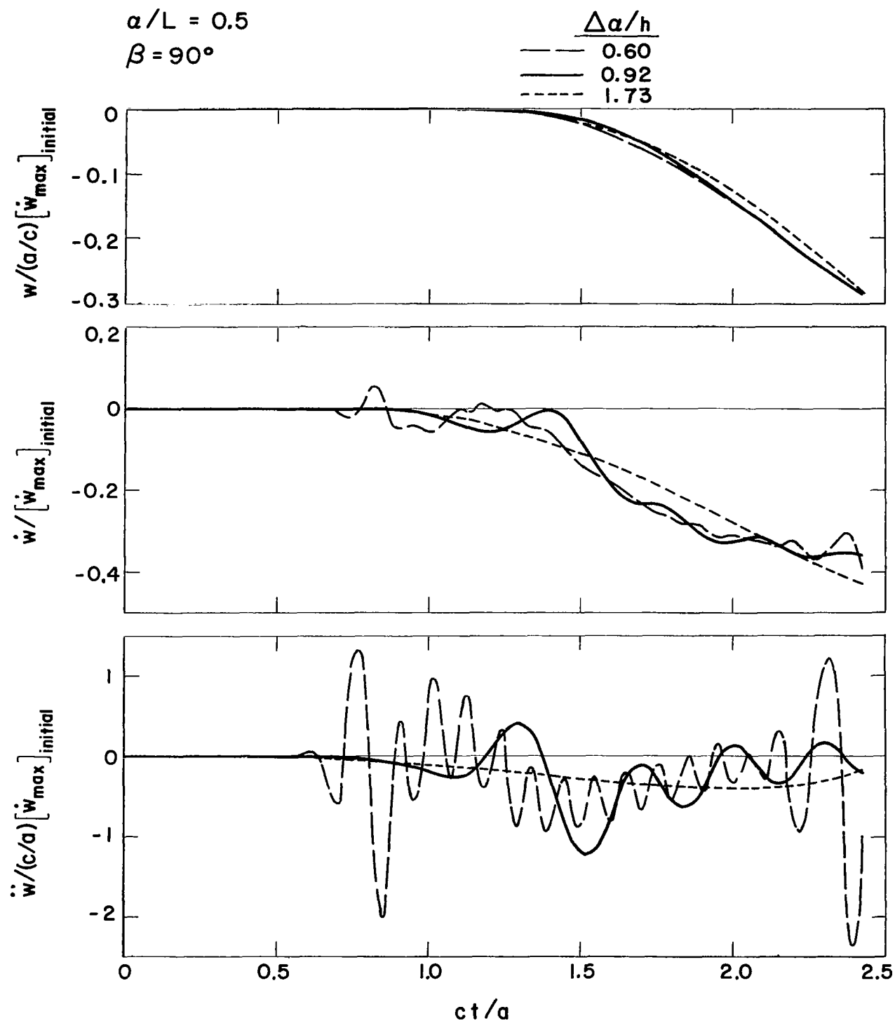
Figure 35. Kinematic Response Histories for Example 13 (Cosine Impulse)
