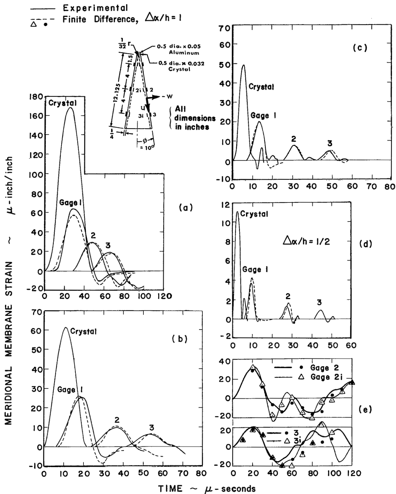
Figure 54. Strain Response Histories for Example 17
