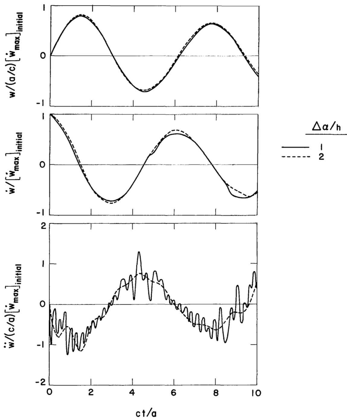
Figure 22. Kinematic Response Histories for Example 10 ( \alpha_w = 0.8a )
