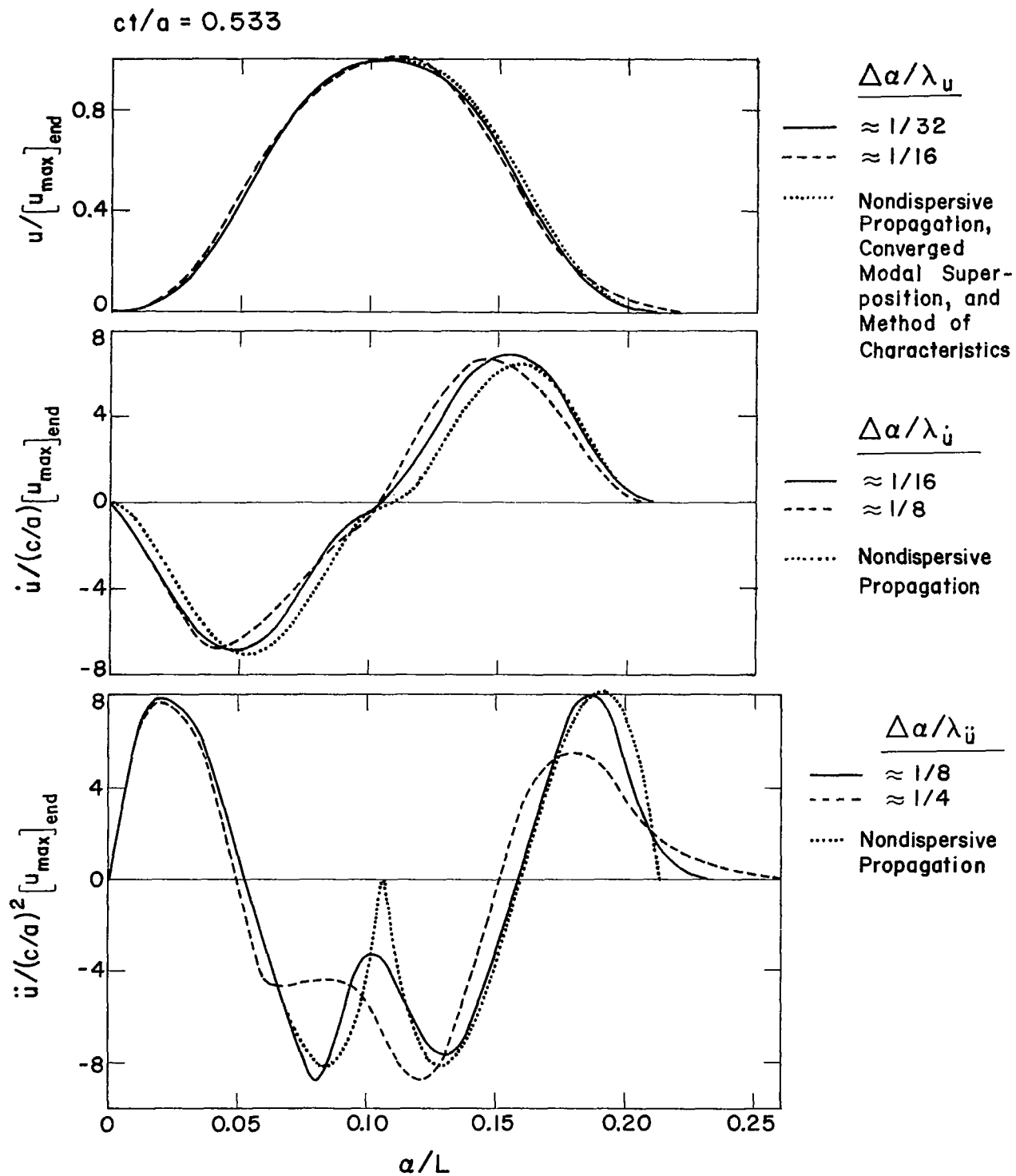
Figure 2. Kinematic Response Snapshots for Example 1
