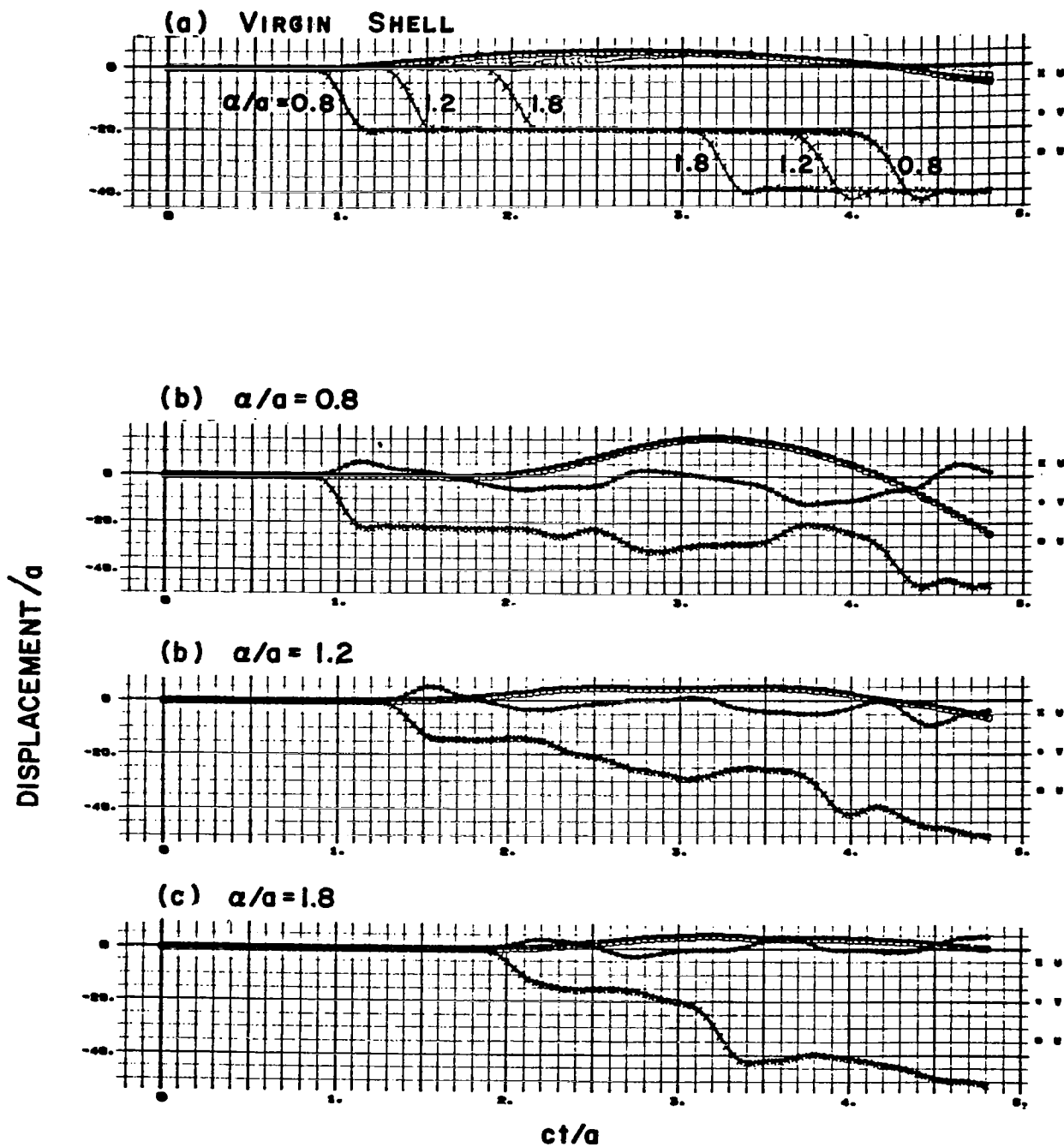
Figure 3. Virgin Shell and ( \beta = \pi/12 ) Cut Shell Displacement Histories
