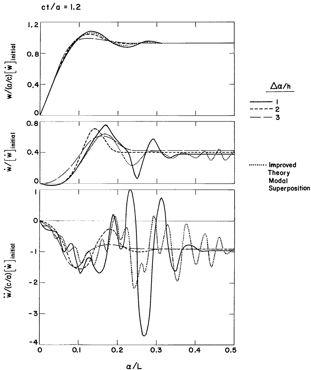
Figure 31. Kinematic Response Snapshots for Example 12
