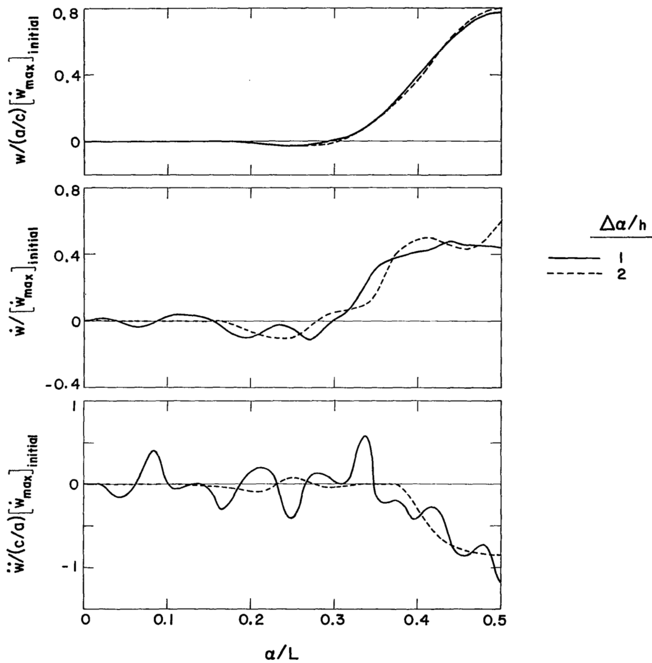
Figure 23. Kinematic Response Snapshots for Example 10 ( \alpha_w = 0.8a )
