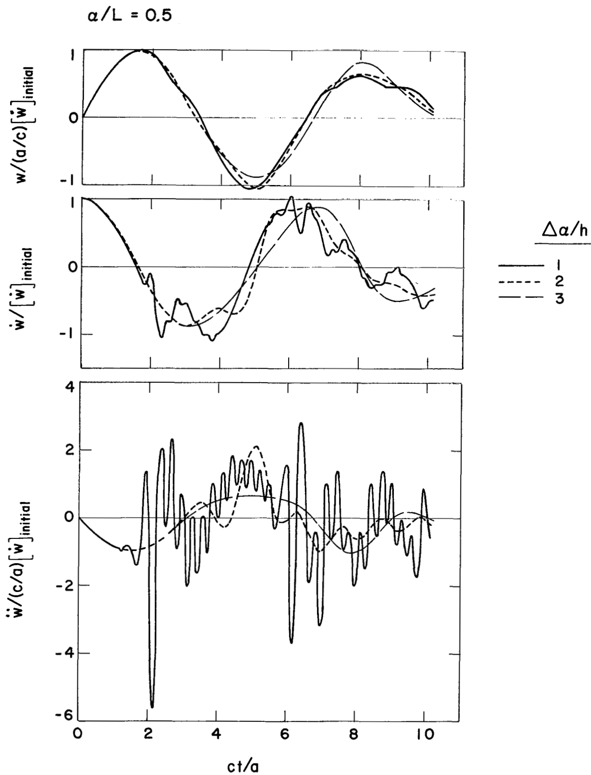
Figure 30. Kinematic Response Histories for Example 12
