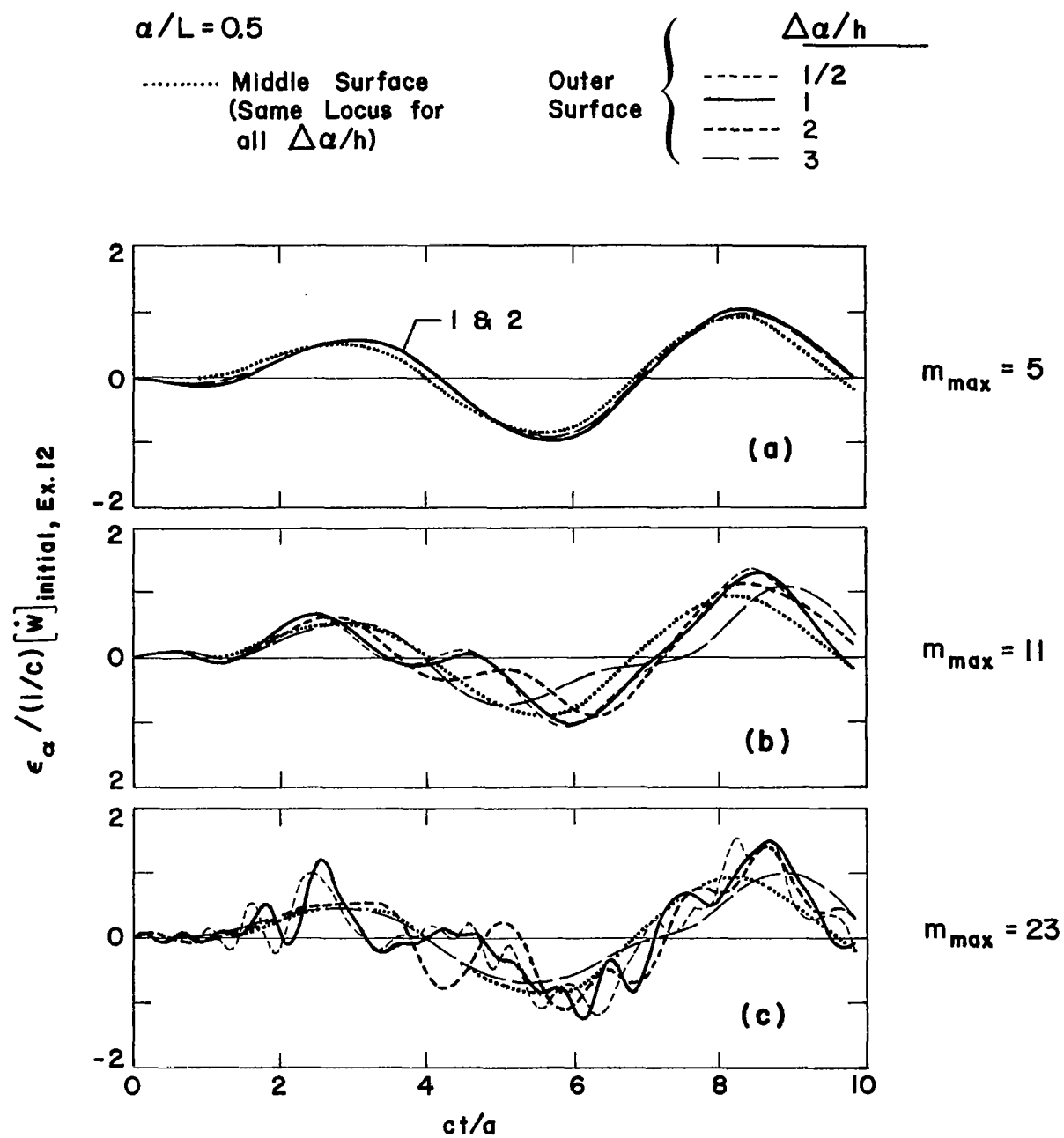
Figure 61. Strain Response Histories for Example 15
