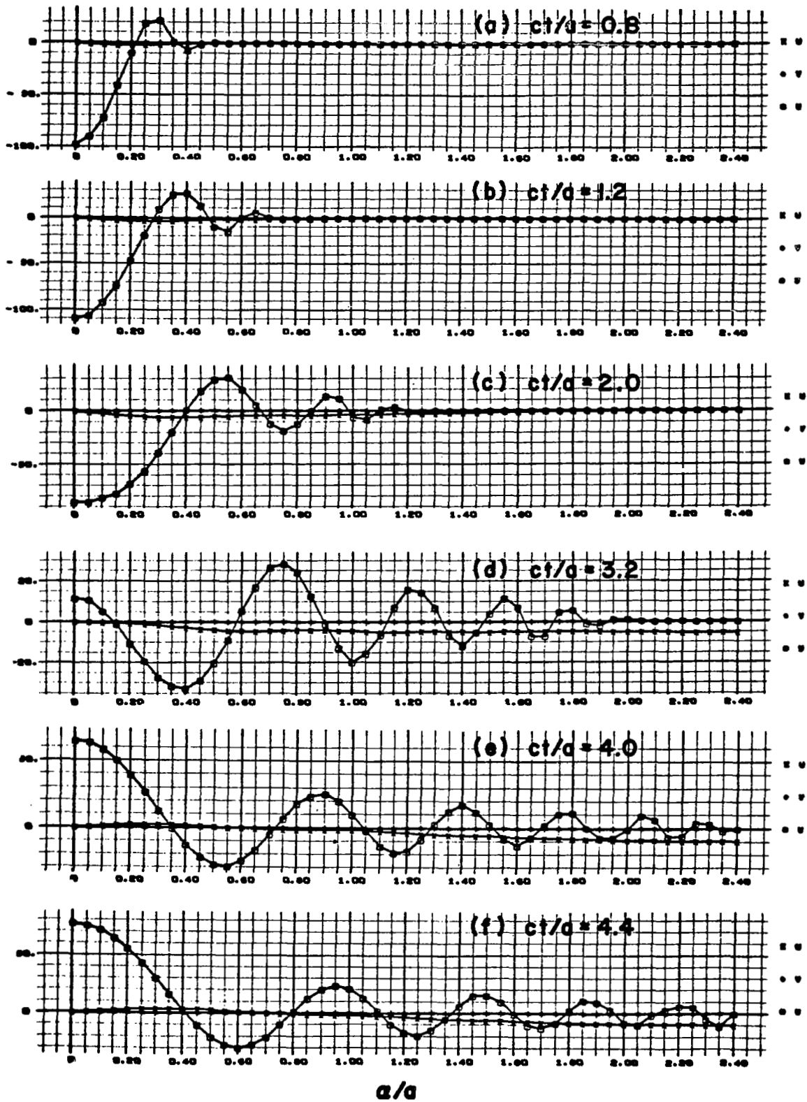
Figure 20. Virgin Shell Displacement Snapshots
