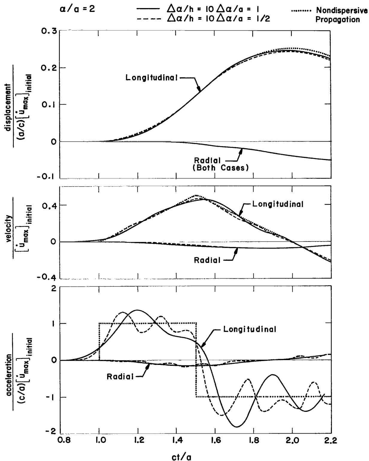
Figure 13. Kinematic Response Histories for Example 6
