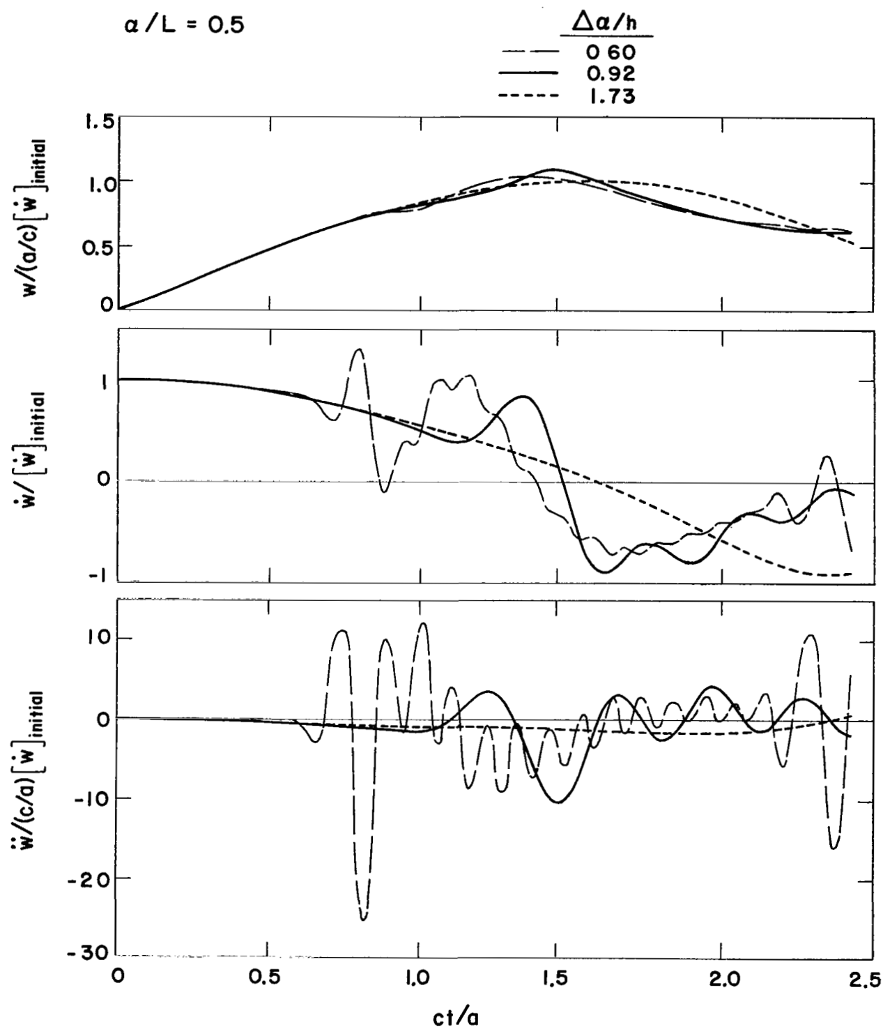
Figure 33. Kinematic Response Histories for Example 13 (Uniform Impulse)
