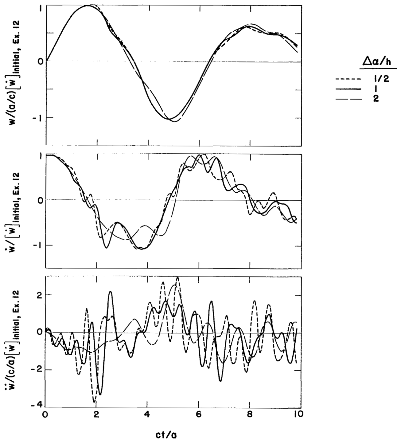
Figure 45. Kinematic Response Histories for Example 15 ( m_{\max} = 23 )
