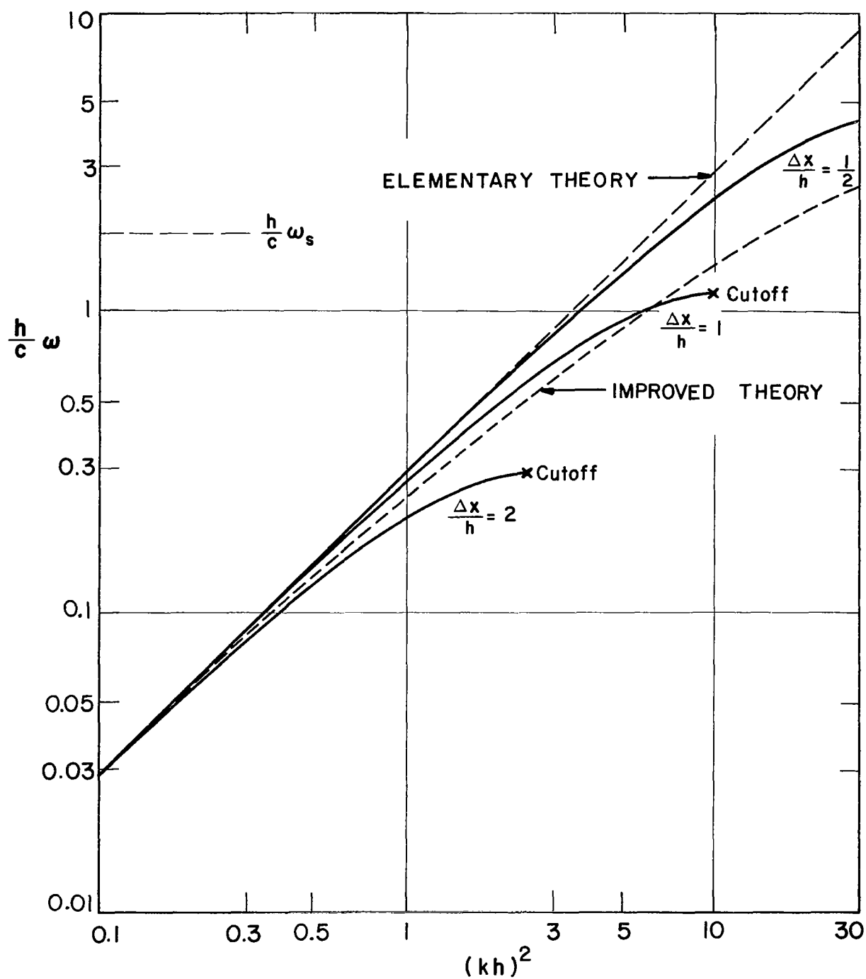
Figure 4. Frequency Curves for Continuous and Finite Difference Plates (k_x = k, k_y = 0)
