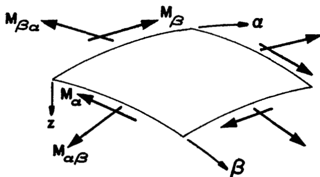
MOMENT RESULTANTS
