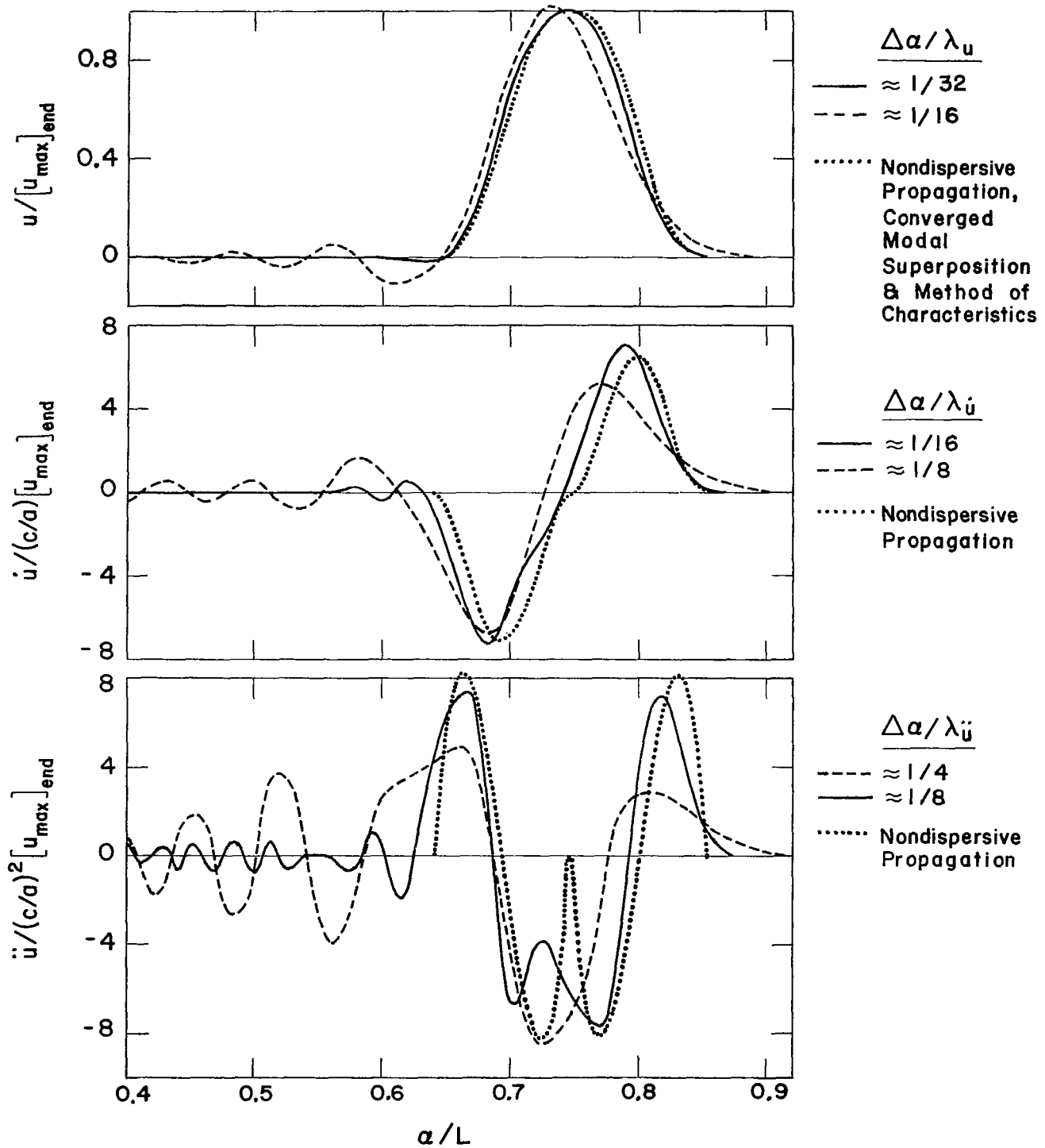
Figure 3. Kinematic Response Snapshots for Example 1 2-23
