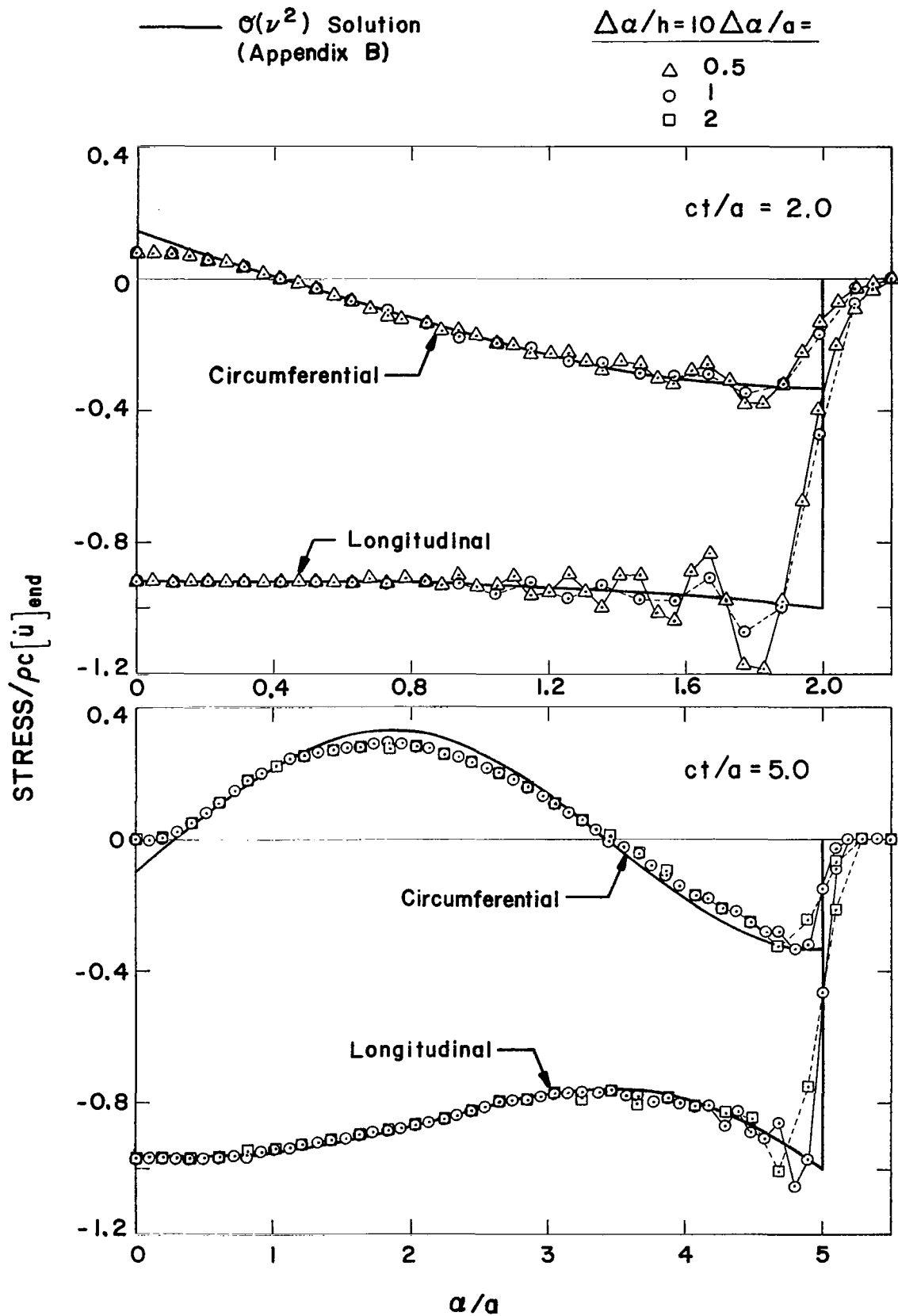
Figure 49. Stress Response Snapshots for Example 7
