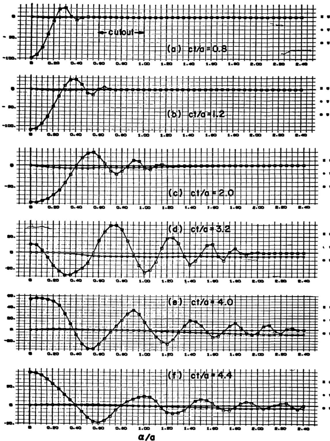
Figure 23. Cut Shell Displacement Snapshots along the Line \beta = \pi/4
