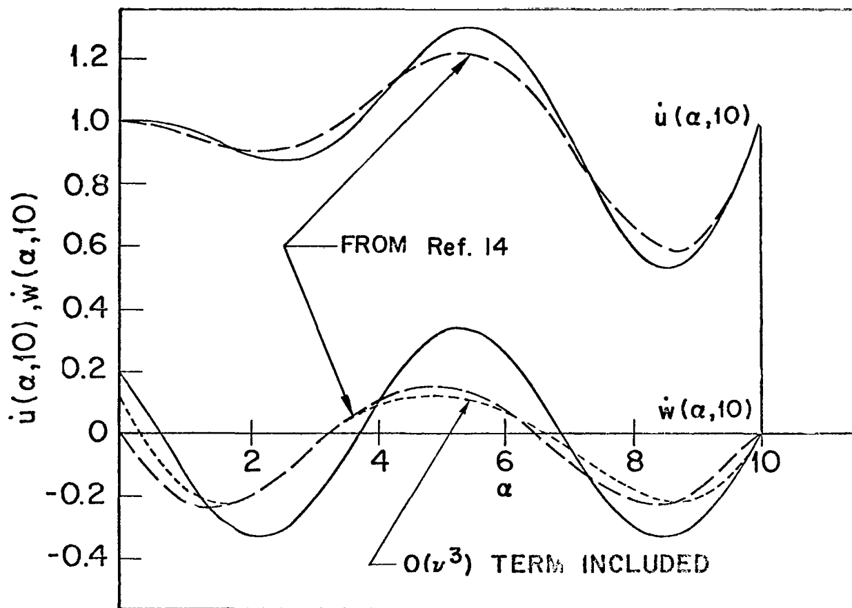
Figure 2. Velocity Snapshot at \tau = 10 (Step-Velocity Excitation)
