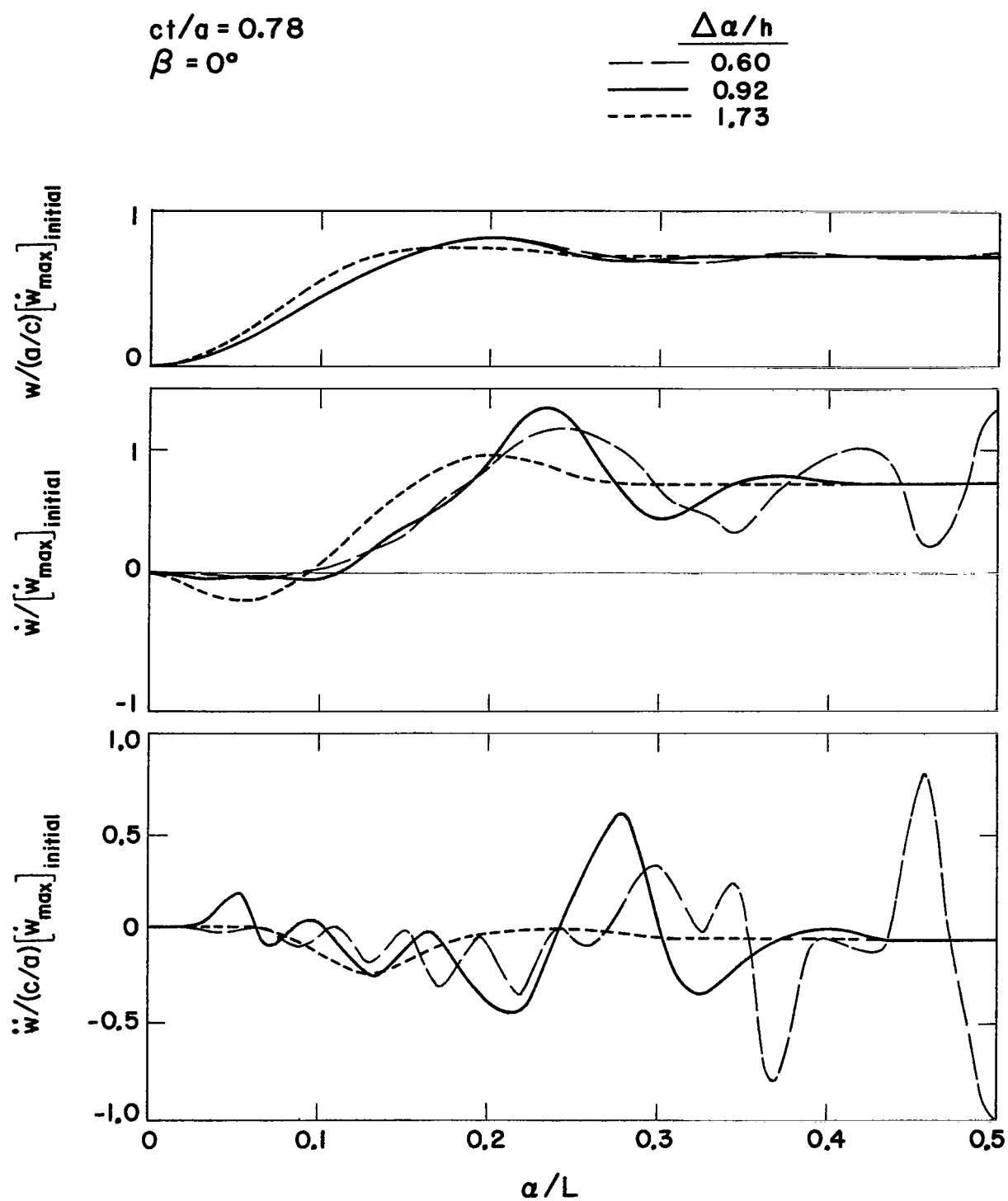
Figure 38. Kinematic Response Snapshots for Example 13 (Cosine Impulse)
