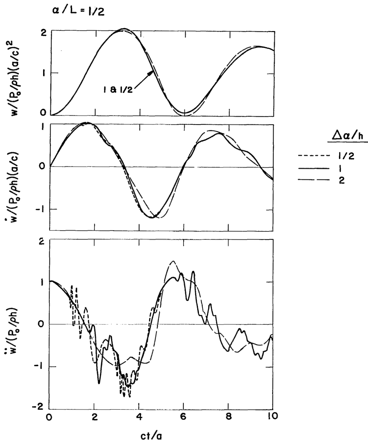
Figure 19. Kinematic Response Histories for Example 9
