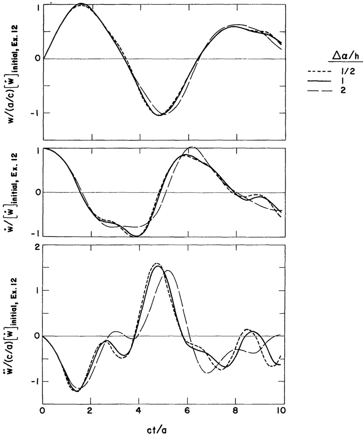
Figure 44. Kinematic Response Histories for Example 15 ( m_{\max} = 11 )
