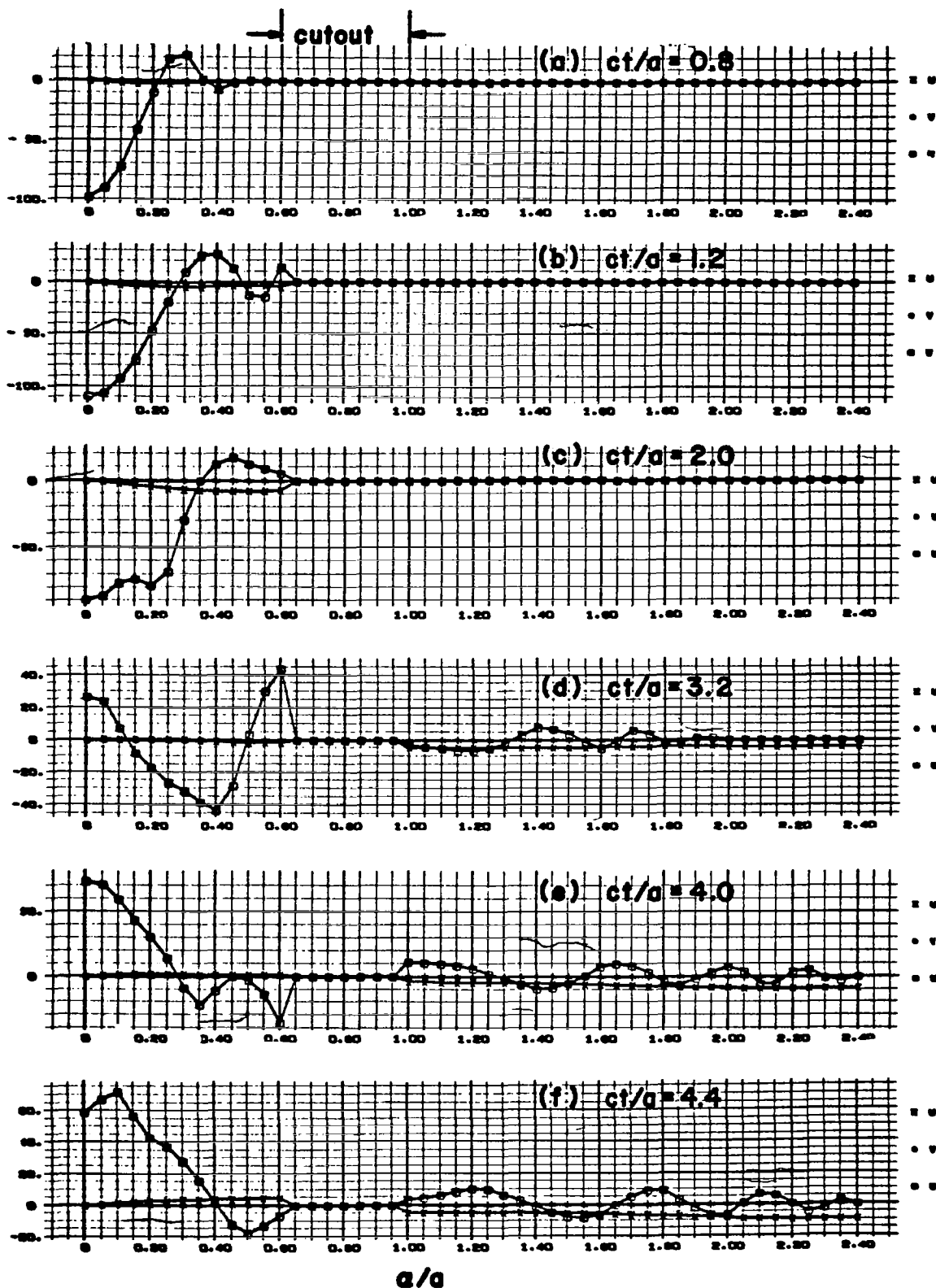
Figure 21. Cut Shell Displacement Snapshots along the Line \beta = 0
