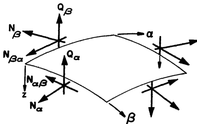
FORCE RESULTANTS
