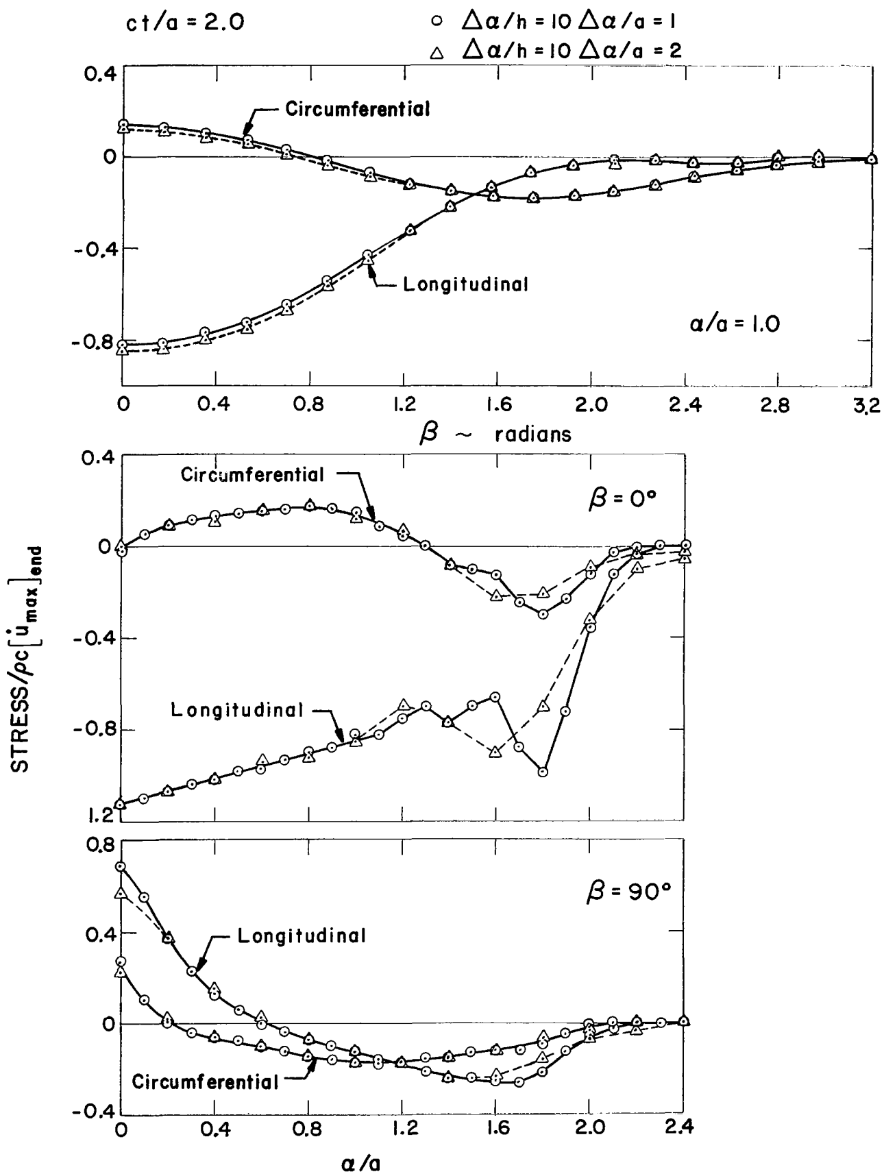
Figure 50. Stress Response Snapshots for Example 8
