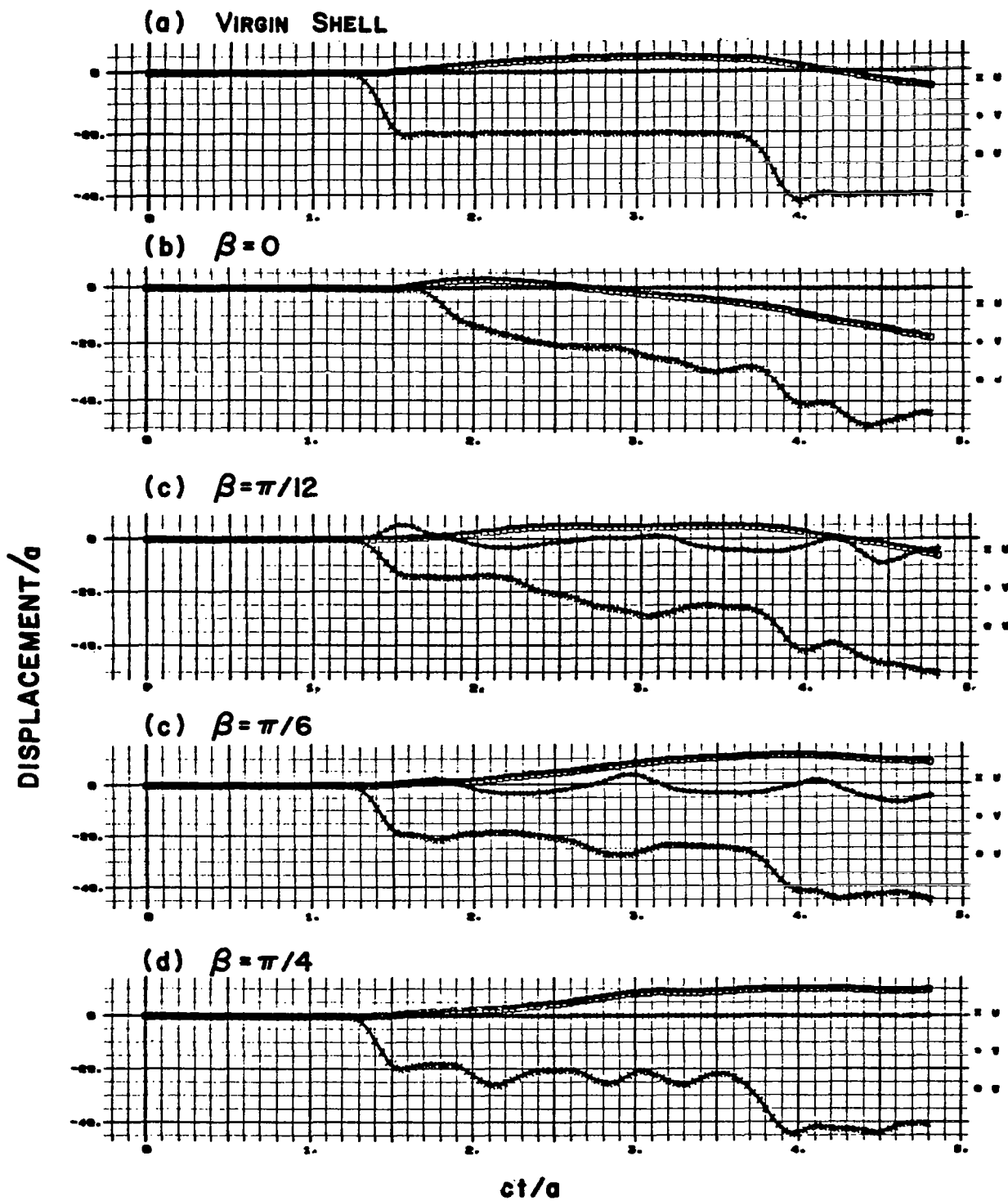
Figure 4. Virgin Shell and Cut Shell Displacement Histories at \alpha/a = 1.2
