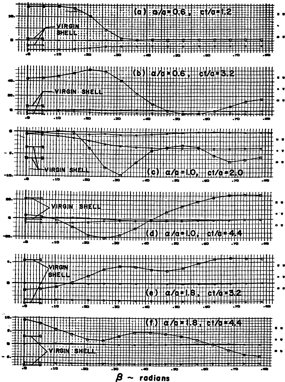
Figure 24. Circumferential Snapshots of Cut Shell Displacement Response
