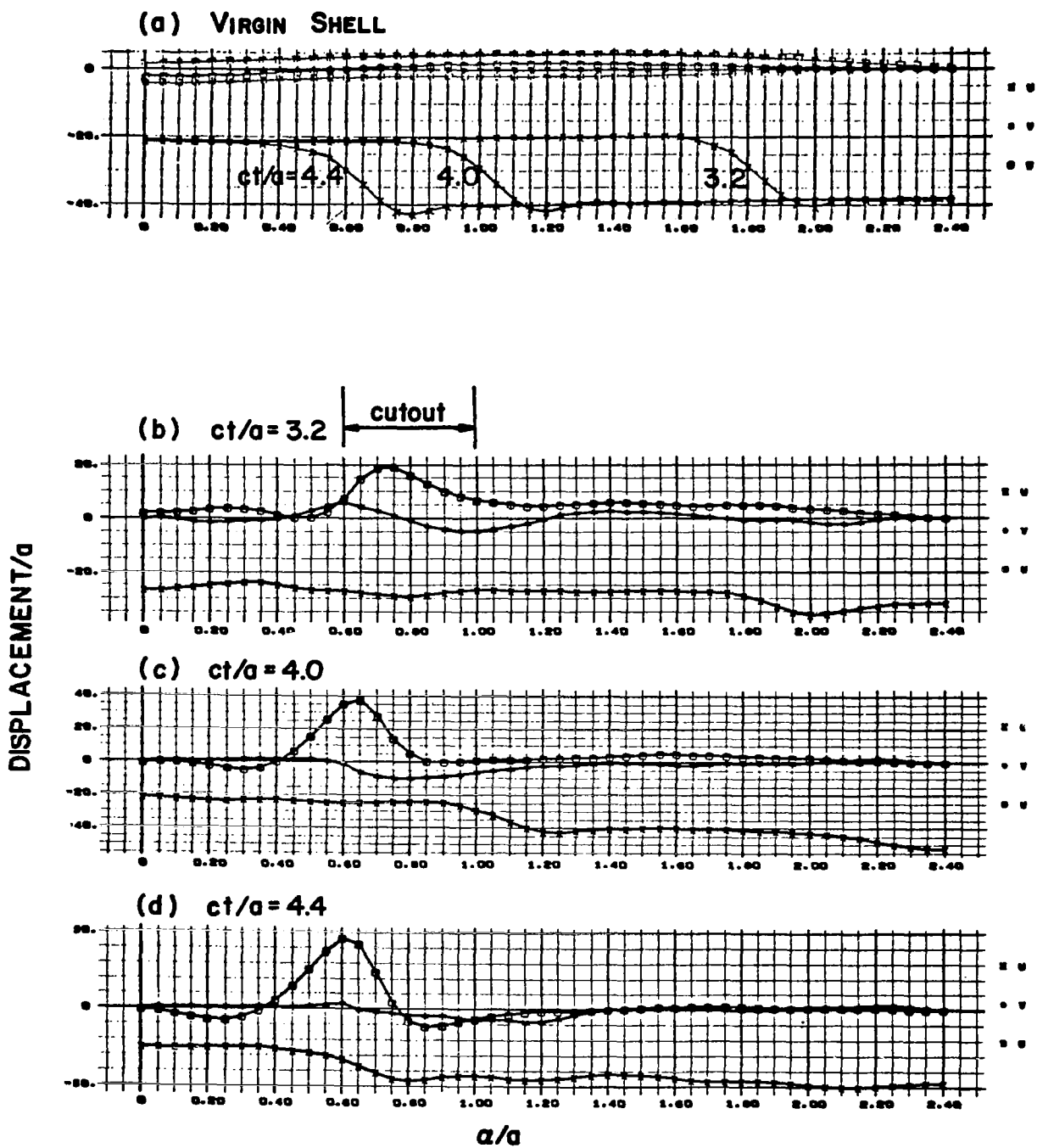
Figure 11. Virgin Shell and ( \beta = \pi/12 ) Cut Shell Displacement Snapshots
