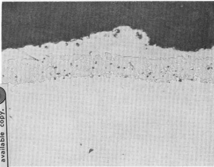
Poor Edge Coverage on TD-Ni Specimen 32
