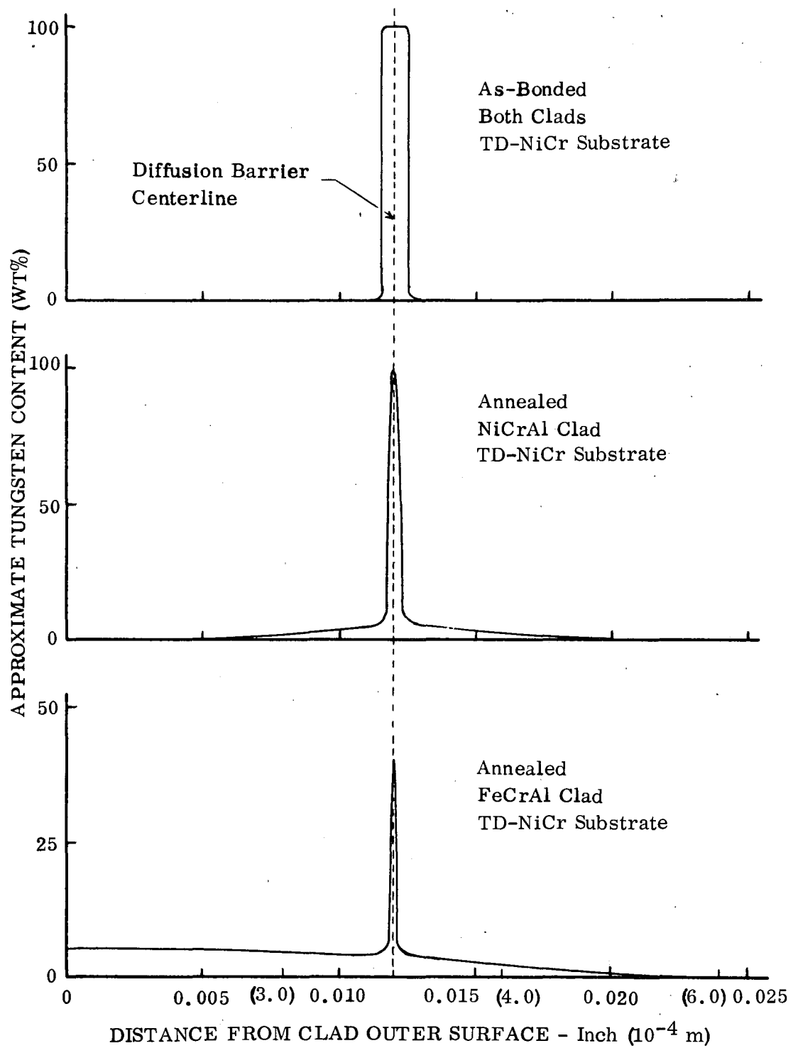
FIGURE 20. INTERDIFFUSION OF FOIL TUNGSTEN BARRIER WITH CLAD AND SUBSTRATE DURING ANNEALING (2300° F for 100 Hours in Argon)
