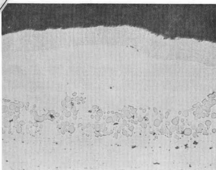
FIGURE 31. ALUMINIZED NC-15 MODIFIER ON W-11 COATED TD-Ni AND TD-NiCr
