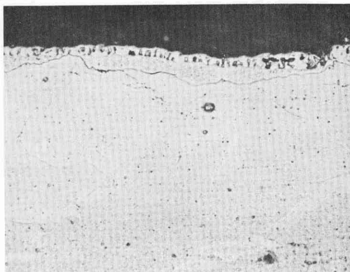
FIGURE 4. Cr-C DIFFUSION BARRIER ON TD-Ni AND TD-NiCr; Solar H2-56B Pack Chromized Plus Gas Carburized in 94\text{Ar}-6\text{CH}_4 for 1 Hour at 1900^\circ\text{F}
