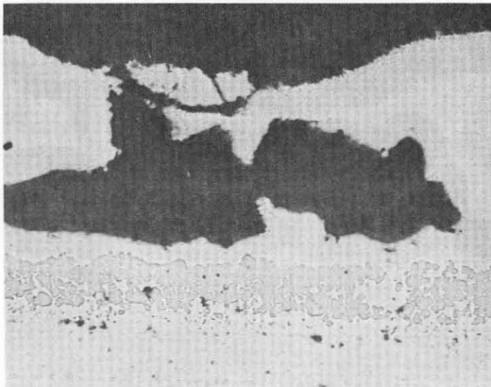
FIGURE 32. COATING DEFECTS ON TD-Ni AND TD-NiCr TENSILE SPECIMENS
