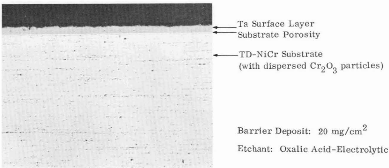
FIGURE 3. Ta DIFFUSION BARRIER ON TD-Ni AND TD-NiCr; Applied by Fused Salt Plating
