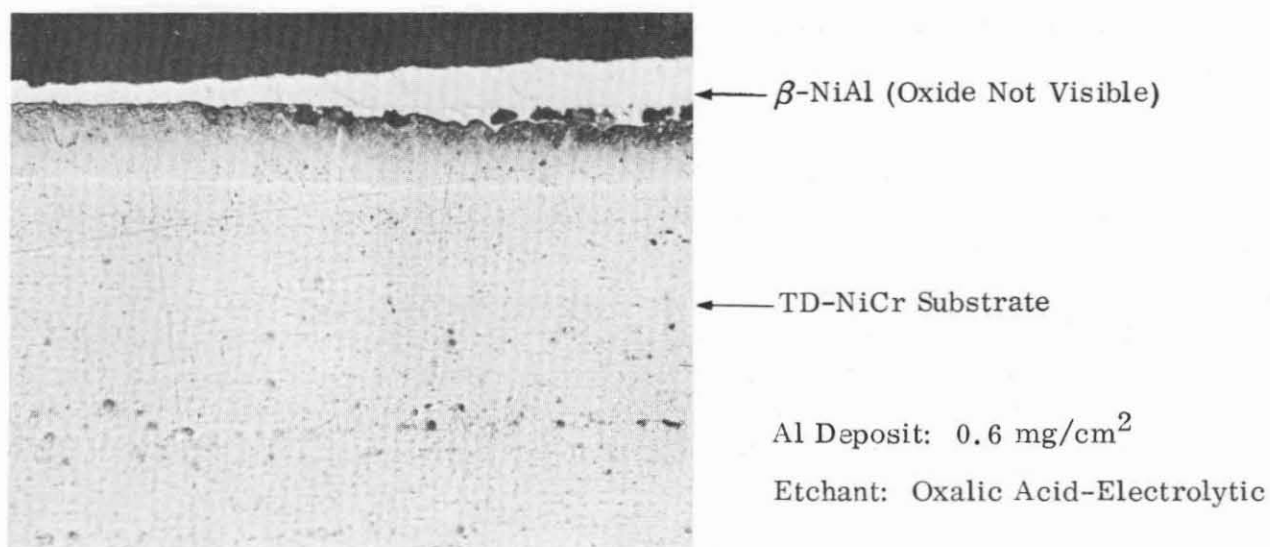
FIGURE 6. CONTINUOUS \text{Al}_2\text{O}_3 DIFFUSION BARRIER ON TD-Ni AND TD-NiCr; Solar S8100 Fusion Slurry Aluminized Plus Controlled Oxidation in 10^{-4} Torr Air at 1900^\circ \text{F} for 1 Hour
