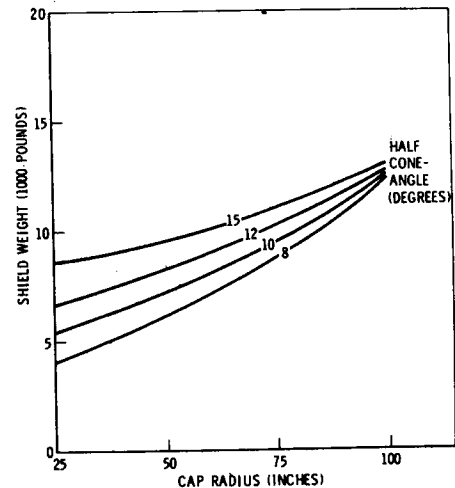
Figure 5. Shield Weight Variation for Single Tank Conical Configuration
