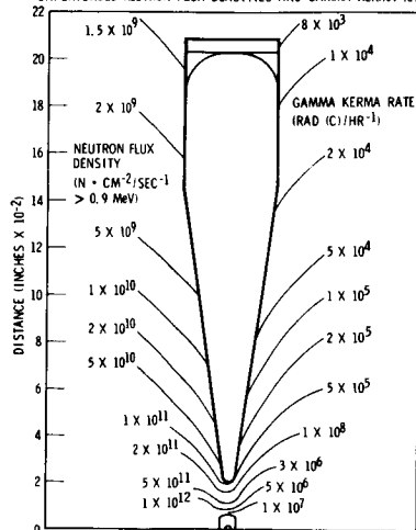
Figure 15. RNS Baseline Configuration - Iso Contours
