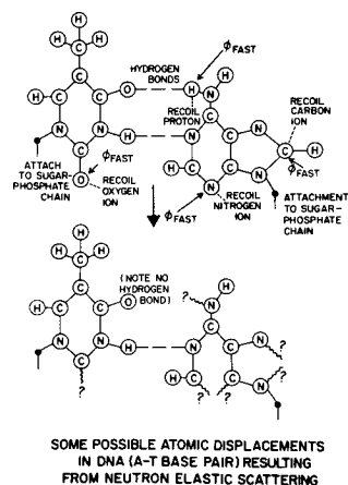
Fig. 4: Fast neutrons (fast) interacting by elastic scatter with and recoiling from hydrogen, carbon, oxygen and nitrogen atoms, creating atomic ions in the DNA bases. The question marks indicate uncertainties regarding the ultimate biochemical reactions. The most probable elastic scatter is with the hydrogen atom, producing recoil protons.
