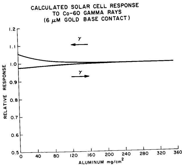
AFCLR PHOTO 121-51 FIGURE 12. - Calculated Response for a Thin Gold Film Near the Base Contact.
