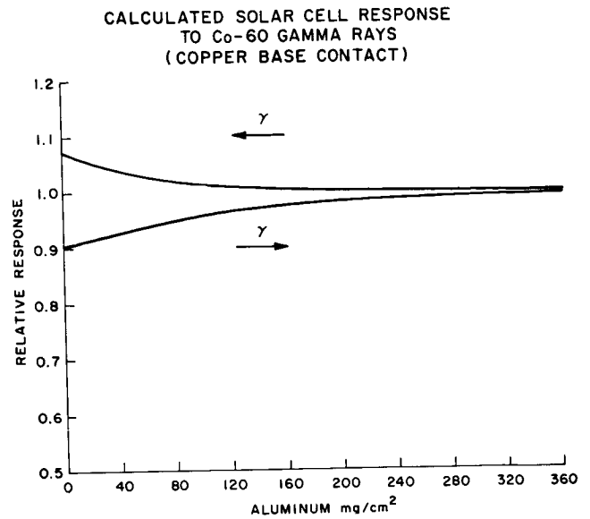
AFCLR PHOTO 121-48 FIGURE 13. - Calculated Response for a Cu-Al Interface Near the Base.
