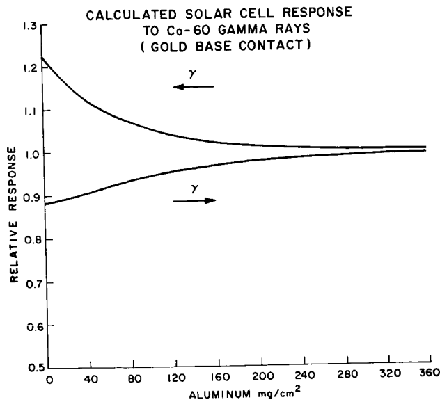
AFCLR PHOTO 121-55 FIGURE 11. - Calculated Response with the Au-Al Interface Near the Base Contact. The thickness of aluminum indicated lies between the gold and the base. Arrows indicate the beam direction relative to the cell face.
