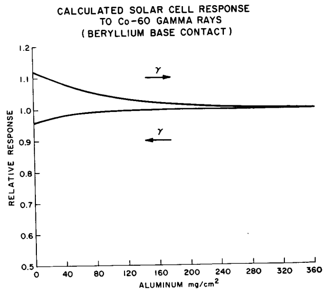
AFCLR PHOTO 12 FIGURE 14. - Calculated Response with a Be-Al Interface Near the Base Contact.
