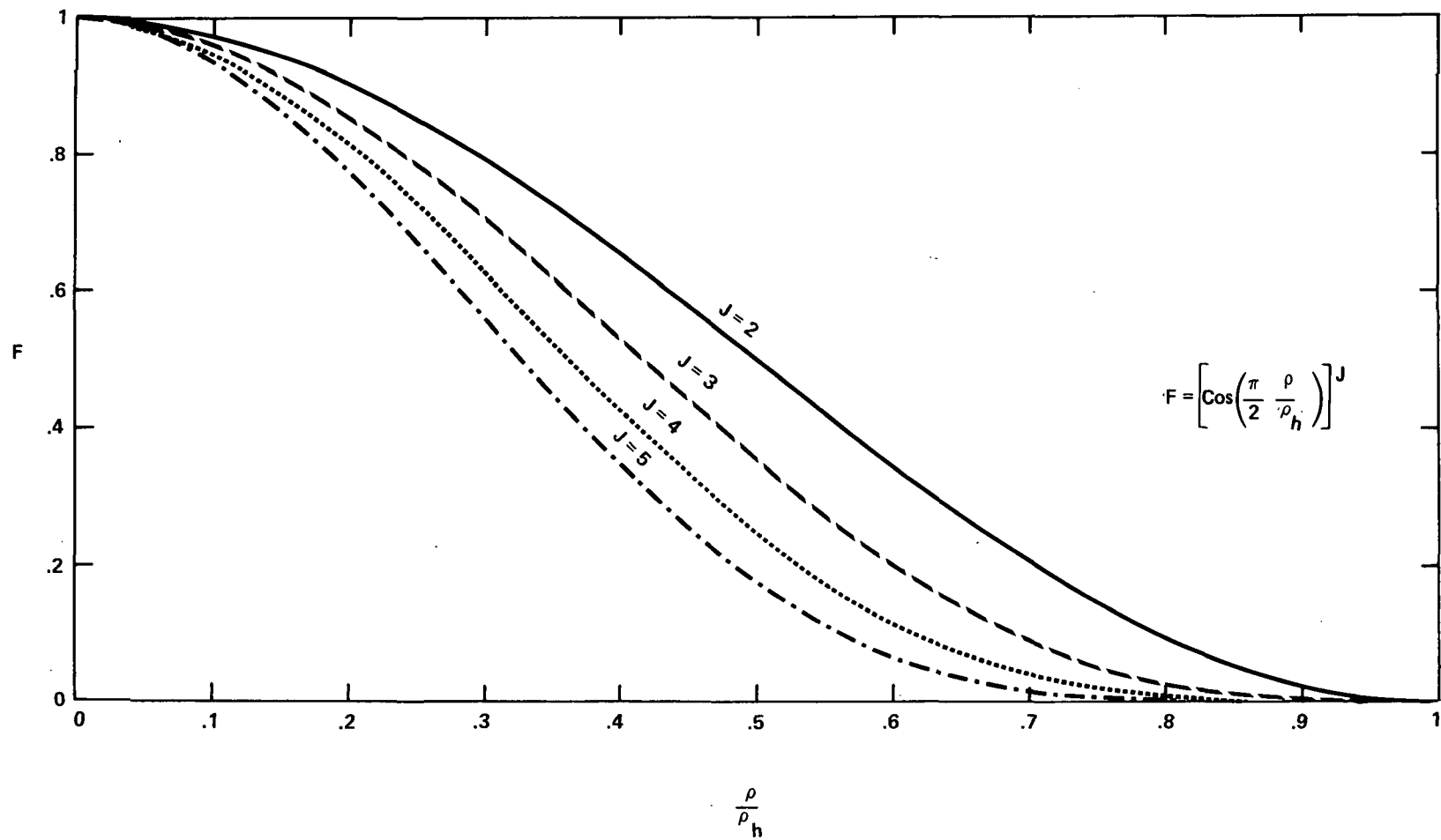
FIGURE 9 - INHOMOGENEOUS SEA WATER DROPLETS PROFILES
