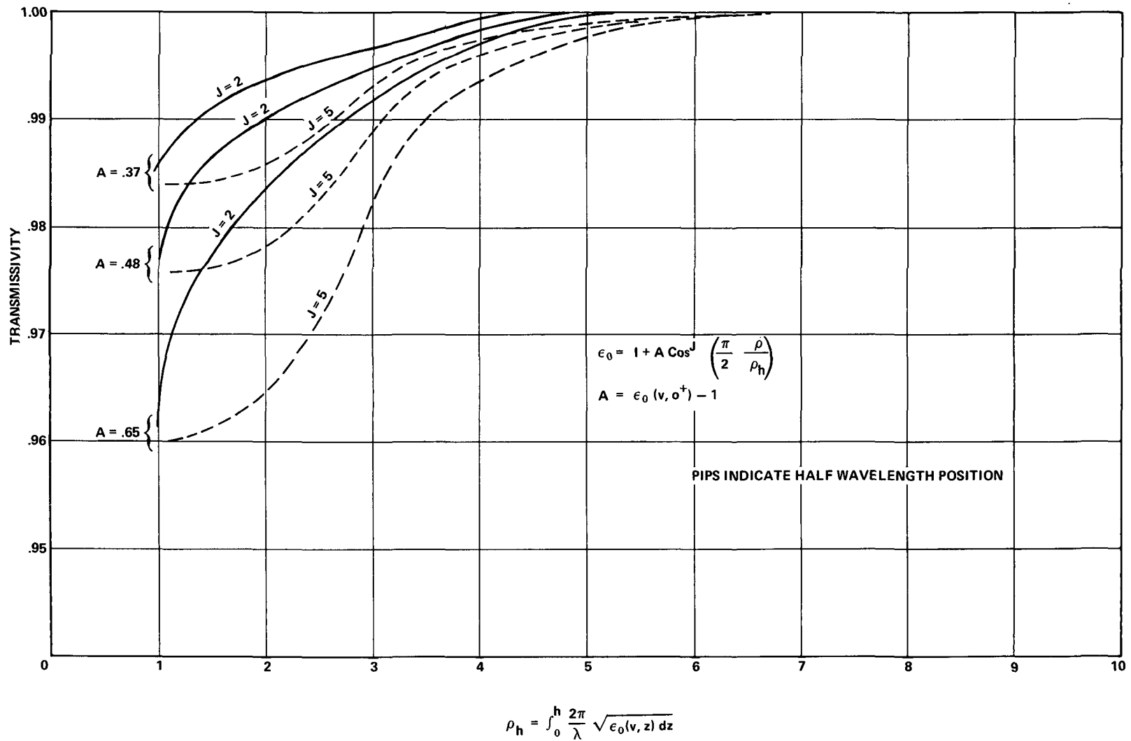
FIGURE 10 - TRANSMISSIVITY (FOR NORMAL INCIDENCE) OF INHOMOGENEOUS LOSSLESS SEA WATER DROPLETS PROFILES
