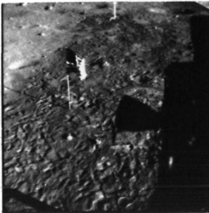
AS11-39-5819
