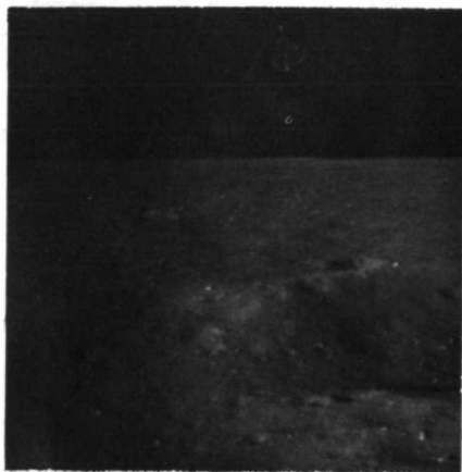
AS11-39-5743
