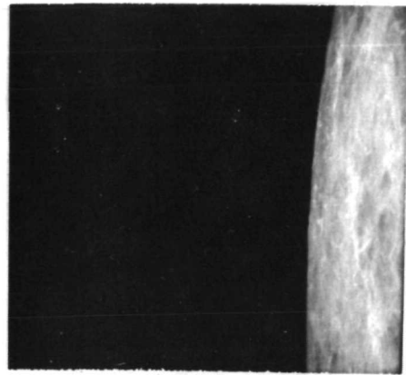
AS11-41-5990
