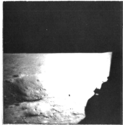
AS11-39-5756
