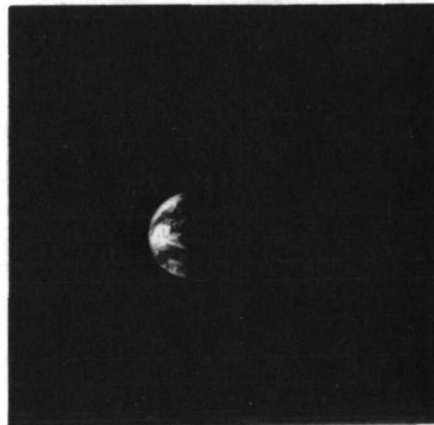
AS11-38-5697
