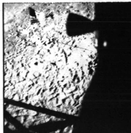
AS11-39-5802
