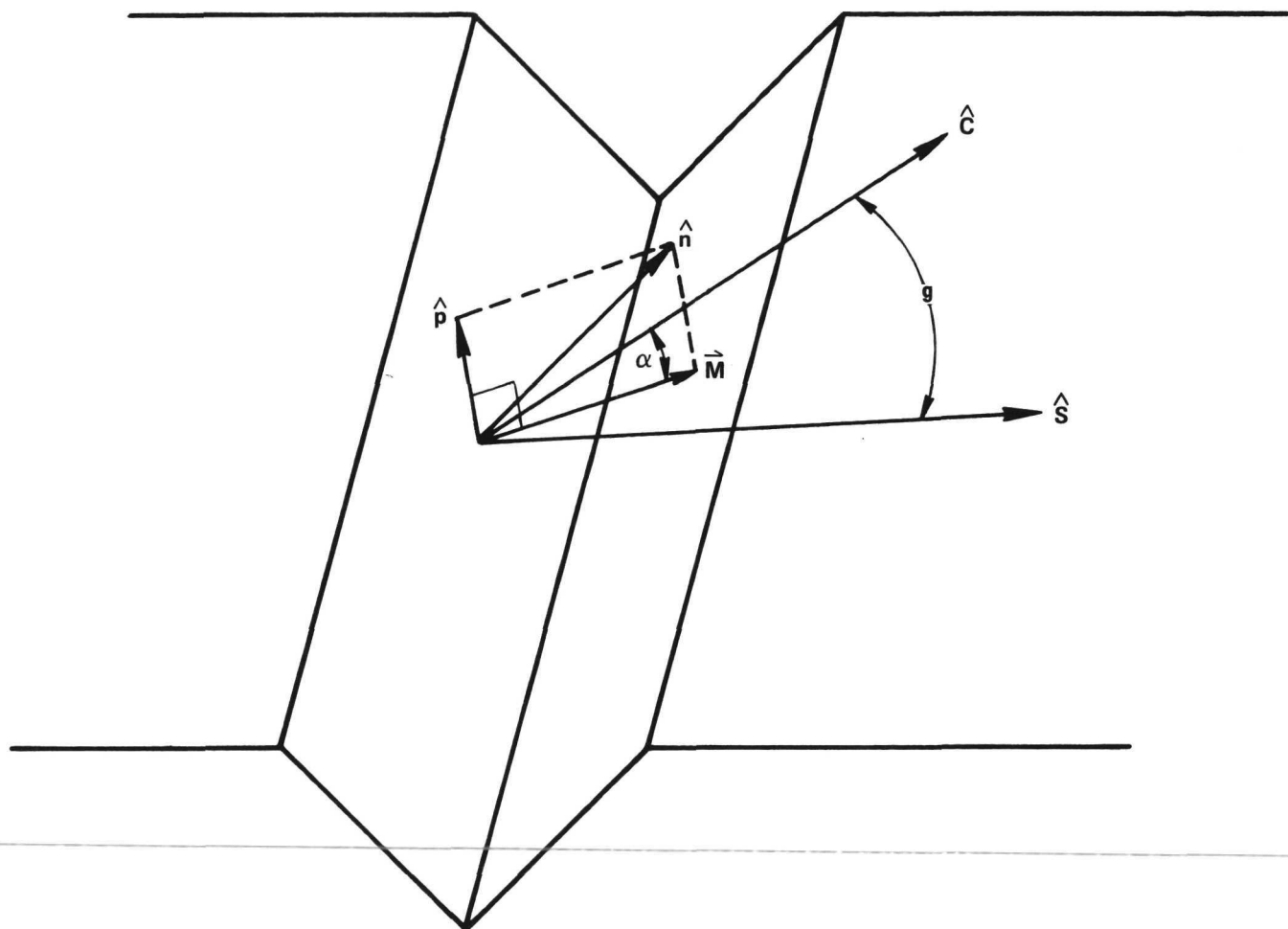
FIGURE AI-1 - GEOMETRY OF PHASE PLANE
