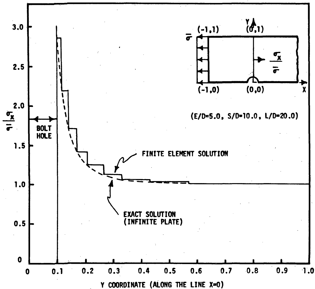
FIGURE 3a: ISOTROPIC BOLT BEARING VERIFICATION: \sigma_x / \bar{\sigma} vs Y
