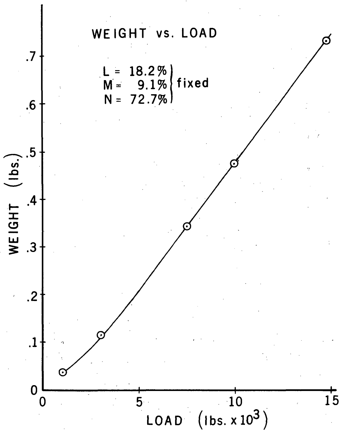
FIGURE 1: WEIGHT VS. LOAD FOR FIXED ORIENTATIONS
