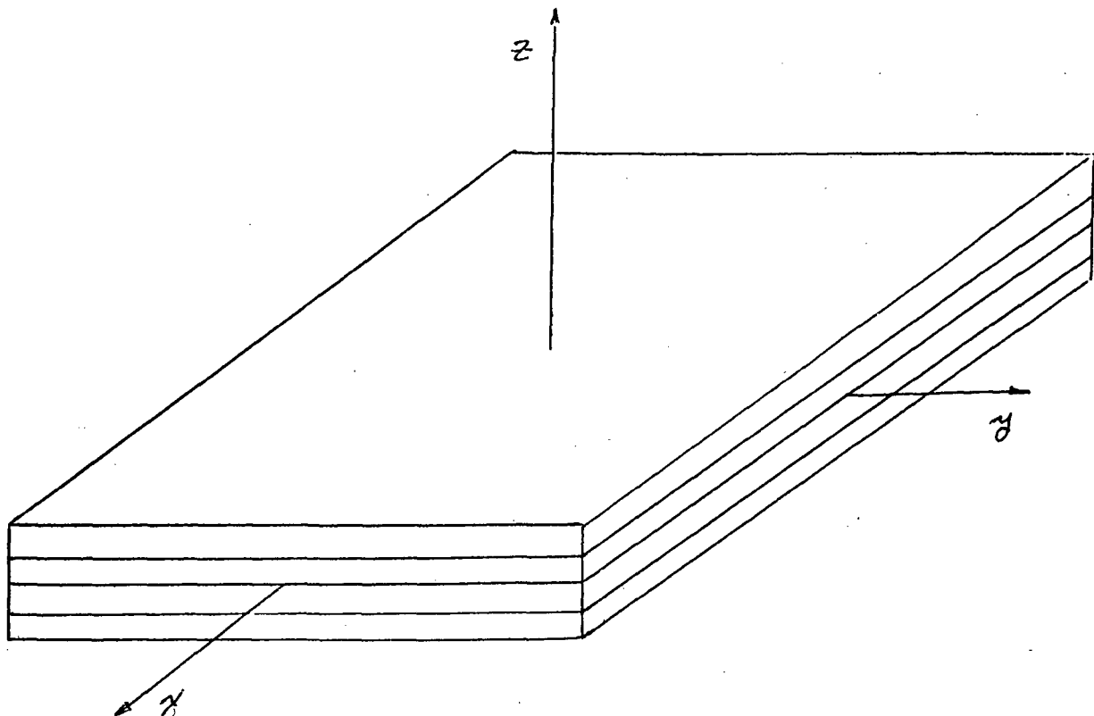
FIGURE 1: GEOMETRY FOR INTERLAMINAR SHEAR PROBLEM
