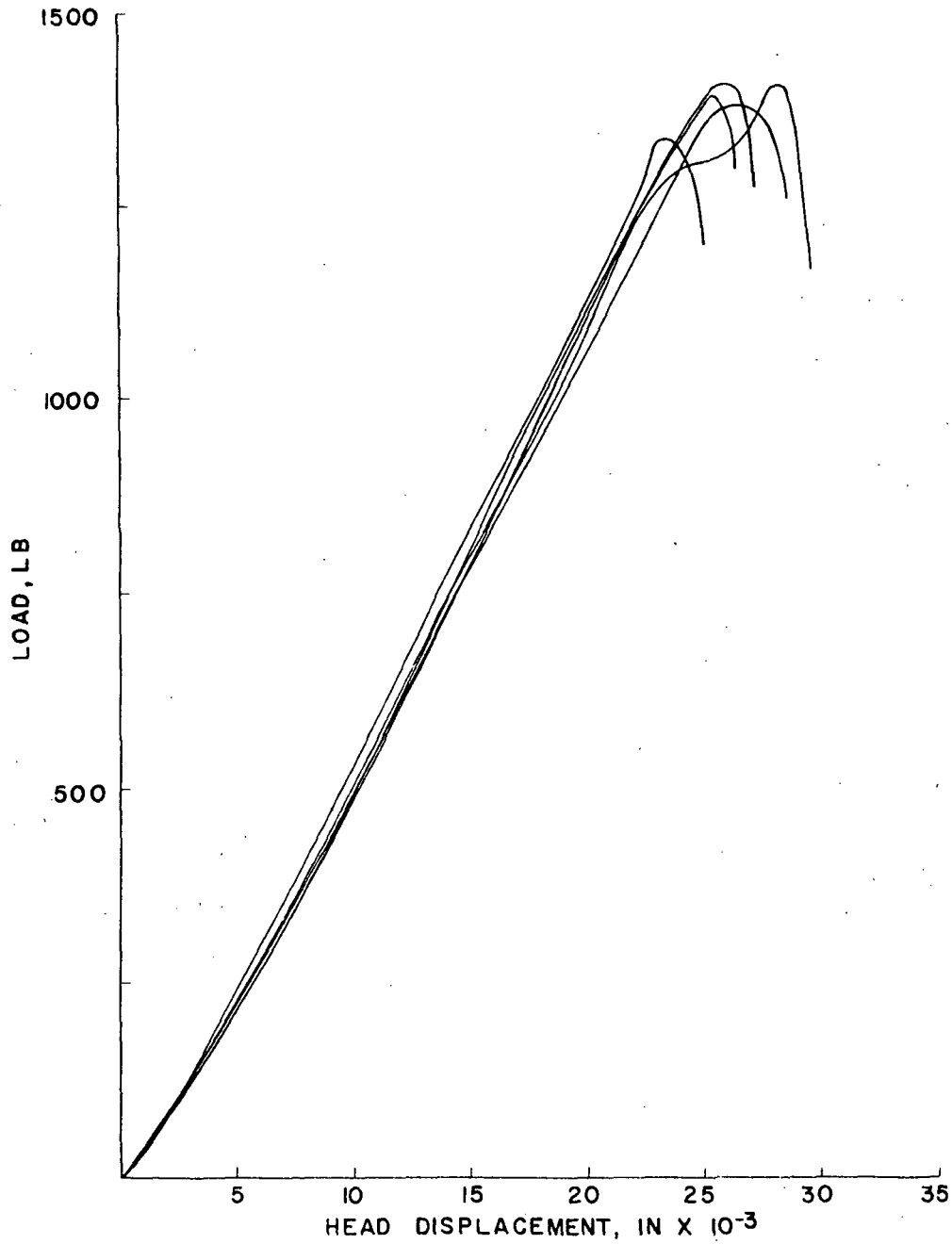
Figure 11: Traces of load vs. cross-head displacement for five specimens used in reproducibility tests for a multi-directional laminate ( \alpha = (0^\circ/\pm 45^\circ/90^\circ)_s , a = 0.4 in).
