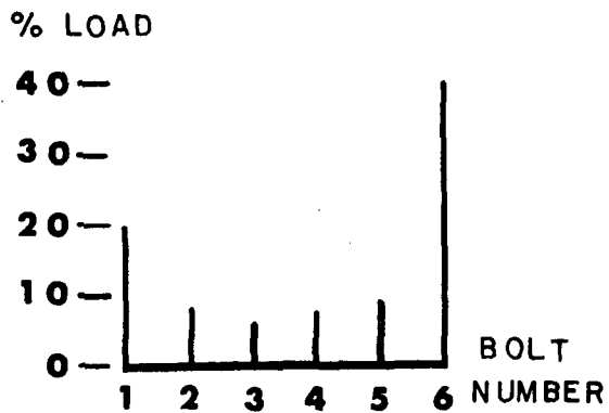
(a) Specimen 1
