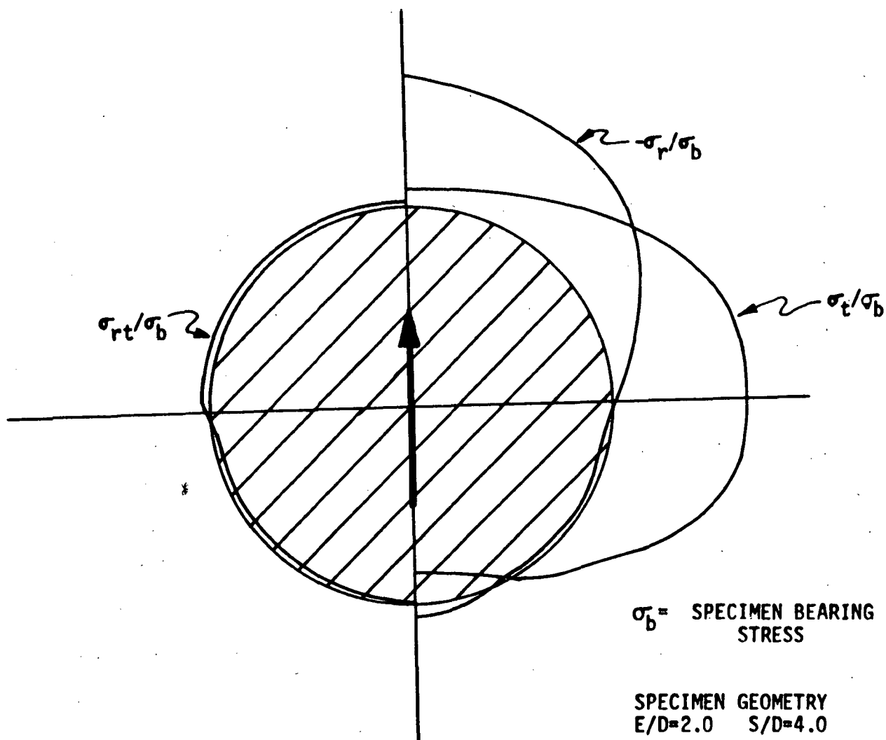
FIGURE 4; POLAR PLOT OF EDGE STRESSES FOR AN ISOTROPIC TEST RUN
