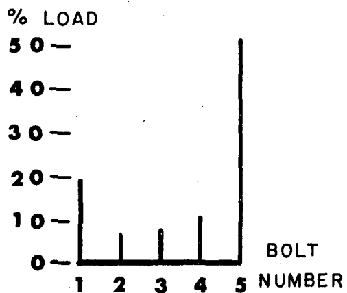
(c) Specimen 3
