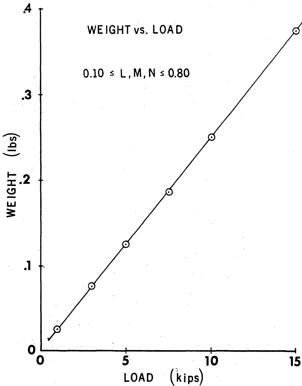
FIGURE 2: WEIGHT VS. LOAD FOR VARIABLE ORIENTATIONS
