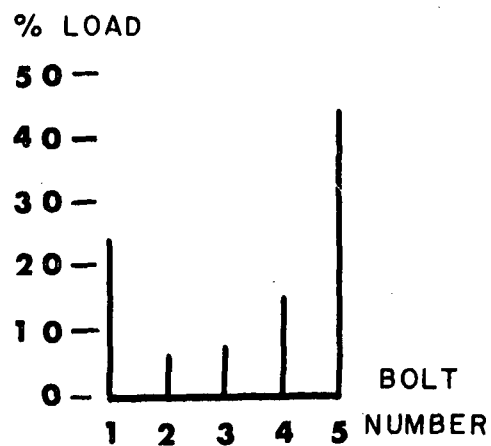
(b) Specimen 2
