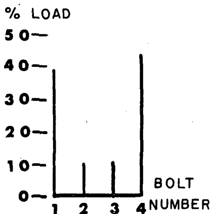
(e) Specimen 5
