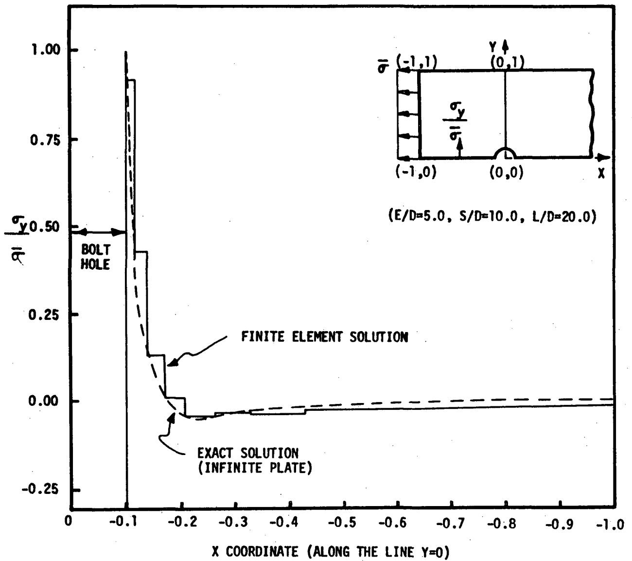
FIGURE 3b: ISOTROPIC BOLT BEARING VERIFICATION: \sigma_y/\sigma_0 vs X
