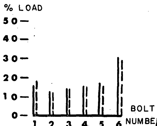
(f) Specimen 6
