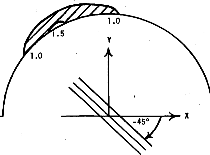
FIGURE 7b: NET TENSION FAILURE -45° LAMINA
