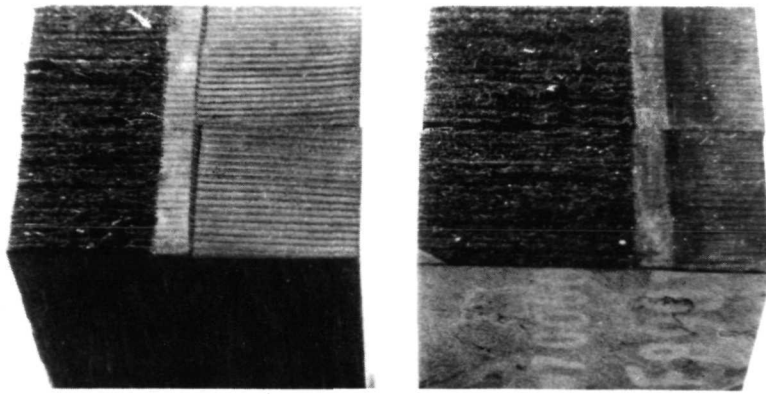
Figure 8: Failure surfaces for \alpha = (0^\circ/\pm 45^\circ/90^\circ)_s specimens of two starter crack lengths ( a = 0.6, 0.4 in).
