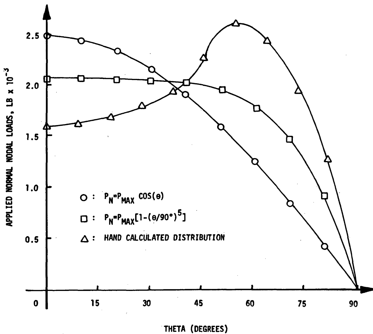
FIGURE 5: VARIATIONS ABOUT THE COSINE DISTRIBUTION OF NORMAL STRESS
