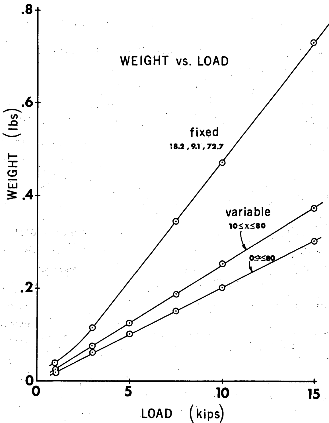
FIGURE 3: SUMMARY OF WEIGHT VS. LOAD RESULTS
