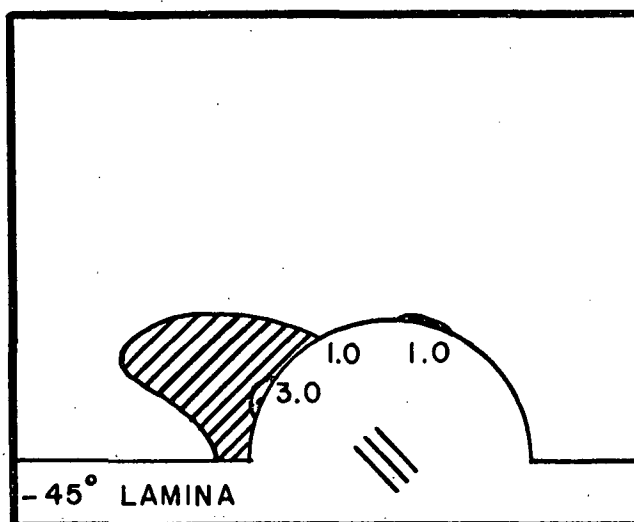
Figure 9. Specimen 3: Distortional Energy Contour Plots for the Experimental Failure Load.
