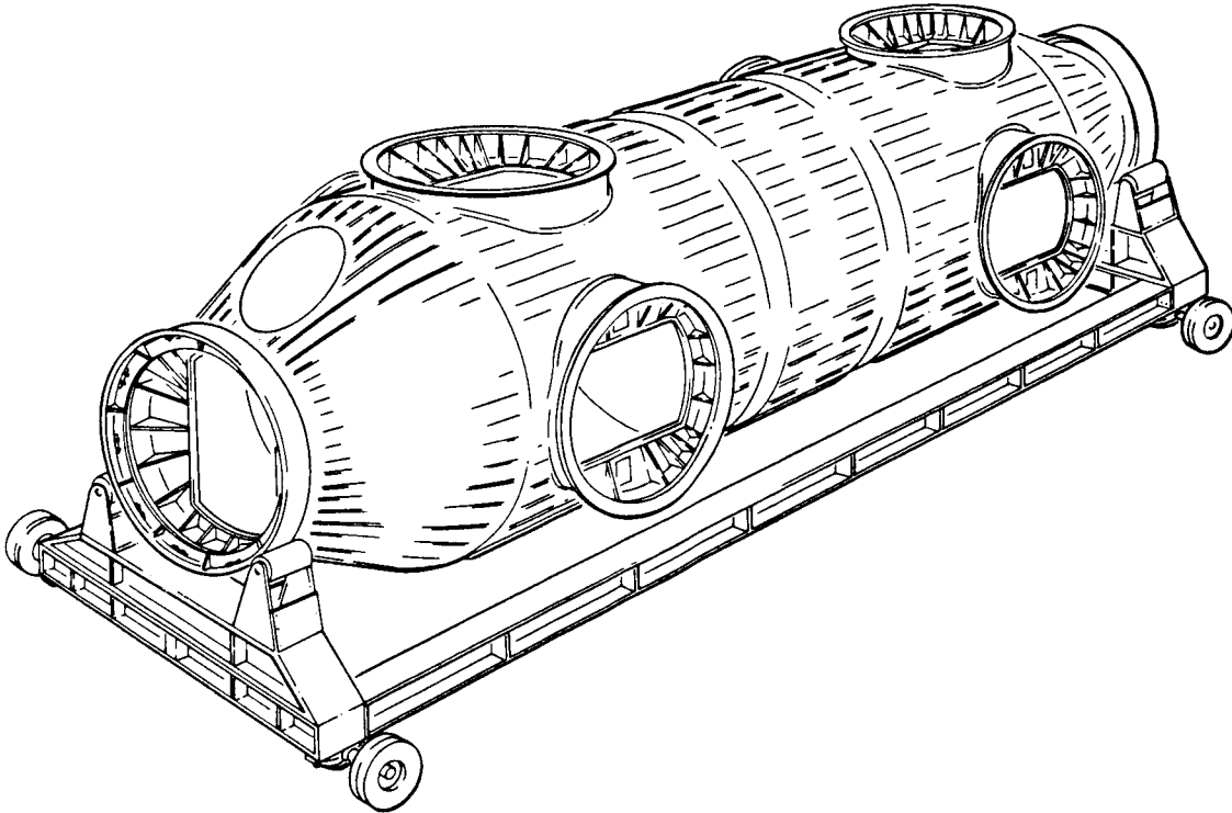
Figure 4-3. Rotational Transporter
