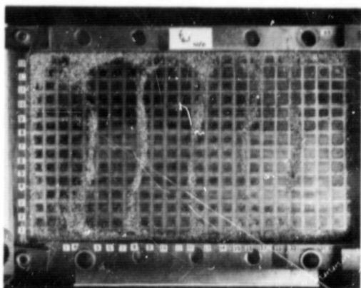
Mode (6,1)
