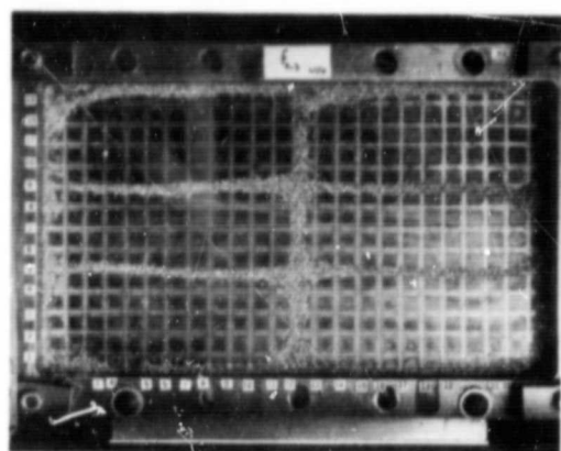
Mode (2,3)
