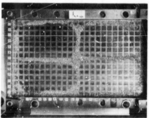
Mode (2,2)
