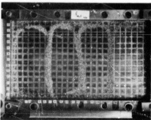
Mode (4,1)
