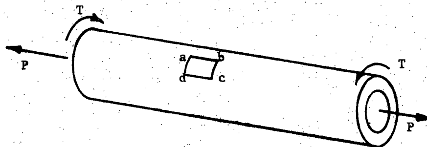
(a) Combined Loading System - Tubular Specimen
