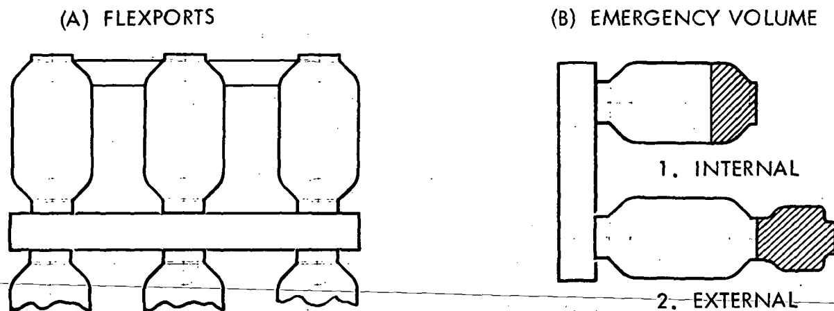
Figure 4.2-2. Alternative Solutions for Dual Egress
