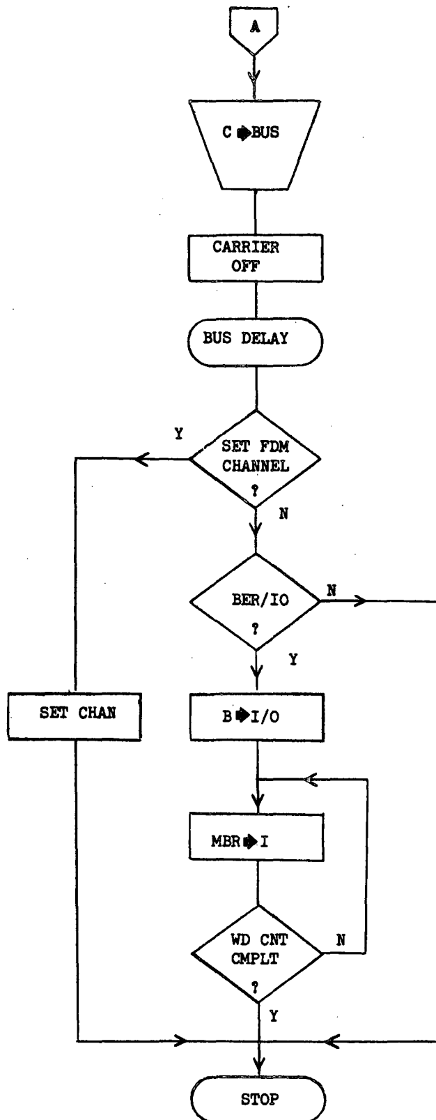
Figure 3-33. Data Bus Terminal Flow Diagram (page 3 of 3)
