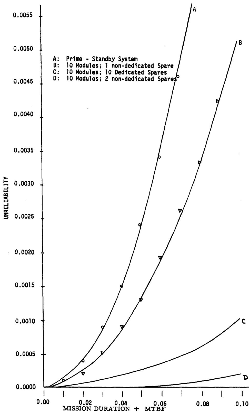
Figure 9-1. Computer System Unreliability
