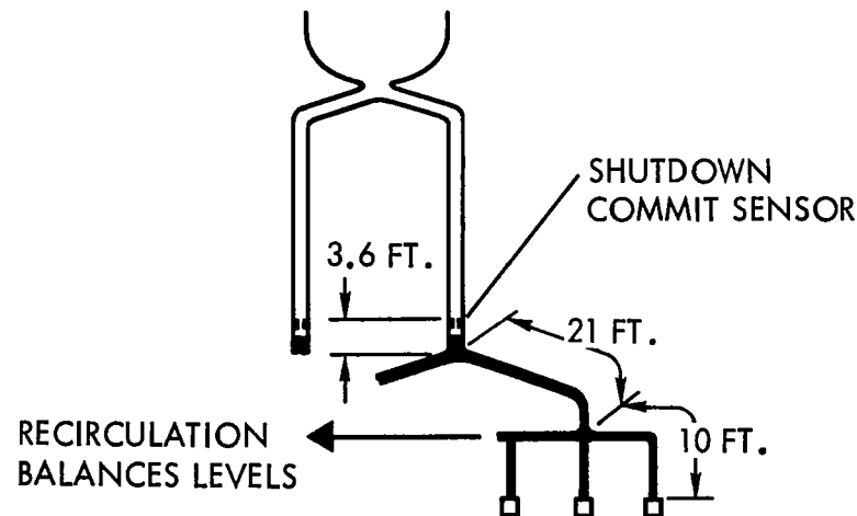
TWO-PHASE LAYER ELIMINATED T \cong 9 \text{ SEC.}
