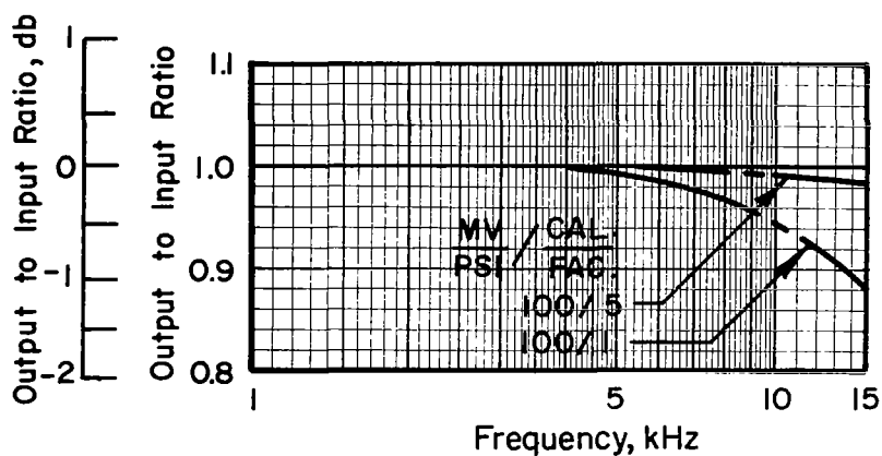
b. Test Transducer Charge Amplifier
