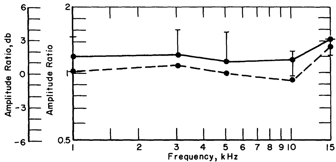
FIGURE 9. AMPLITUDE RATIO VS FREQUENCY FOR KISTLER MODEL 616 SERIAL NO.1692 STATIC-PRESSURE LEVEL, 150 psia ( 104 \frac{\text{N}}{\text{cm}^2} abs)
