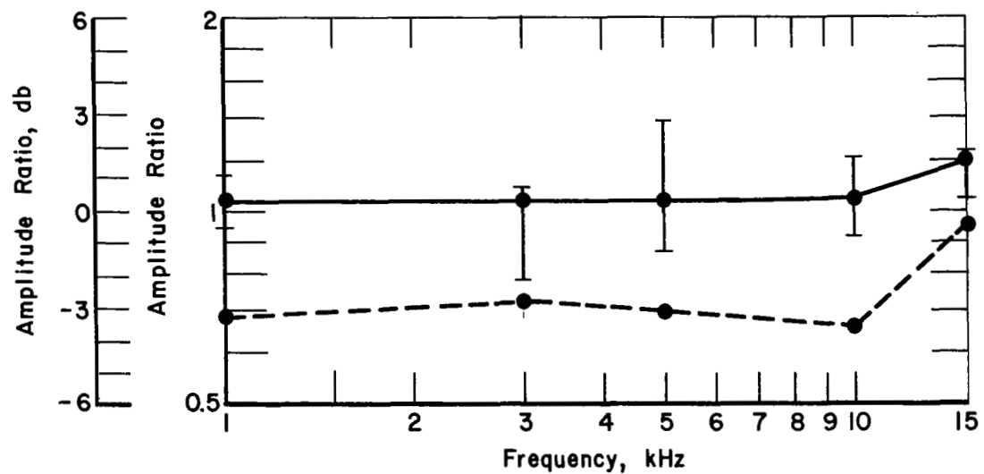
FIGURE II. AMPLITUDE RATIO VS FREQUENCY FOR SENSOTEC MODEL SA8J-6H, SERIAL NO. 5563; STATIC -PRESSURE LEVEL 45 psia \left(31 \frac{\text{N}}{\text{cm}^2} \text{ abs}\right)
