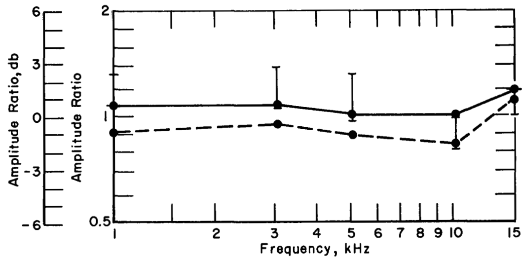
FIGURE 10. AMPLITUDE RATIO VS FREQUENCY FOR PCB MODEL 122 MO3 SERIAL NO. 108. STATIC-PRESSURE LEVEL, 150 psia ( 104 \frac{\text{N}}{\text{cm}^2} abs)
