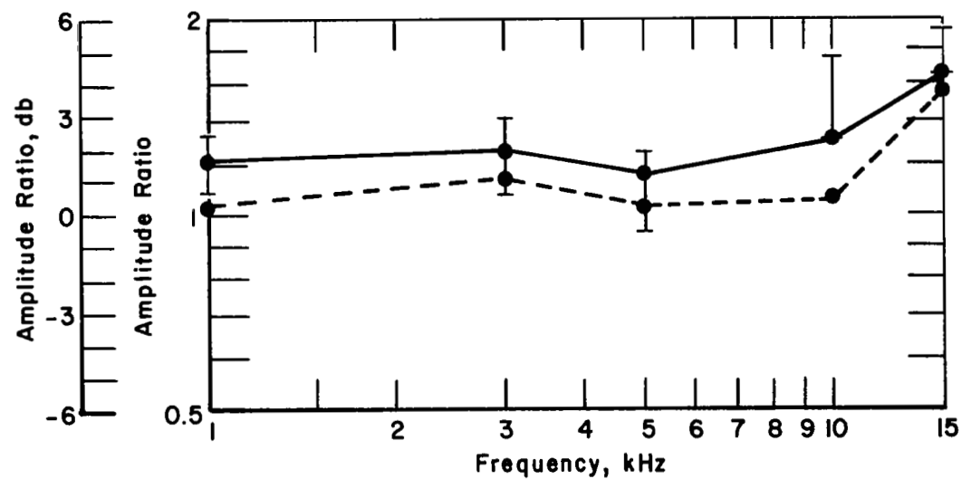
FIGURE 8. AMPLITUDE RATIO VS FREQUENCY FOR KISTLER MODEL 614A, SERIAL NO. 348; STATIC-PRESSURE LEVEL, 150 psia ( 104 \frac{\text{N}}{\text{cm}^2} \text{ abs} )
