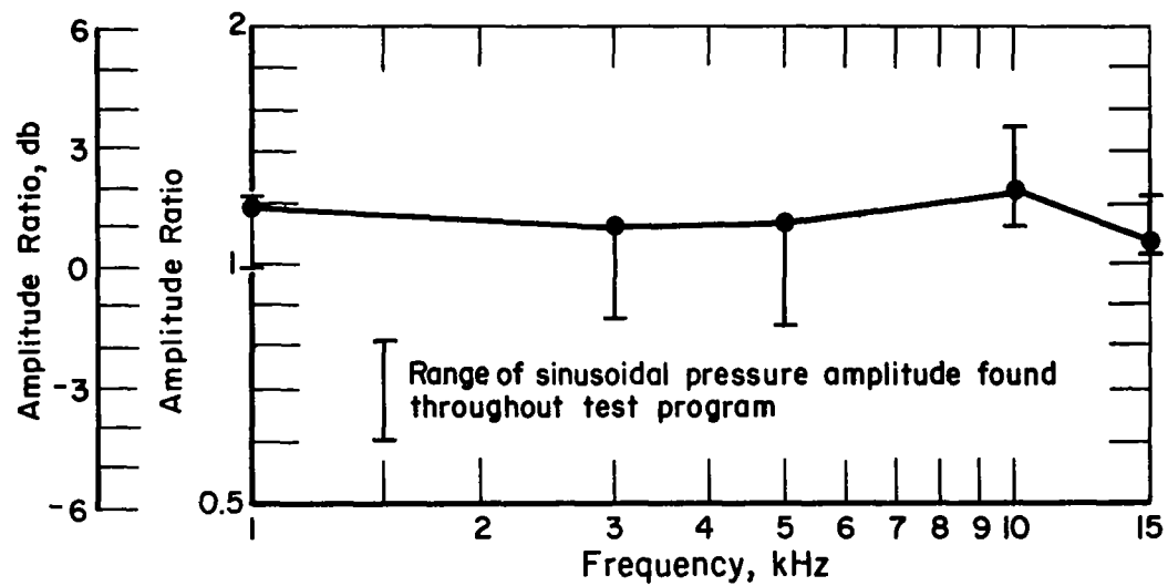
FIGURE 6. AMPLITUDE RATIO VS FREQUENCY FOR KISTLER MODEL 603A SERIAL NO. 2275. STATIC - PRESSURE LEVEL, 150 psia ( 104 \frac{\text{N}}{\text{cm}^2} abs)
