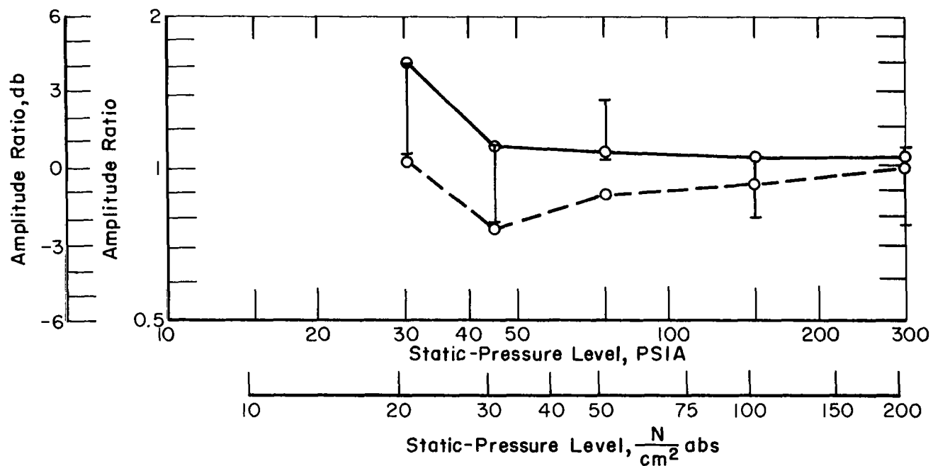
FIGURE I5. AMPLITUDE RATIO VS STATIC-PRESSURE LEVEL FOR KISTLER MODEL 603 A SERIAL NO. 2275 SILASTIC DIAPHRAM, 0.025 INCH (0.064 cm); FREQUENCY, 3 kHz
