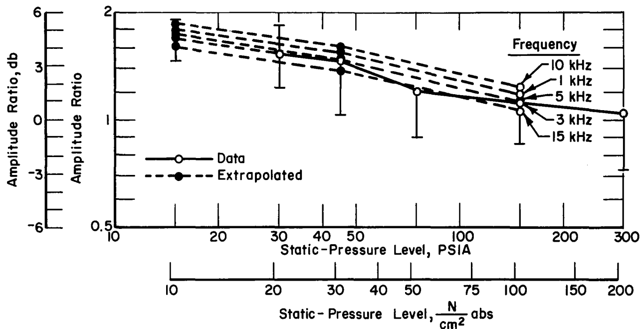
FIGURE I4. AMPLITUDE RATIO VS STATIC-PRESSURE LEVEL AT VARIOUS FREQUENCIES FOR KISTLER MODEL 603A SERIAL NO. 2275. INCLUDES EXTRAPOLATED CONDITIONS USED TO RATIO TEST TRANSDUCER TO TEST TRANSDUCER SIDE OF SINUSOIDAL PRESSURE GENERATOR
