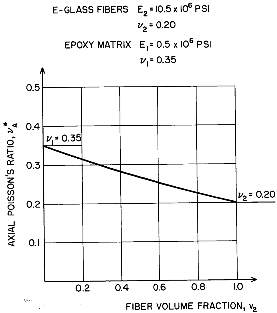
FIG. 3.5.4 - AXIAL POISSON'S RATIO, \nu_A^* , CCA MODEL
