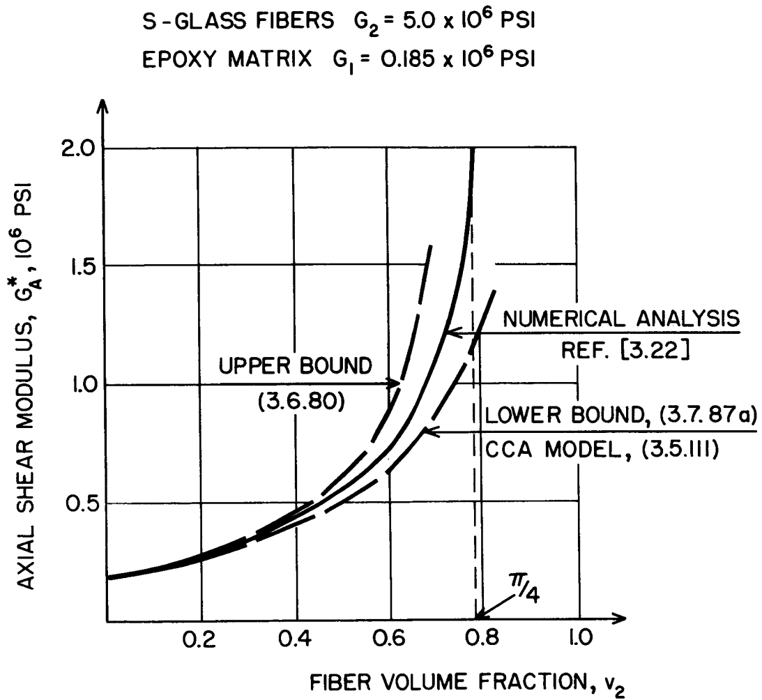
FIG. 3.7.5 - BOUNDS FOR AXIAL SHEAR MODULUS G_A^* OF SQUARE ARRAY OF CIRCULAR FIBERS
