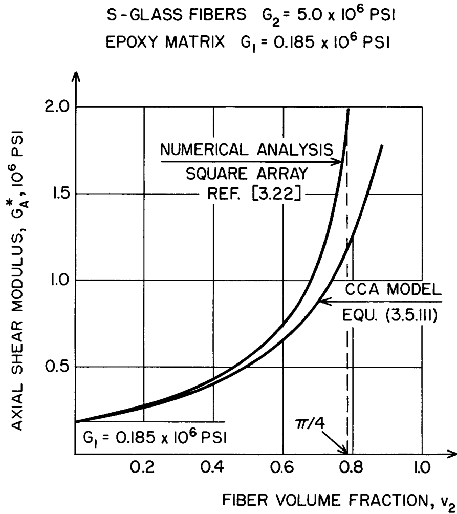
FIG. 3.5.11 - COMPARISON OF SQUARE ARRAY AND CCA MODEL RESULTS: AXIAL SHEAR MODULUS G_A^*
