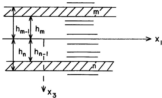
FIG. 3.10.4 - SYMMETRIC LAMINAE PAIR
