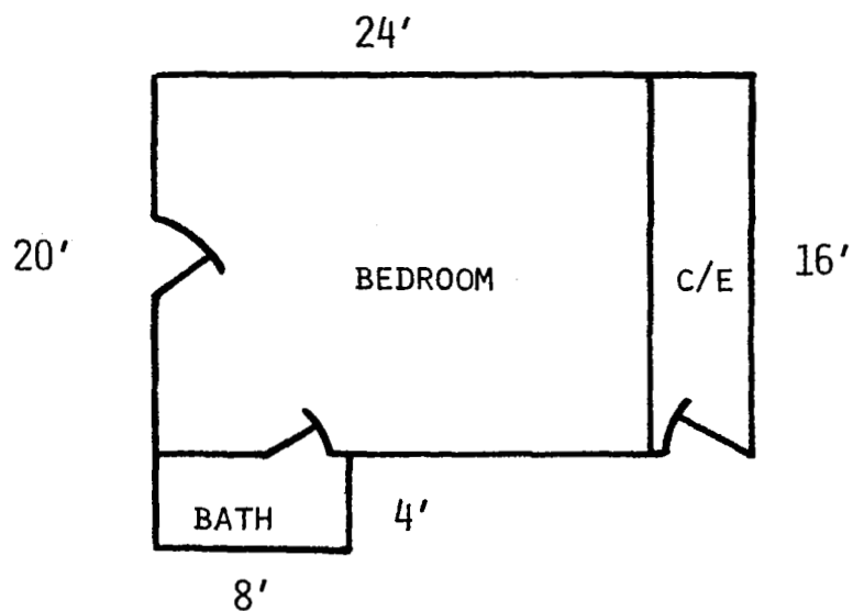
TOP PROFILE
