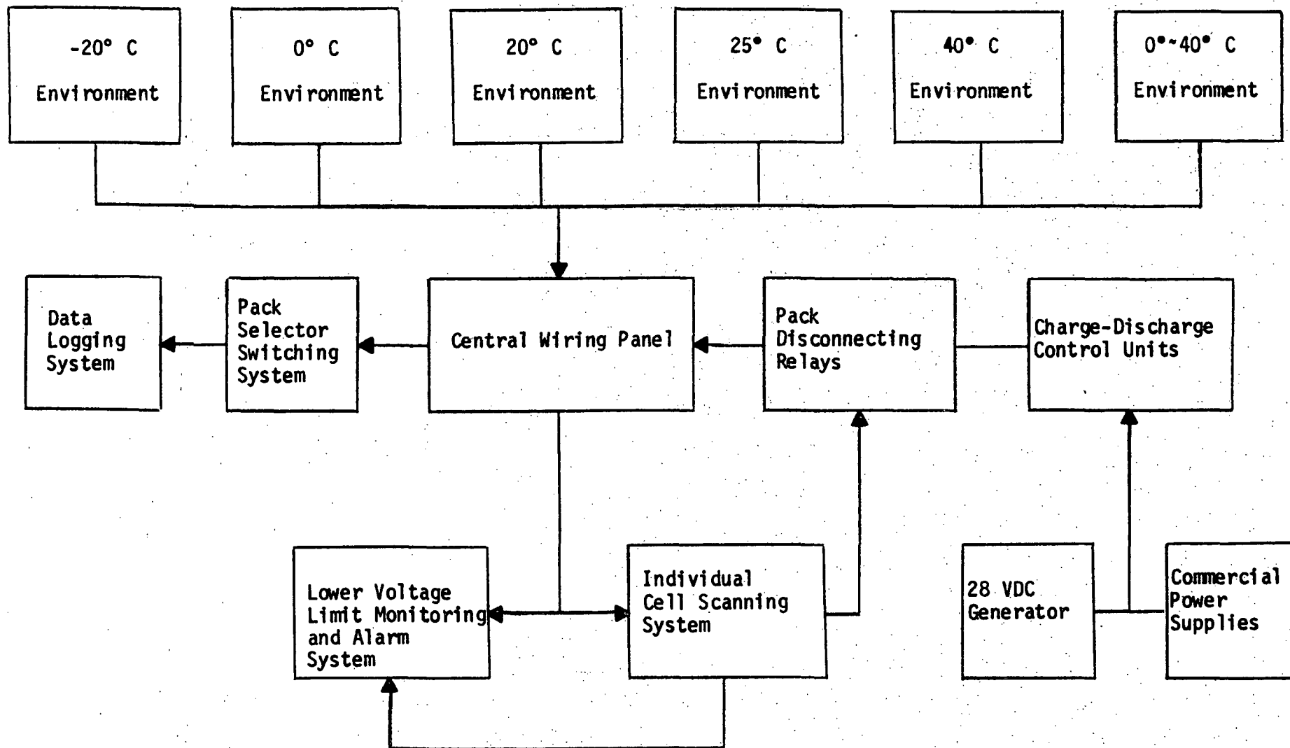
BLOCK DIAGRAM OF TEST SETUP
